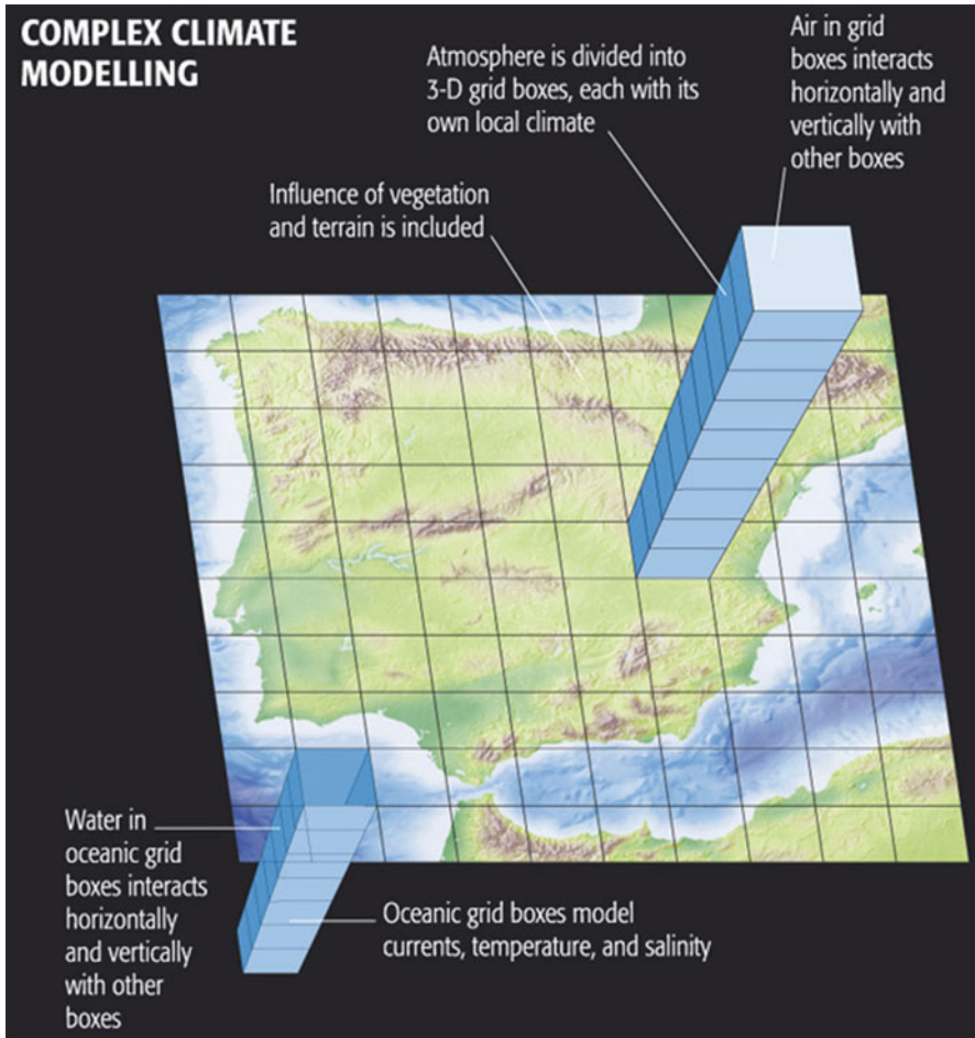
Fig. 18.5 A climate model showing the horizontal and vertical grids and the physical processes in a global circulation model (GCM) (From Mann and Kump, Dirge Predictions , supported by the National Science Foundation, Public Domain)
