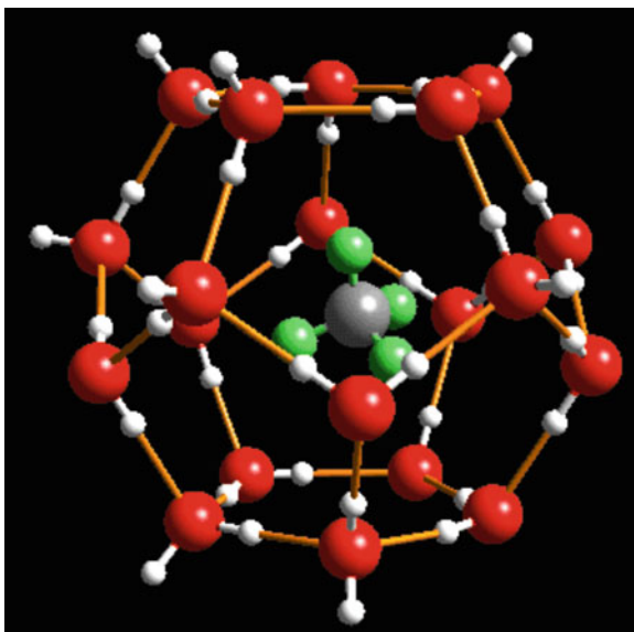
Fig. 5.10 A model of a methane clathrate showing the cage of \text{H}_2\text{O} molecules trapping a methane molecule (From http://peggy.uni-mki.gwdg.de/docs/kuhs/clathrate_hydrates.html ; No source information given on web site. Permission granted by Dr. Werner Kuhs from which the figure is taken)
