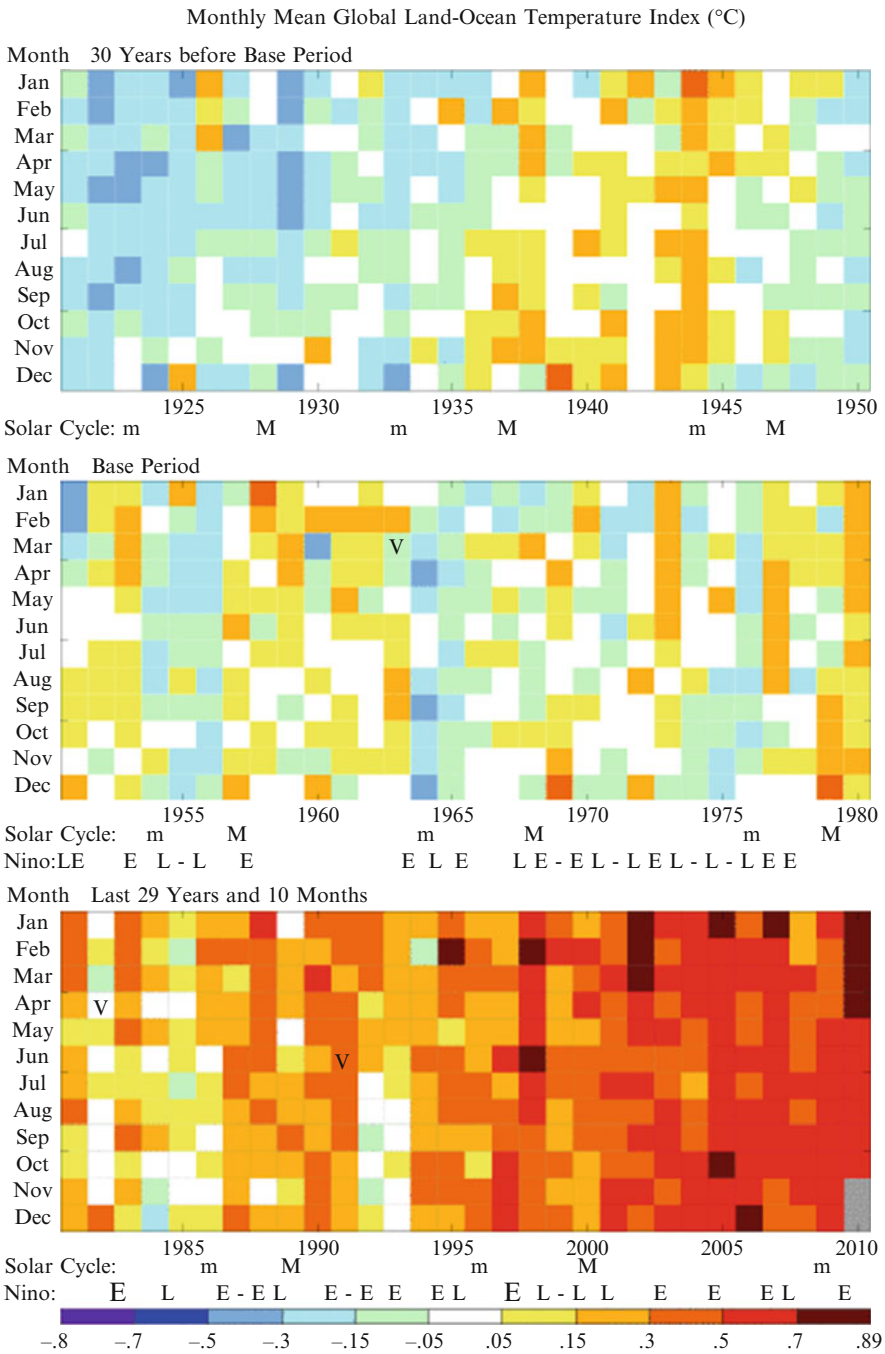
Fig. 6.9 Monthly mean global land-ocean temperature index (°C); (Top Panel) 30 years prior to the Base Period. (Middle Panel) The Base Period. (Bottom Panel) Past 30 years (1980–2010) (NASA/GISS, Public Domain)
