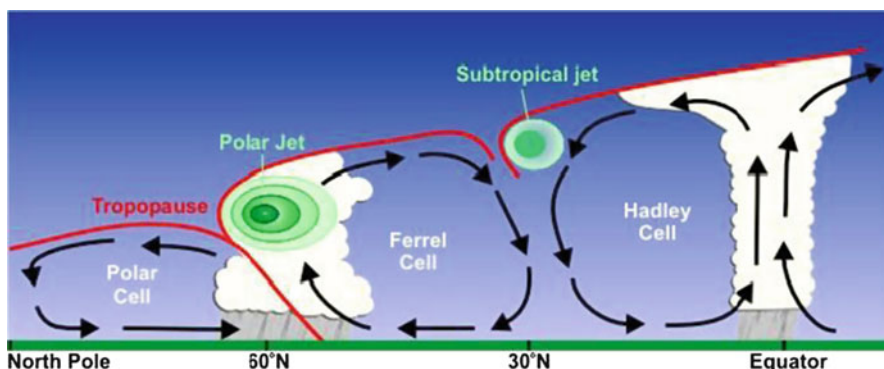
Fig. 8.4 The tropopause varies in elevation within the atmosphere being higher at the Equator and lower at the poles (NOAA, Public Domain)
