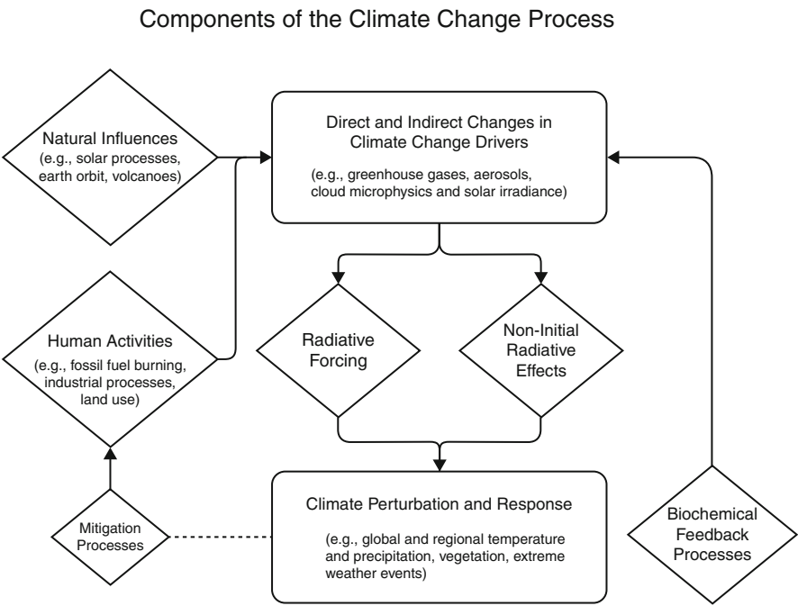
Fig. 5.15 Components of the climate change process (Redrawn from IPCC, AR4, 2007 by John Cook)
