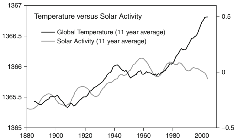
Fig. 5.12 Global temperature ( dark line , NASA GISS) and Total solar irradiance ( lighter line , 1880–1978 from Solanki; 1979–2009 from Physikalisch-Meteorologisches Observatorium Davos (PMOD). (From SkepticalScience.com, redrawn by John Cook)
