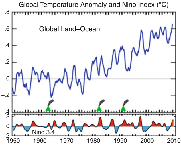
Fig. 6.3 Blue curve: 12-month running-mean global temperature. Note correlation with Niño index (red=El Niño, blue=La Niña). Large volcanoes (green) have a cooling effect for ~2 years (NASA/GISS, Public Domain)
