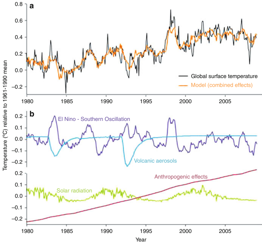
Fig. 7.1 (a) Observed monthly mean global temperatures ( black ) and an empirical model ( orange ) that combines four different influences. (b) Individual contributions of these influences, namely ENSO ( purple ), volcanic aerosols ( blue ), solar irradiance ( green ) and anthropogenic effects ( red ). Together the four influences explain 76% ( r^2 ) of the variance in the global temperature observations (Adapted from Lean and Rind 2009)
