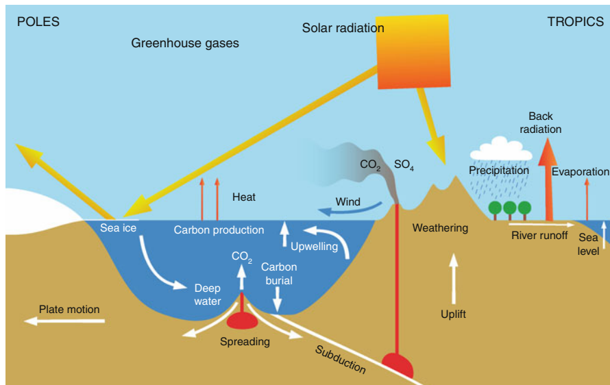
Fig. 5.17 The major components of the climate system. \text{H}_2\text{O}_v is water vapor (Source: John Cook Redrawn from Ruddiman 2001)
