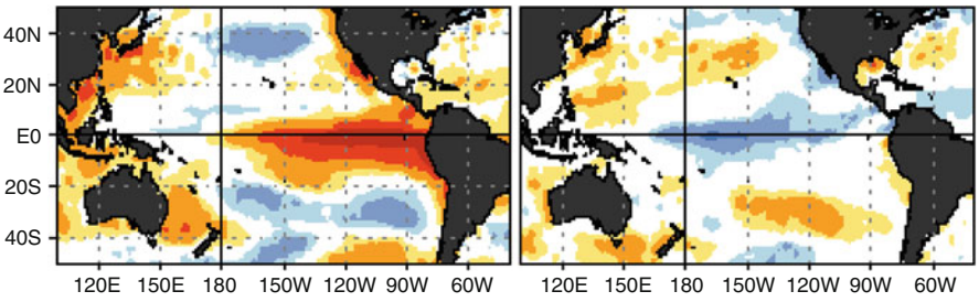
Fig. 13.7 El Niño ( left panel ) and La Niña ( right panel ) sea surface temperatures (From http://www.cpc.ncep.noaa.gov/products/analysis_monitoring/ensocycle/enso_cycle.shtml , Public Domain)
