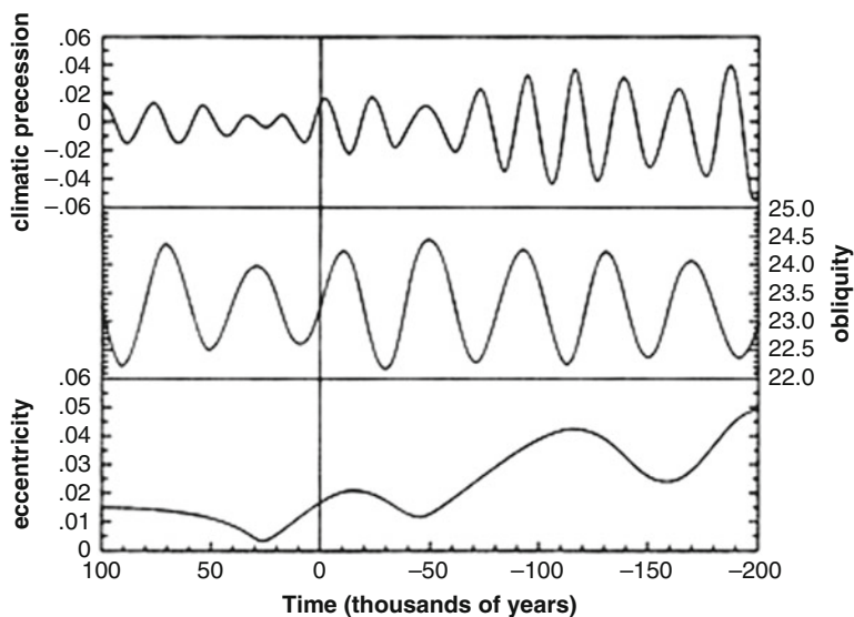
Fig. 14.23 Milankovitch calculated solar energy receipt during summer at 65°N for the past 600,000 years (also for 55° and 60°, but they are not shown in the above graph). The above graphs show calculated values for 300,000 years of orbital variation. The line labeled “0” represents today, while “-200” indicates 200,000 years in the past and “100” indicates 100,000 years from now. Milankovitch noticed that these cycles of orbital mechanics correspond to many indicators of past climate change, such as Ice Ages (From NASA, Public Domain; originally from Berger and Loutre 1991)
