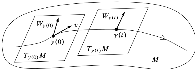
Fig. 9.12 The problem with directional derivatives of vector fields
