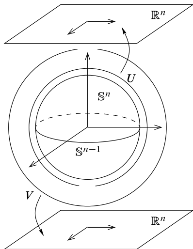
Fig. 17.2 Computing the de Rham cohomology of S^n
