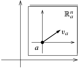
Fig. 3.1 Geometric tangent space
