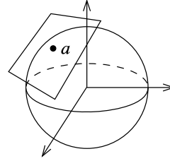
Fig. 3.2 Tangent space to \mathbb{S}^{n-1}
