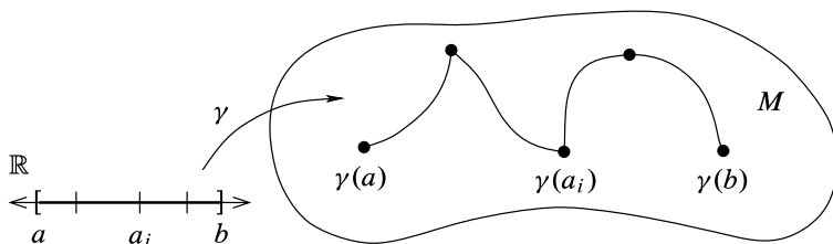
Fig. 11.4 A piecewise smooth curve segment
