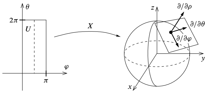
Fig. 15.7 Parametrizing the sphere via spherical coordinates
