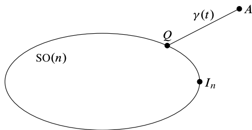
Fig. 21.2 Proof that \text{GL}^+(n, \mathbb{R}) is connected
