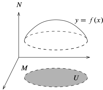
Fig. 5.1 A graph is an embedded submanifold
