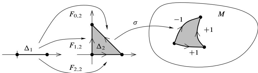
Fig. 18.2 The singular boundary operator
