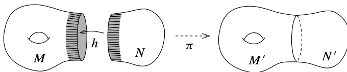
Fig. 9.10 Attaching manifolds along their boundaries
