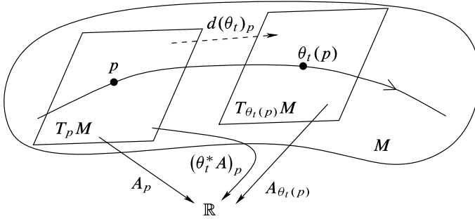
Fig. 12.1 The Lie derivative of a tensor field
