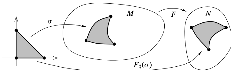
Fig. 18.3 The homology homomorphism induced by a continuous map
