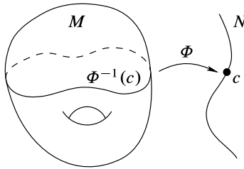
Fig. 5.4 A level set
