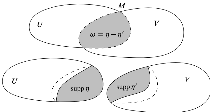
Fig. 17.4 Surjectivity of i^* - j^*
