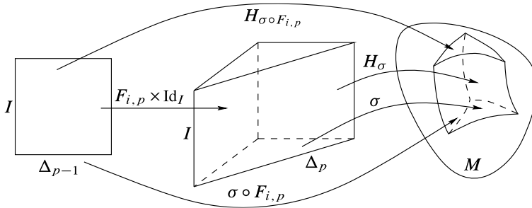
Fig. 18.4 The homotopy H_\sigma
