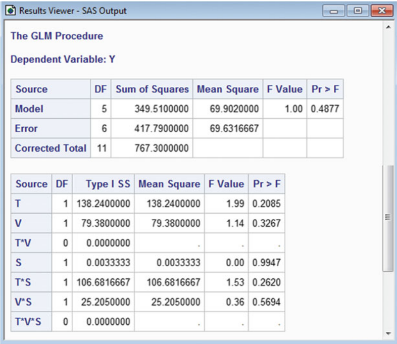
Fig. 7.8 Output from the first call of PROC GLM for the rail weld experiment
