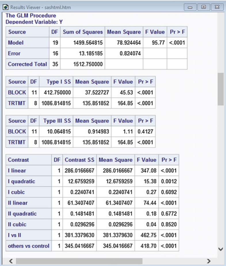
Fig. 11.6 Partial output from PROC GLM for analysis of an incomplete block design—detergent experiment
