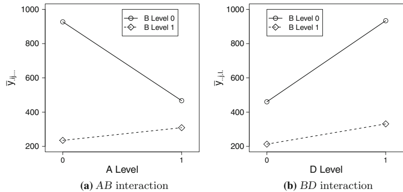
Fig. 13.5 Interaction plots for the decontamination alpha-particle experiment
