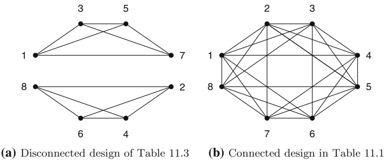
Fig. 11.1 Connectivity graphs to check connectedness of designs
