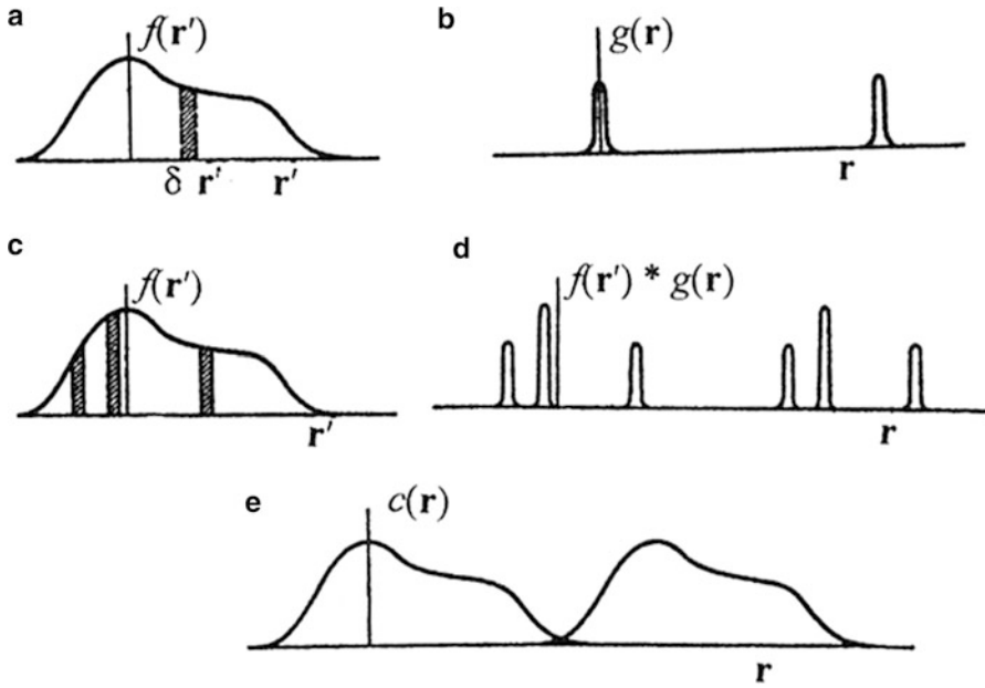
Fig. 6.18 Convolution of two functions in the one-dimension space of \mathbf{r} . (a) Function f(\mathbf{r}') , showing an element of width \delta \mathbf{r}' . (b) Function g(\mathbf{r}) , showing two sharp peaks. (c) Function f(\mathbf{r}') with three selected elements \delta \mathbf{r}' . (d) Convolution of (b) and (c); the three elements are reproduced by g(\mathbf{r}) , modified by the values of that function. (e) The completed convolution f(\mathbf{r}') * g(\mathbf{r}) ; because the function g(\mathbf{r}) does not have infinitesimal width, f(\mathbf{r}') is reproduced in a slightly modified form (6.14)
