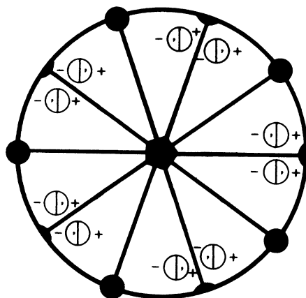
Fig. 1.35 Stereogram of the non-crystallographic point group \overline{10}m2 ( D_{5h} ) showing the general form (20 poles), and a special form of 5 poles lying on the m planes that can be used to represent the five F atoms in one plane in \text{UF}_7 . The poles for the remaining two F atoms lie at these center of the stereogram, on the \overline{10} axis
