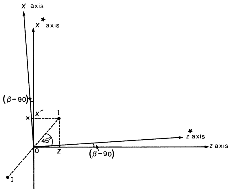
Fig. 6.16 Geometry of the reconstruction of the x and z coordinates of the iodine atoms in euphenyl iodoacetate. The \beta angle is 94.1^\circ ; X , X' , and Z are measured along the x , x^* , and z axes, respectively. Note that since the space group of euphenyl iodoacetate is P2_1 , the y coordinates of the iodine atoms may be set at \pm \frac{1}{4} , so as to fix the position of the origin with respect to the symmetry elements
