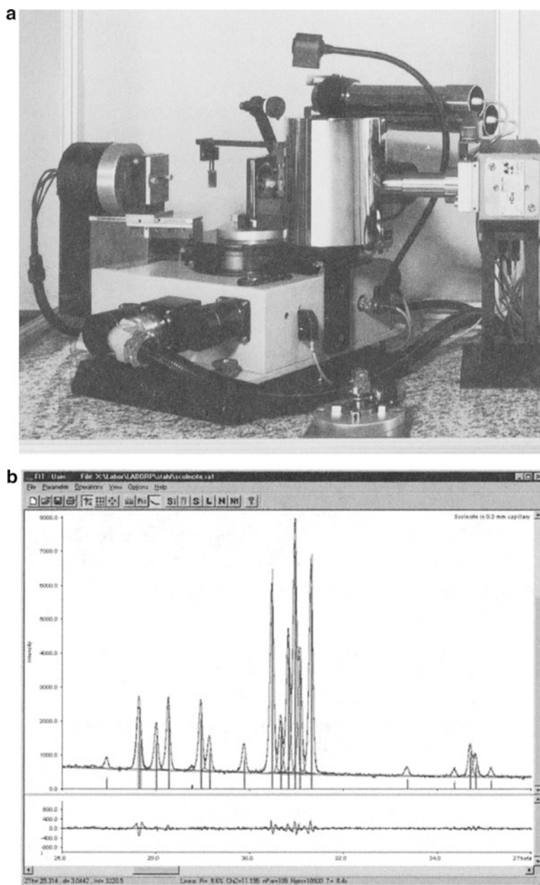
Fig. 12.8 (a) The Stoe STADI P powder diffractometer system: the radiation is K\alpha_1 , in the range available from Fe to Mo targets; the focusing circle diameter is 130 mm, the 2\theta range is 0 – 140^\circ , and the minimum step size is 0.0005^\circ . Intensities are measured by a scintillation counter, and the whole operation is handled by built-in structure-solving software. (b) A diffractogram of solecite, a calcium-containing zeolite, measured in the Debye–Scherrer transmission mode in a capillary of 0.3 mm diameter: calculated and experimental peaks (with probable errors indicated), positions of main peaks (vertical lines) and, below, the difference curve are shown (courtesy Stoe & Cie GmbH, Darmstadt, Germany)
