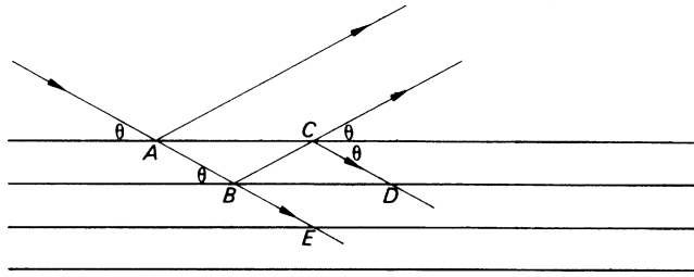
Fig. 4.3 Primary extinction: the phase changes by reflection at B and C are each \pi/2 , so that between the directions BE and CD , the total phase change is \pi . Thus, there is an attenuation of the incident X-ray beam reaching planes deeper into the crystal
