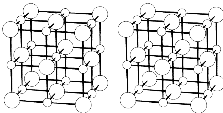
Fig. 1.6 Stereoview of the face-centered cubic unit cell and its environs for the crystal structure of sodium chloride:
