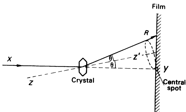
Fig. 5.14 Geometry of the Laue method: XY, X-ray beam direction; ZZ', a zone axis; R, generator of the cone of diffracted rays of semi-angle \theta , the Bragg angle; Y, central spot on the film and extremity of the major axis of the ellipse formed by the intersection of the cone with the film
