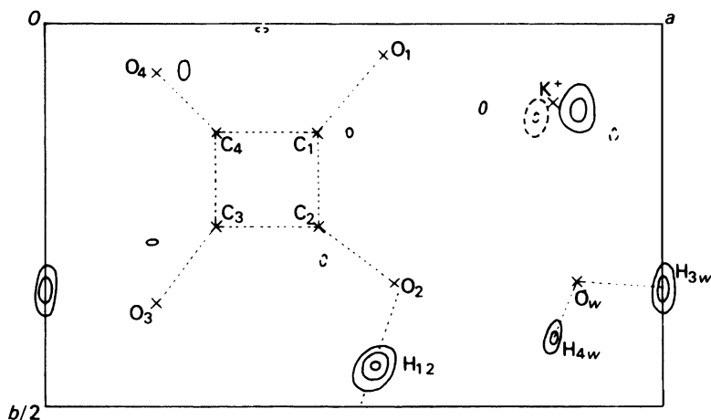
Fig. 9.27 Composite difference electron density map for KHSQ. Positive contours are solid lines and negative contours are broken lines. Bonds in the squarate ring and those involving hydrogen atoms are shown as dotted lines. Some spurious, small peaks (unlabeled) were shown by this synthesis
