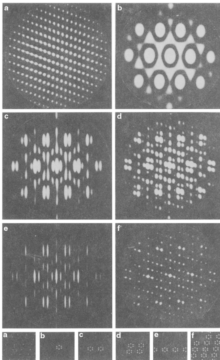
Fig. 6.10 Optical diffraction patterns illustrating scattering. (a) Two-dimensional lattice (portion only). (b) Single molecule (simulated benzene ring). (c) Two such molecules. (d) Four molecules. (e) A row (portion only) of six molecules. (f) A net (portion only) of molecules; this pattern resembles closely an X-ray diffraction photograph (reproduced from Taylor and Lipson 1964)
