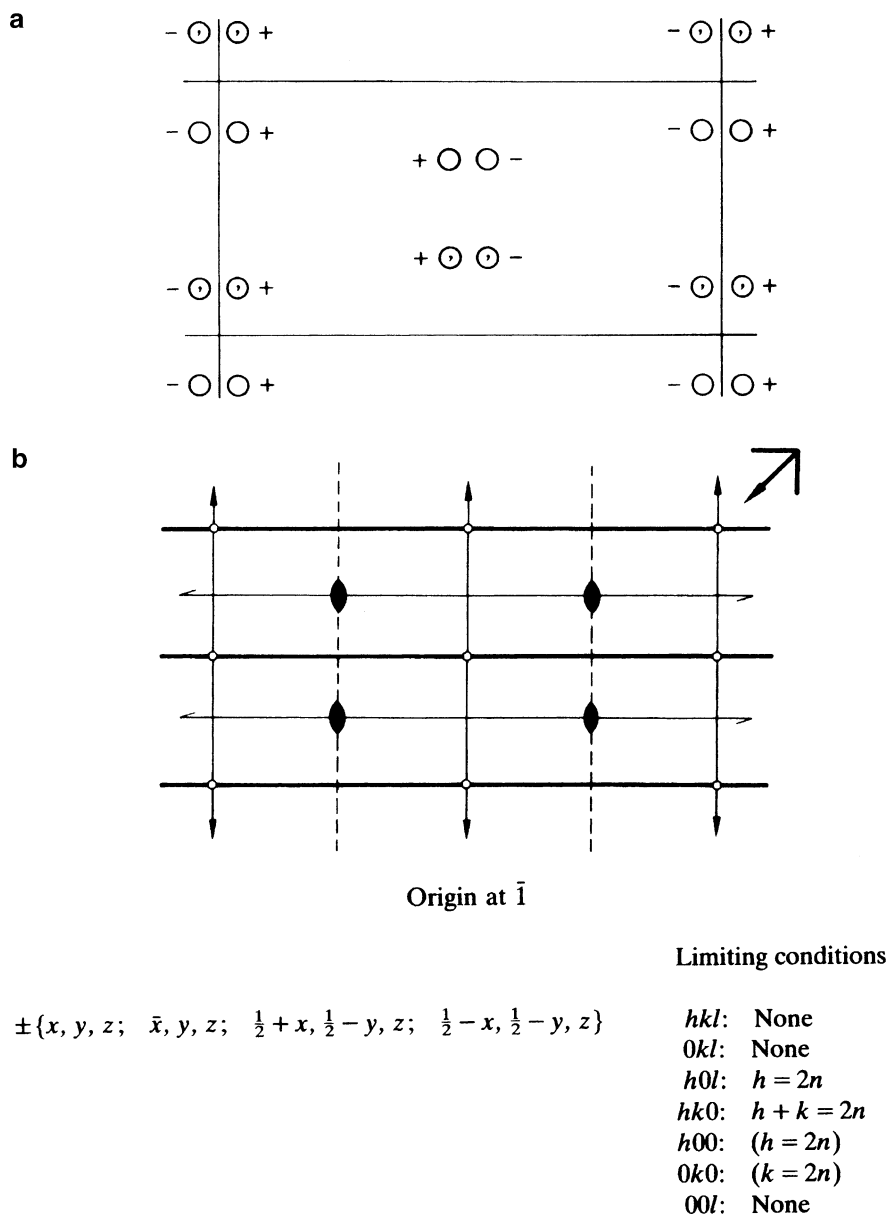
Fig. 3.26 Space group Pman . (a) General equivalent positions. (b) Symmetry elements; the origin is on \bar{1} . The diagram shows also the limiting conditions for this space group.
