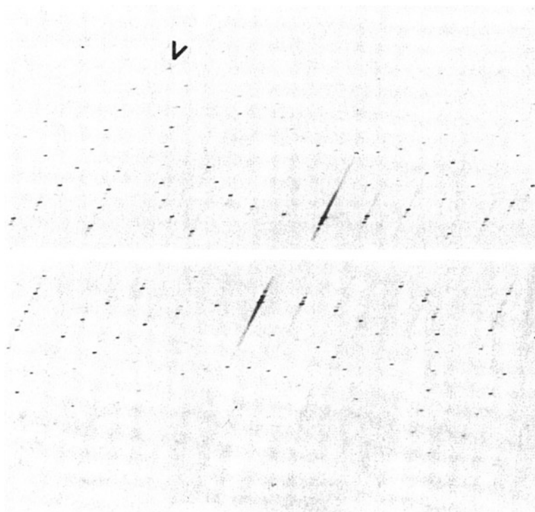
Fig. 9.5 Weissenberg photograph of the h0l layer. The more intense reflections show spots arising from both Cu K\alpha ( \lambda = 1.5418 \text{ \AA} ) and Cu K\beta ( \lambda = 1.392 \text{ \AA} ) radiations. In some areas, spots from W L\alpha radiation ( \lambda = 1.48 \text{ \AA} ) arise due to sputtering of the copper target in the X-ray tube with tungsten from the filament; see Sect. 3.1.1. In each case, the spots for a given h0l reflection lie along the directions of axial rows at decreasing values of \sin \theta , in proportion to the change in \lambda . The continuous streaks (Laue streaks) arise from the “white” radiation; filtering (Chap. 3, Sect. 3.1.4) is never perfect
