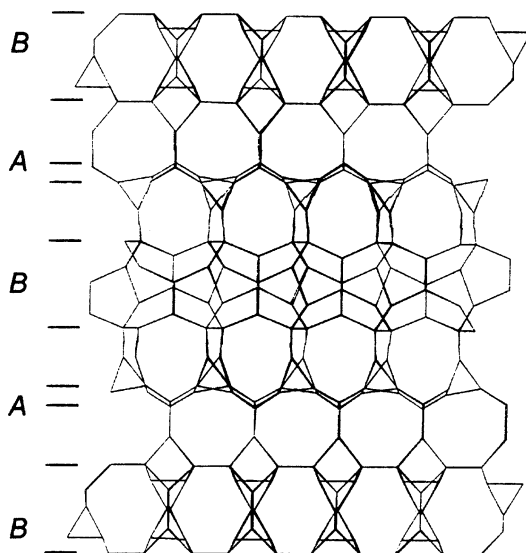
Fig. 12.18 The framework topology of VIP-9 viewed along [110] ; oxygen atoms have been omitted for clarity. Layer B at z = \frac{1}{2} is rotated by 90^\circ with respect to those at z = 0 and 1 . Similarly layer A at z = \frac{3}{4} is rotated by 90^\circ relative to that at z = \frac{1}{4} .
