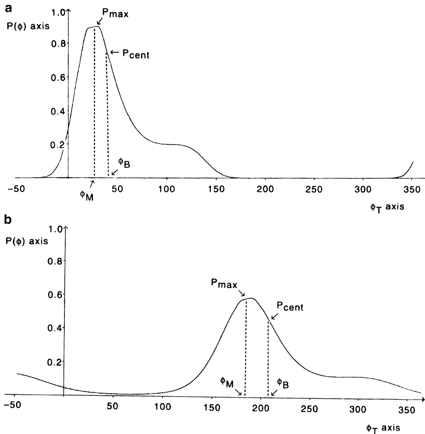
Fig. 7.35 Examples of MIR where the phase circles do not intersect at a point. The most probable value of the phase ( \phi_M at P_{\max} ) and the centroid phase ( \phi_B at P_{\text{cent}} ) are indicated. (a) P(\phi) calculated for the two-derivative case in Fig. 7.34, with \phi_B = 43^\circ , \phi_M = 31^\circ , and m = 0.80 . (b) An example of three-derivative phasing (see Problem 7.14) with \phi_B = 204^\circ , \phi_M = 185^\circ , and m = 0.59 . Although based on three derivatives, the probability distribution in (b) is not as sharp as that in (a), resulting in a lower figure of merit, m , and larger \phi_B \rightarrow \phi_M difference
