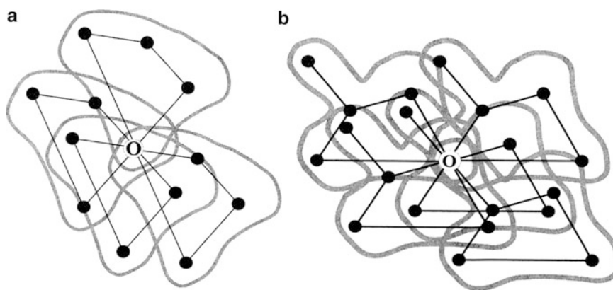
Fig. 8.14 Interatomic vectors for (a) the search model S , and (b) the target molecule T . Only those vectors independent of the Patterson center of symmetry are shown. Both diagrams contain multiple images, or part images, of structures. There is a rotational relationship between the two Patterson functions that the reader should try to determine (see text). Note that the sets of vectors shown here are arranged around the origin of the Patterson function at distances corresponding to the distances between atoms within a given molecule. The high vector density which always occurs at the Patterson origin has been omitted
