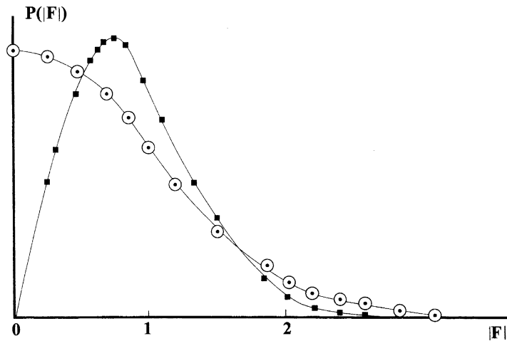
Fig. 4.9 Distribution function for structure amplitudes: (a) acentric, (b) centric. The acentric distribution has a low dispersion of |F| values, whereas the centric distribution has significant proportions of both small and large |F| values
