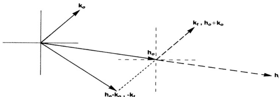
Fig. P9.3 \sum_2 relationships: subscript o refers to the original chart, and subscript t refers to the transparency. If the origin of the transparency is placed over a chosen h_o , it may be seen that coincidences of |E| values given by +k_t , h_o + k_o or by -k_t , h_o - k_o will represent \sum_2 triplets. It should be noted that this technique applies only to centrosymmetric projections of space groups
