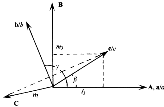
Fig. C.1 \mathbf{A} , \mathbf{B} and \mathbf{C} are unit vectors on Cartesian (orthogonal) axes X , Y , Z , and \mathbf{a}/a , \mathbf{b}/b , and \mathbf{c}/c are unit vectors on the conventional crystallographic axes x , y , z
