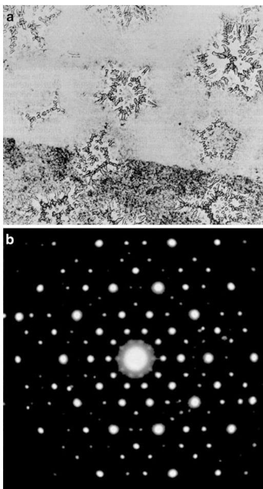
Fig. 1.36 Transmission electron microscopy (TEM) on an \text{Al}_6\text{Mn} alloy. (a) Surface of the \text{Al}_6\text{Mn} alloy, with irregularities inviting further examination. (b) Copy of Original TEM photograph of the alloy surface taken by Professor Shechtman, showing a tenfold spot pattern indicative of a crystalline nature, but without the periodicity of classical crystals (reproduced by courtesy of Professor Shechtman)
