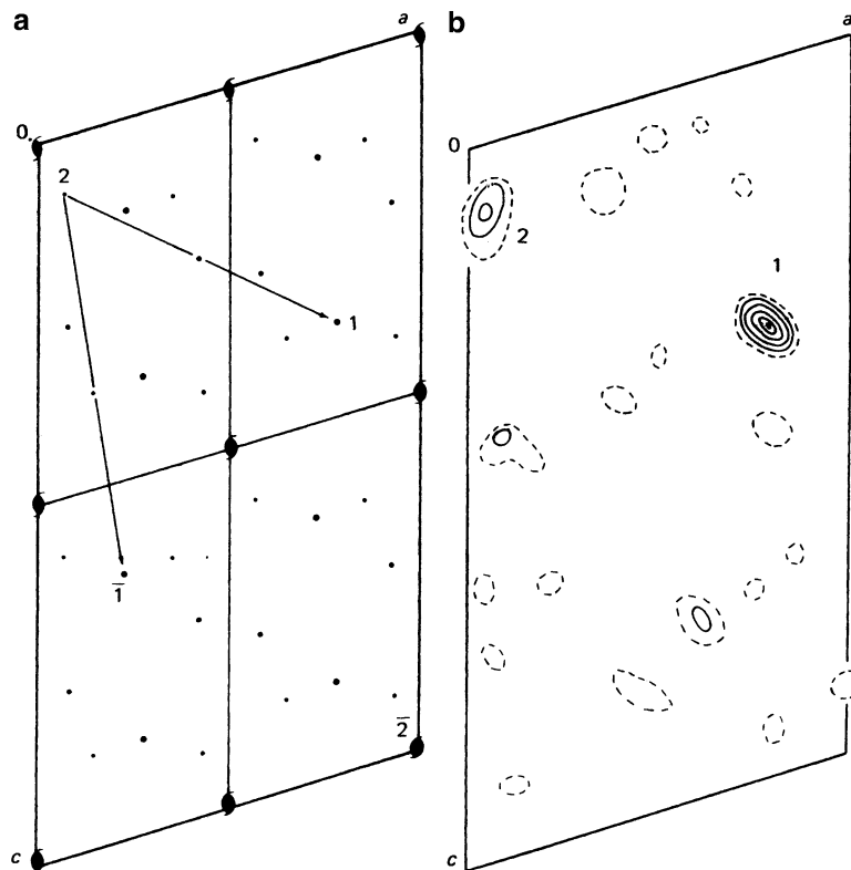
Fig. 7.31 Interpretation of the (\Delta F)^2 Patterson sections for ribonuclease. (a) Implication diagram. (b) Electron density map showing the Pt atom sites
