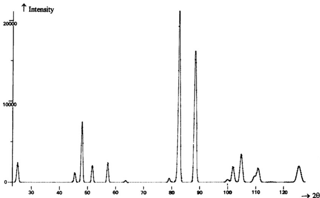
Fig. 12.11 Neutron diffraction pattern of a powdered sample of \text{CaUO}_4 , measured at \lambda = 2.565 \text{ \AA} ; the full line shows the calculated profile and the dots indicate the observed profile
