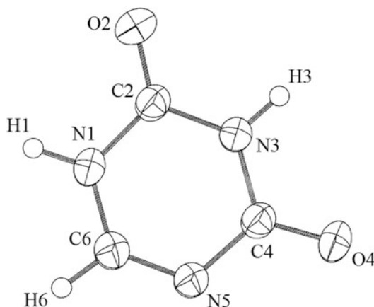
Fig. 8.34 View of the molecule of 5-azauracil molecule in the crystal structure, perpendicular to the molecular plane, showing 50% thermal ellipsoids
