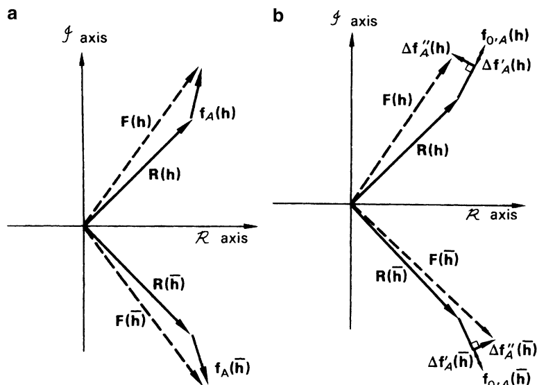
Fig. 7.39 Anomalous scattering of atom A with respect to the rest of the structure R . (a) Normal case: |F(\mathbf{h})| = |F(\bar{\mathbf{h}})| . (b) Anomalous case: |F(\mathbf{h})| \neq |F(\bar{\mathbf{h}})| . The general non-centrosymmetric case is illustrated. For centrosymmetric crystals, |F_{\mathbf{h}}| always equals |F_{\bar{\mathbf{h}}}| , but \phi_{\mathbf{h}} differs to a small degree from 0 or \pi if anomalous scattering is significant
