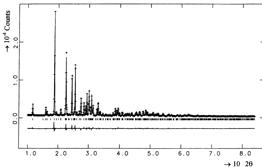
Fig. 12.21 Profile refinement for p\text{-BrC}_6\text{H}_4\text{CH}_2\text{CO}_2\text{H} ; the experimental points are marked + and the calculated profile is the full line. The lower line is the difference-Fourier profile
