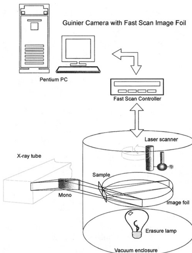
Fig. 12.6 Schematic diagram of the Huber Imaging Powder Camera. The powder pattern, collected on the imaging plate, is scanned by a laser and then digitized for computer analysis (courtesy Huber Diffraktionstechnik GmbH, 83253 Rimsting, Germany)
