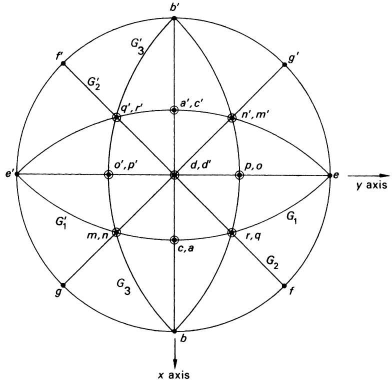
Fig. 1.18 Stereogram of the crystal shown in Fig. 1.17; the zone circle (great circle) G_1G'_1 , symbol [101] , passes through e, q, a, n, e', q', d', n' ; the zone circle G_2G'_2 symbol [1\bar{1}0] , passes through f, r, d, q', f', r', d', q ; the zone circle G_3G'_3 , symbol [011] , passes through b, m, o', q', b', m', o, q
