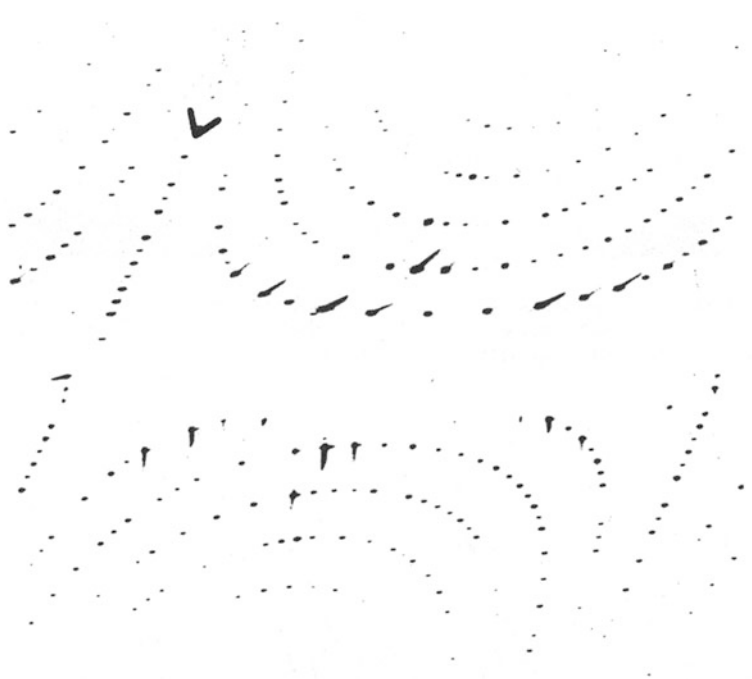
Fig. 9.6 Weissenberg photograph of the h1l layer. The 01l reciprocal lattice row, indicated by an arrowhead, illustrates clearly the effect of slight mis-setting of the crystal
