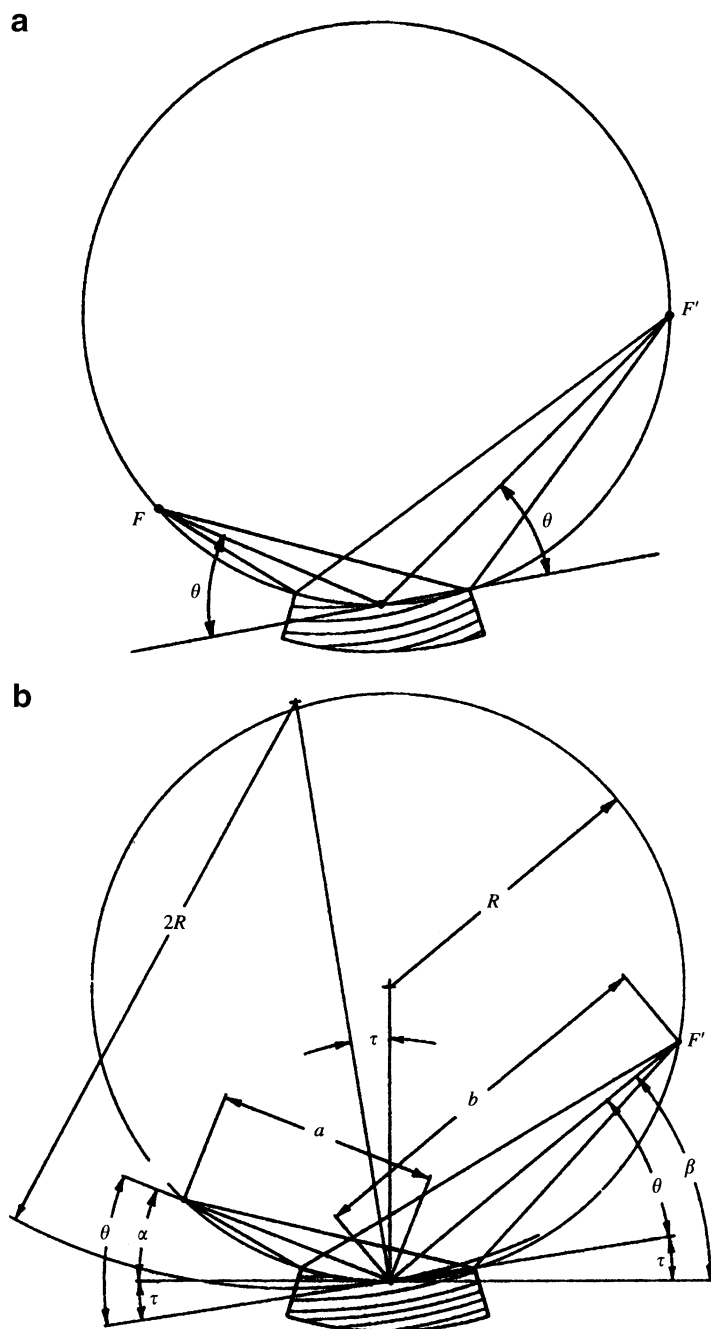
Fig. 12.4 (a) A curved crystal monochromator, showing the incident divergent bundle of rays from the X-ray tube at F reflected at the glancing angle \theta , and the bundle convergent at the point F' . (b) The curved crystal, showing the determinants involved in the setting of the crystal; the constancy of a and b with change of wavelength depends on the correct choice of \tau . (c) The principle of the Guinier method, showing the disposition of X-ray tube, monochromator, powder specimen, and focusing cylinder. The focusing cylinder carries a photographic film, or can be replaced by a scintillation counter (diffractometer) or an imaging plate (imaging camera) (courtesy Huber Diffraktionstechnik GmbH, 83253 Rimsting, Germany)
