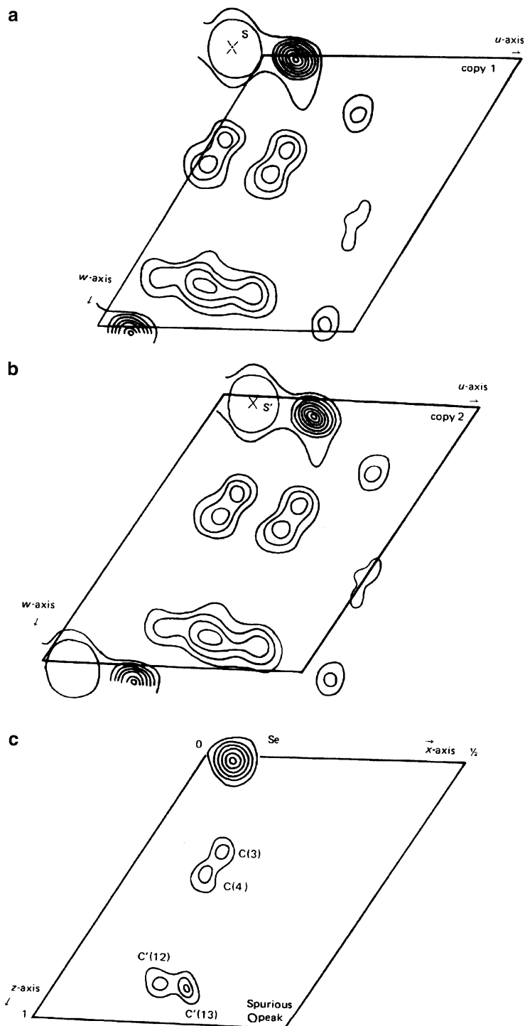
Fig. 7.14 Bisdiphenylmethyldiselenide. (a, b) Shifted copies 1 and 2 prepared from the (u0w) section. (c) Minimum-function M_2 section at y = 0.0 ; C'(12) and C'(13) are symmetry-related to C(12) and C(13) in Fig. 7.15
