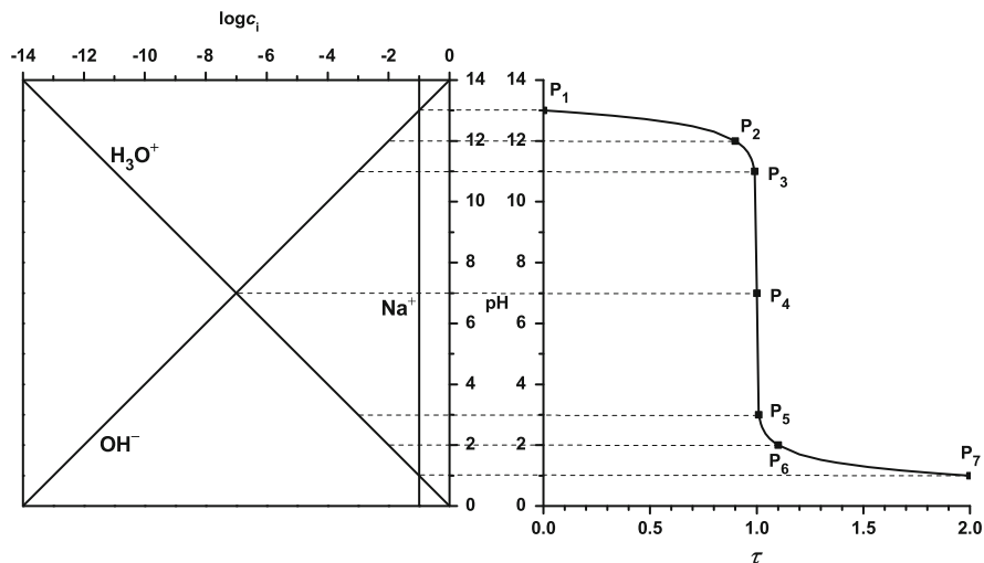
Fig. 75 Titration diagram of sodium hydroxide with hydrochloric acid ( \log C_{\text{NaOH}}^{\circ} = -1 )
