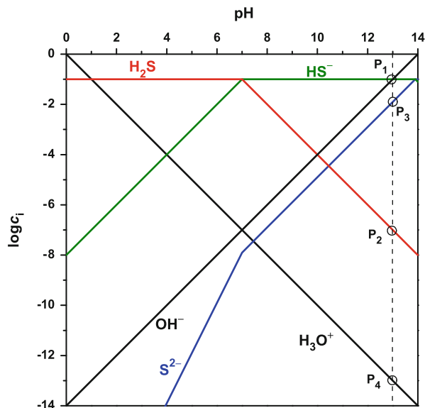
Fig. 54 pH-log c i diagram of a solution containing 0.1 mol L -1 Na 2 S
