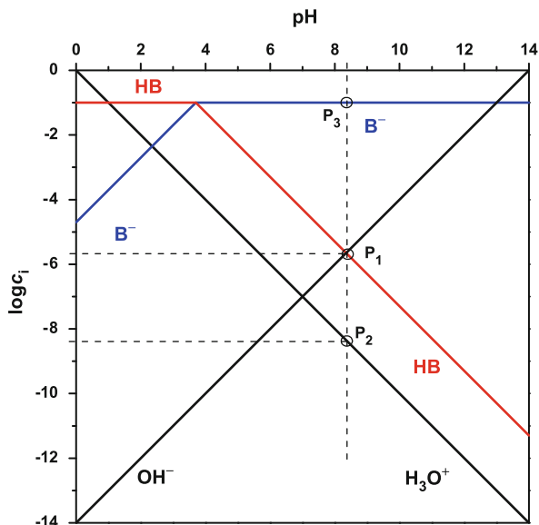
Fig. 39 pH- \log c_i diagram of sodium formate solution at C_{\text{HB}}^{\circ} = 10^{-1} \text{ mol L}^{-1} (Formic acid: \text{p}K_{\text{a}} = 3.75 )
