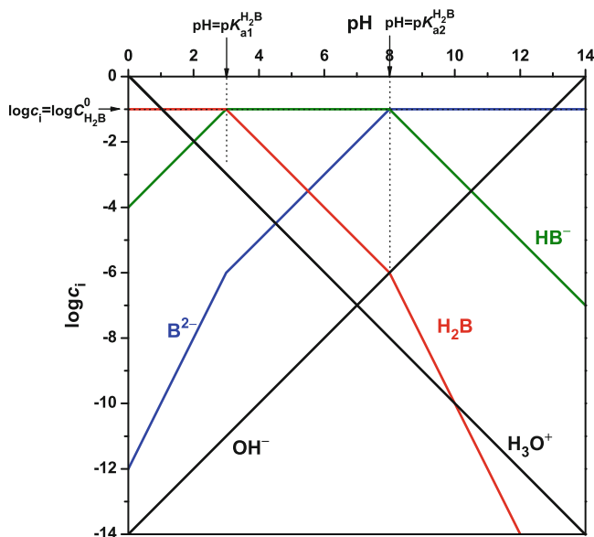
Fig. 19 Plotting the three lines of B^{2-} in the ranges pH < pK_{a1} , pK_{a1} < pH < pK_{a2} and pH > pK_{a2} . Example: acid with \log C_{H_2B}^0 = -1 , pK_{a1} = 3 and pK_{a2} = 8
