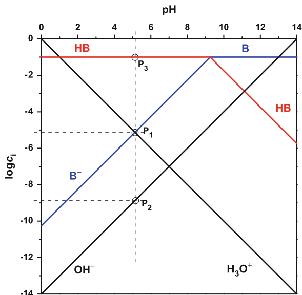
Fig. 41 pH-log i diagram of an ammonium chloride solution at C_{\text{HB}}^{\circ} = 10^{-1} mol L -1 (ammonium: pK_{\text{a}} = 9.25 )
