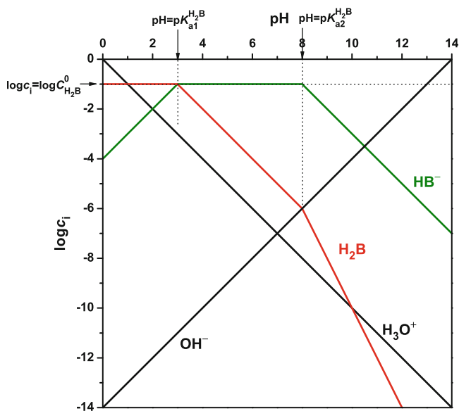
Fig. 18 Plotting the three lines of HB^- in the ranges pH < pK_{a1} , pK_{a1} < pH < pK_{a2} and pH > pK_{a2} . Example: acid with \log C_{H_2B}^0 = -1 , pK_{a1} = 3 and pK_{a2} = 8
