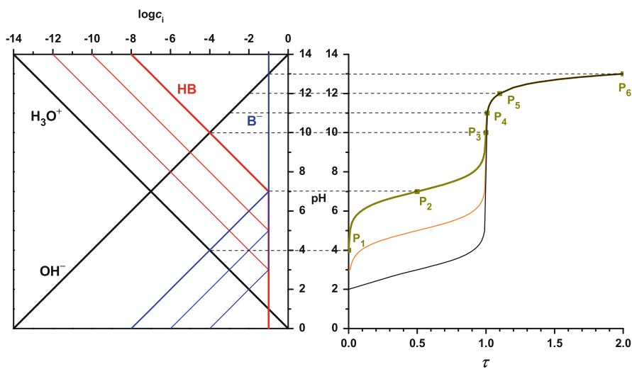
Fig. 80 Titration diagrams of three acids ( \log C_{\text{acid}}^{\circ} = -1 ) with pK_a = 3 (black line); pK_a = 5 (orange line) and pK_a = 7 (olive line) with sodium hydroxide solution. The distinctive points are given only for pK_a = 7
