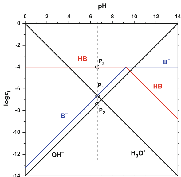
Fig. 42 pH-log i diagram of an ammonium chloride solution at C_{\text{HB}}^{\circ} = 10^{-4} mol L -1 (ammonium: pK_{\text{a}} = 9.25 )
