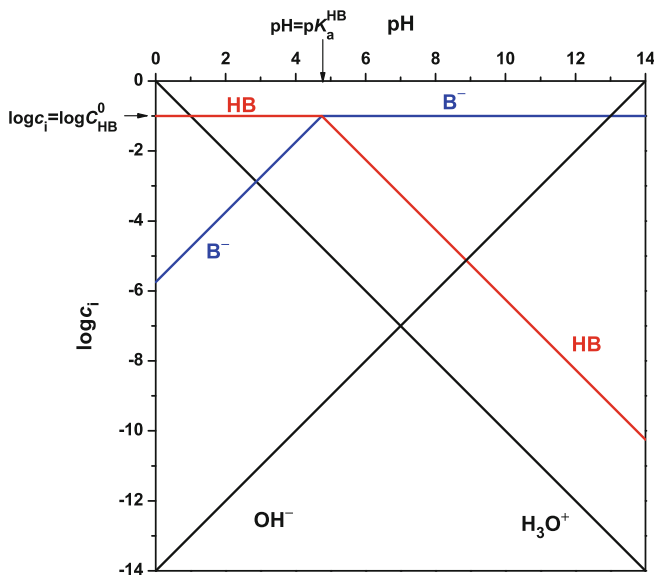
Fig. 9 The pH-log c i diagram with the H 3 O + line, the OH - line and the asymptotes of HB and B - for acetic acid with C HB 0 = 0.1 mol L -1 and pK a = 4.75
