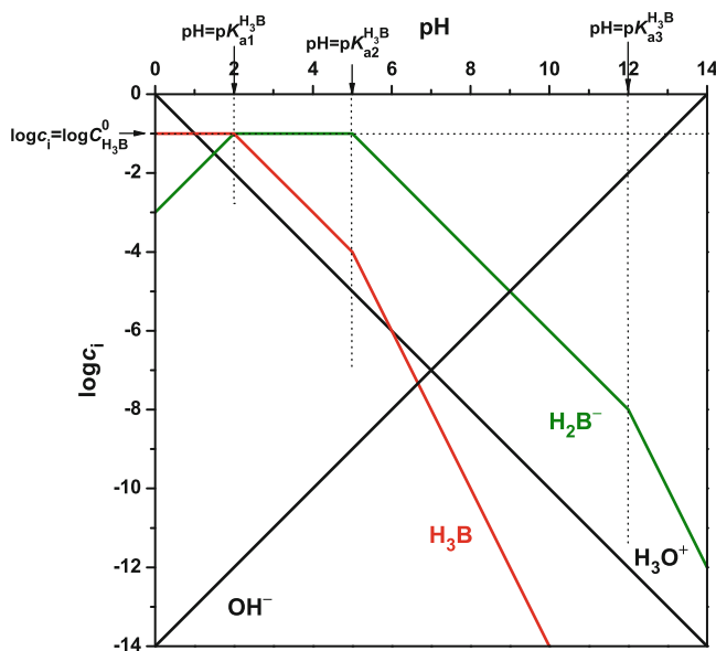
Fig. 23 Plotting the lines of H_2B^- in the ranges pH < pK_{a1} , pK_{a1} < pH < pK_{a2} , pK_{a2} < pH < pK_{a3} and pH > pK_{a3} . Example: \log C_{H_3B}^{\circ} = -1 , pK_{a1} = 2 , pK_{a2} = 5 and pK_{a3} = 12
