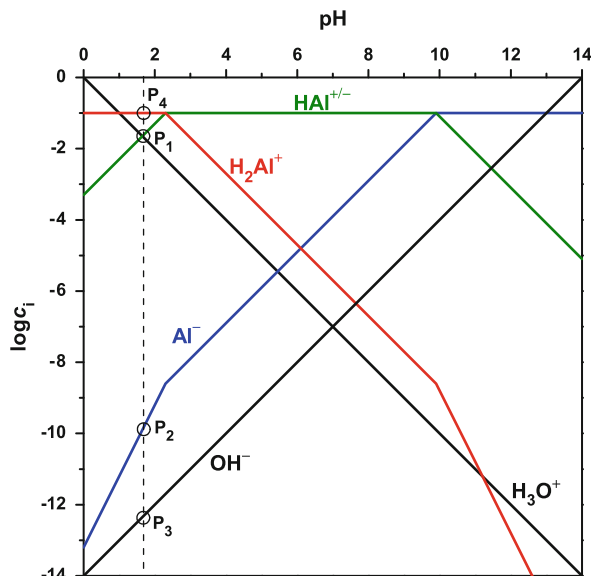
Fig. 50 pH- \log c_i diagram of an alanine hydrochloride ( \text{H}_2\text{Al}^+\text{Cl}^- ) solution of 0.1 \text{ mol L}^{-1} ( \text{p}K_{\text{a}1} = 2.3 , \text{p}K_{\text{a}2} = 9.9 )
