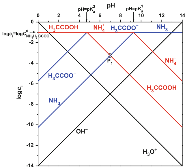
Fig. 57 pH-log i diagram of a solution containing 0.1 mol L -1 ammonium acetate
