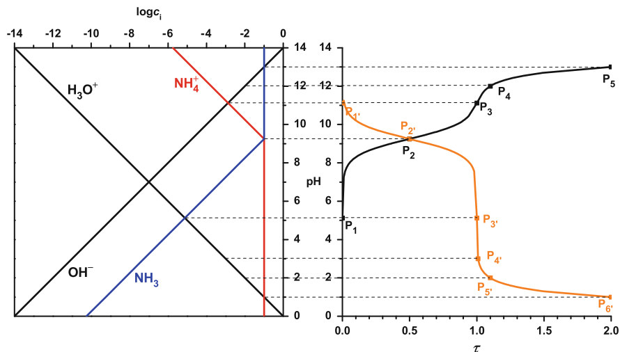
Fig. 83 Titration diagram of ammonia with hydrochloric acid (orange line) and ammonium ions (e.g., ammonium chloride) with sodium hydroxide (black line) ( \log C^\circ = -1 , \text{p}K_a^{\text{NH}_4^+} = 9.25 )
