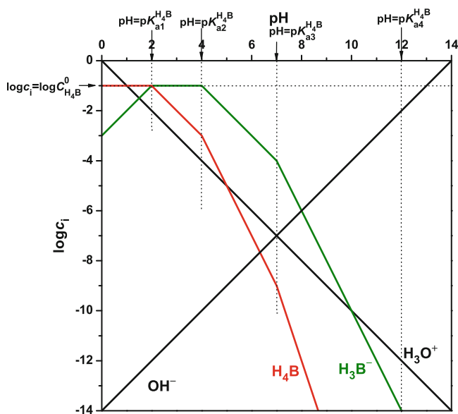
Fig. 28 Plotting the lines of \text{H}_3\text{B}^- for \text{pH} < \text{p}K_{a1} , \text{p}K_{a1} < \text{pH} < \text{p}K_{a2} , \text{p}K_{a2} < \text{pH} < \text{p}K_{a3} and \text{p}K_{a3} < \text{pH} < \text{p}K_{a4} . Example: acid with \log C_{\text{H}_4\text{B}}^0 = -1 , \text{p}K_{a1} = 2 , \text{p}K_{a2} = 4 , \text{p}K_{a3} = 7 and \text{p}K_{a4} = 12
