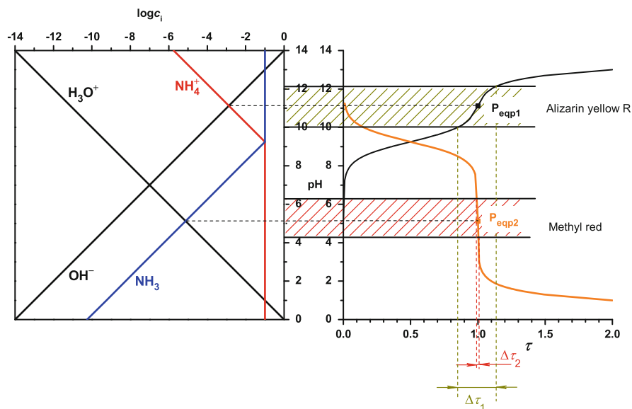
Fig. 88 pH- \log c_i diagram and diagram of the titrations of ammonia with hydrochloric acid (orange line with equivalence point P_{\text{eqp2}} ) and of ammonium ions with sodium hydroxide (black line with equivalence point P_{\text{eqp1}} ). The shadowed ranges indicate the transition ranges of the indicators alizarin yellow R and methyl red
