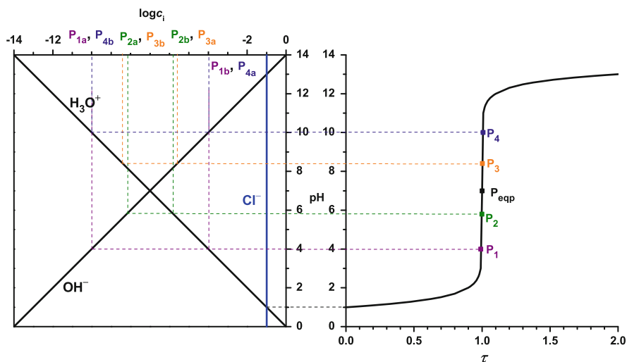
Fig. 86 Reading of the relevant concentration data from the pH- \log c_i diagram for estimation of the systematic titration errors in case of the titration of hydrochloric acid ( C_{\text{hydrochloric acid}}^{\circ} = 0.1 \text{ mol L}^{-1} ) with sodium hydroxide. P_{\text{eqp}} : equivalence point, P_1 to P_4 are the transition points of the color indicators methyl orange, methyl red, phenolphthalein, and thymolphthalein
