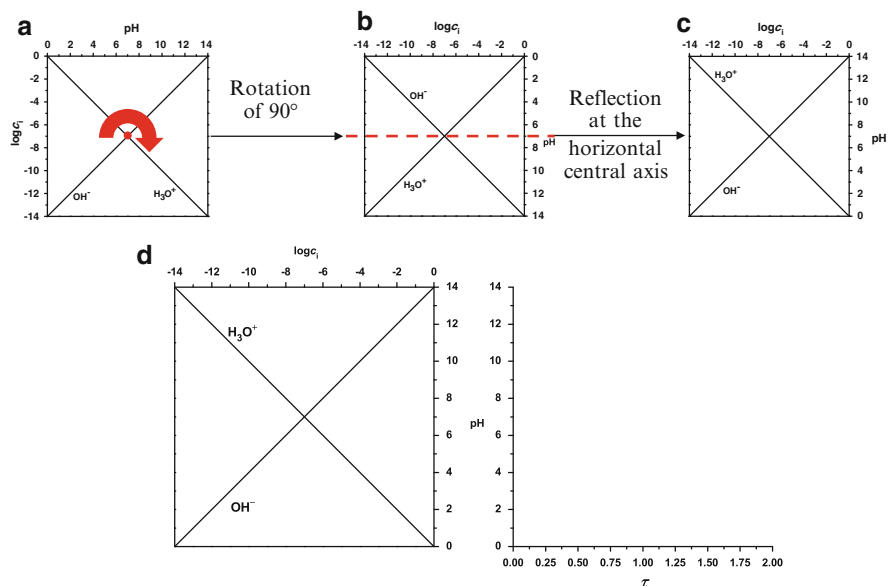
Fig. 72 (a) pH- \log c_i diagram. (b) pH- \log c_i following a turning by 90^\circ to the right side (around the center). (c) pH- \log c_i diagram resulting in (b) and mirrored at the middle axis (pH = 7). (d) pH- \log c_i diagram together with the titration diagram, so that both pH scales are parallel aligned
