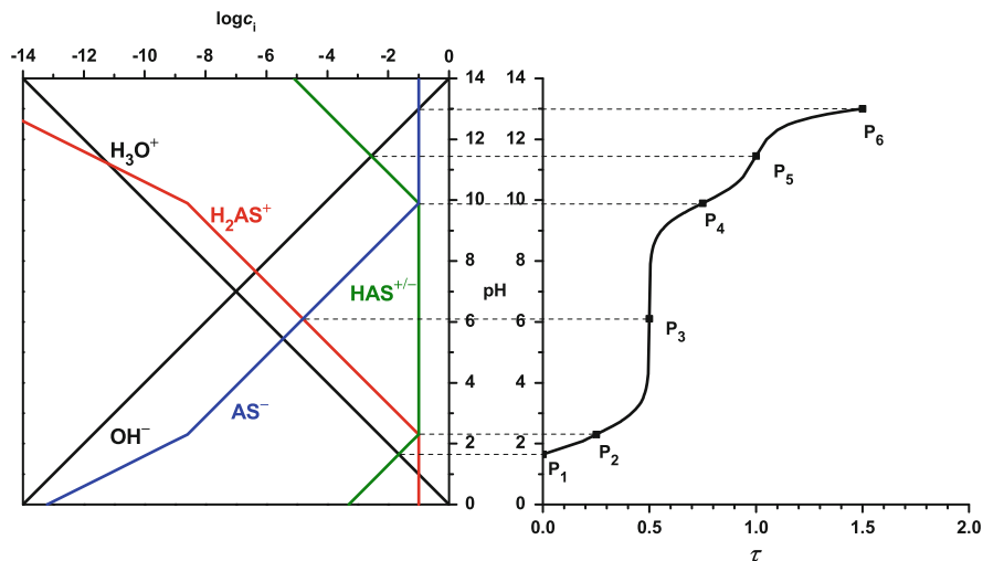
Fig. 82 Titration diagram of alanine ( \log C_{\text{alanine}}^{\circ} = -1 , pK_{a1} = 2.3 , pK_{a2} = 9.9 ) with sodium hydroxide
