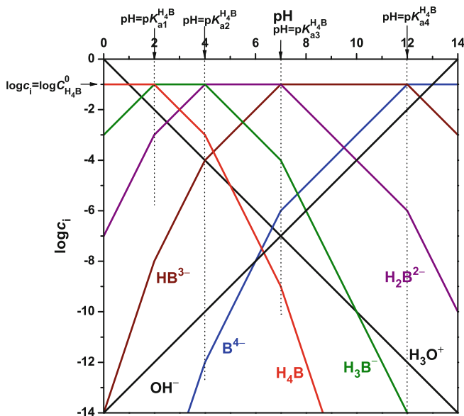
Fig. 31 Plotting the lines of \text{B}^{4-} for \text{p}K_{a1} < \text{pH} < \text{p}K_{a2} , \text{p}K_{a2} < \text{pH} < \text{p}K_{a3} , \text{p}K_{a3} < \text{pH} < \text{p}K_{a4} and \text{pH} > \text{p}K_{a4} . Example: acid with \log C_{\text{H}_4\text{B}}^0 = -1 , \text{p}K_{a1} = 2 , \text{p}K_{a2} = 4 , \text{p}K_{a3} = 7 and \text{p}K_{a4} = 12
