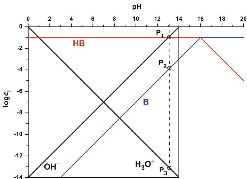
Fig. 45 pH- \log c_i diagram of an aqueous solution prepared by dissolving 10^{-1} mol of sodium ethanolate in water so that 1 l of solution results. The range \text{pH} > 14 is shown for didactic reasons only. Normally it is not shown
