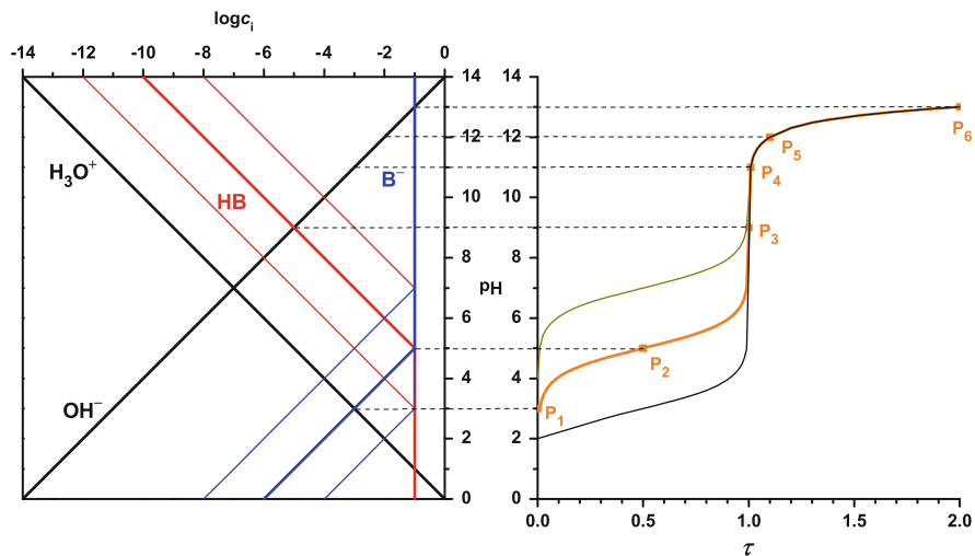
Fig. 79 Titration diagrams of three acids ( \log C_{\text{acid}}^{\circ} = -1 ) with pK_a = 3 (black line); pK_a = 5 (orange line) and pK_a = 7 (olive line) with sodium hydroxide solution. The distinctive points are given only for pK_a = 5
