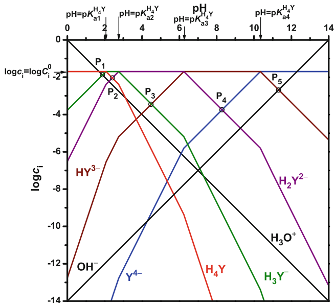
Fig. 70 pH- \log c_i of an EDTA solution ( \log C_i^0 = -1.70 , pK_{a1} = 2.07 , pK_{a2} = 2.75 , pK_{a3} = 6.24 , pK_{a4} = 10.34 )
