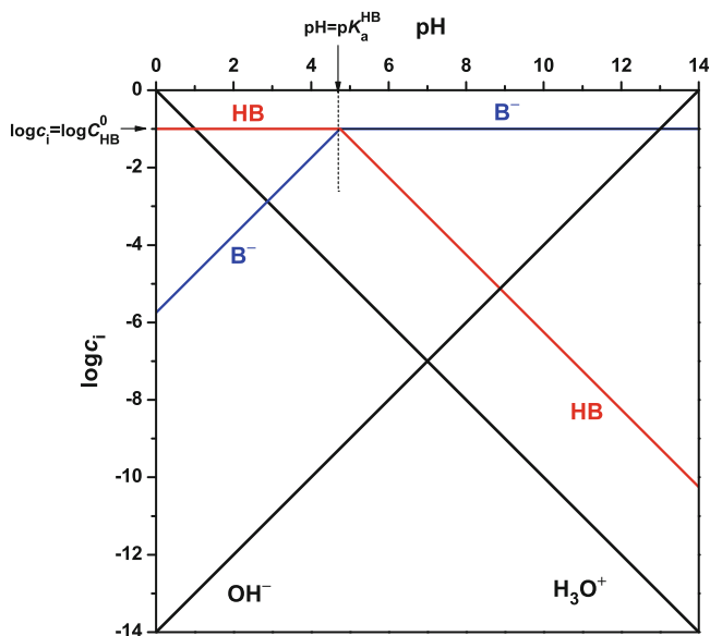
Fig. 14 Plotting the two asymptotes of B - with Eq. (35) for \text{pH} < \text{p}K_a and Eq. (36) for \text{pH} > \text{p}K_a . Example: acetic acid with C_{\text{HB}}^{\text{O}} = 0.1 \text{ mol L}^{-1} and \text{p}K_a = 4.75
