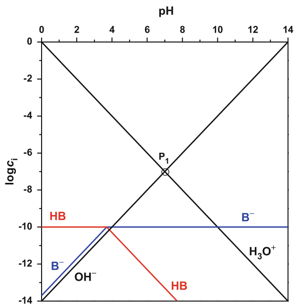
Fig. 38 pH- \log c_i diagram of formic acid ( pK_a = 3.75 ) at C_{HB}^{\circ} = 10^{-10} \text{ mol L}^{-1}
