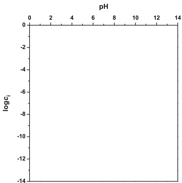
Fig. 10 The coordination system of the pH-log c_i diagram
