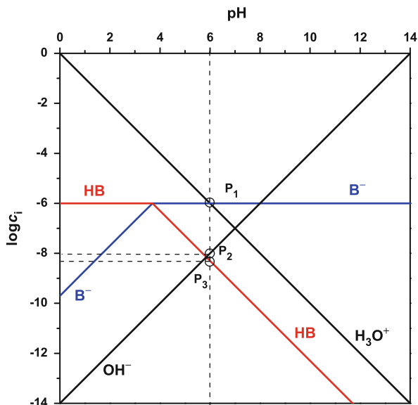
Fig. 37 pH- \log c_i diagram of formic acid ( pK_a = 3.75 ) at C_{HB}^{\circ} = 10^{-6} \text{ mol L}^{-1}
