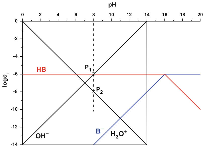
Fig. 46 pH-log c i diagram of an aqueous solution prepared by dissolving 10 -6 mol of sodium ethanolate in water so that 1 l of solution results. The range pH > 14 is shown for didactic reasons only. Normally it is not shown
