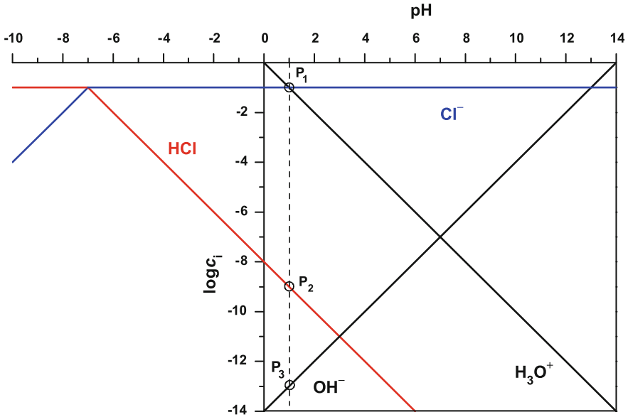
Fig. 32 pH- \log c_i diagram of hydrochloric acid ( pK_a = -7 ) at 0.1 \text{ mol L}^{-1} concentration. The range for \text{pH} < 0 is only shown for didactic reasons. Normally this is not done
