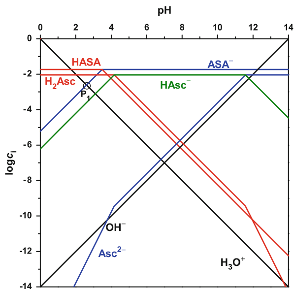
Fig. 66 pH-log i diagram for a solution containing 400 mg ASA and 240 mg vitamin C in 150 mL water
