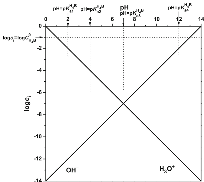
Fig. 26 Plotting the coordination system with the \text{H}_3\text{O}^+ and \text{OH}^- lines of water, and marking the coordinates, here for an example of an acid with \log c_i = \log C_{\text{H}_4\text{B}}^0 = -1 , \text{pH} = \text{p}K_{\text{a}1} = 2 , \text{pH} = \text{p}K_{\text{a}2} = 4 , \text{pH} = \text{p}K_{\text{a}3} = 7 and \text{pH} = \text{p}K_{\text{a}4} = 12
