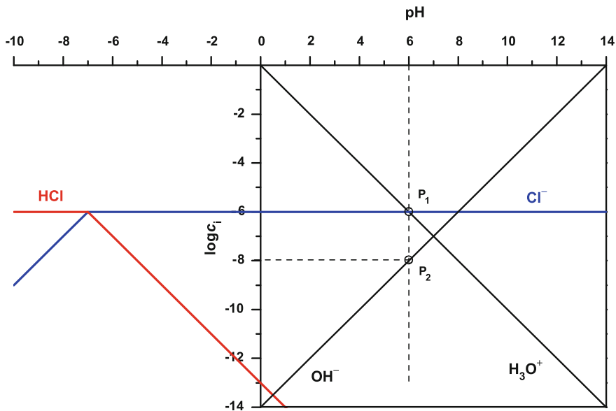
Fig. 33 pH-log i diagram of hydrochloric acid ( pK_a = -7 ) at 10^{-6} \text{ mol L}^{-1} concentration. The range for \text{pH} < 0 is only shown for didactic reasons. Normally this is not done
