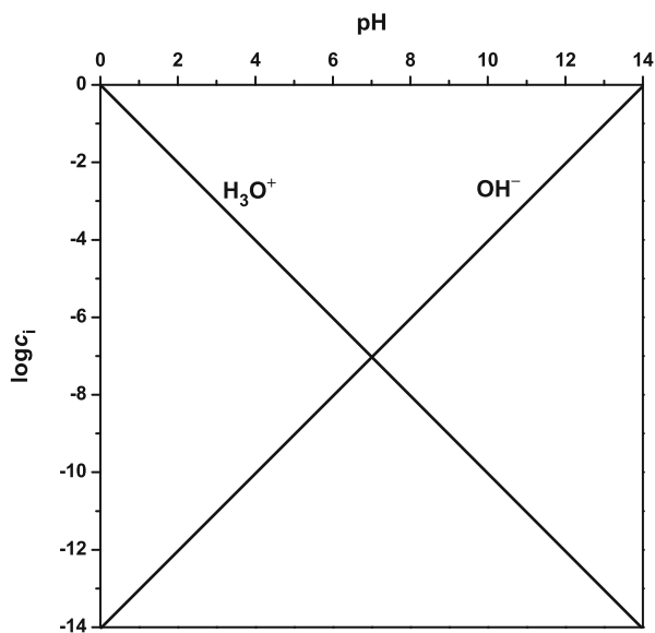
Fig. 11 Plotting the H 3 O + and OH - lines of the water system
