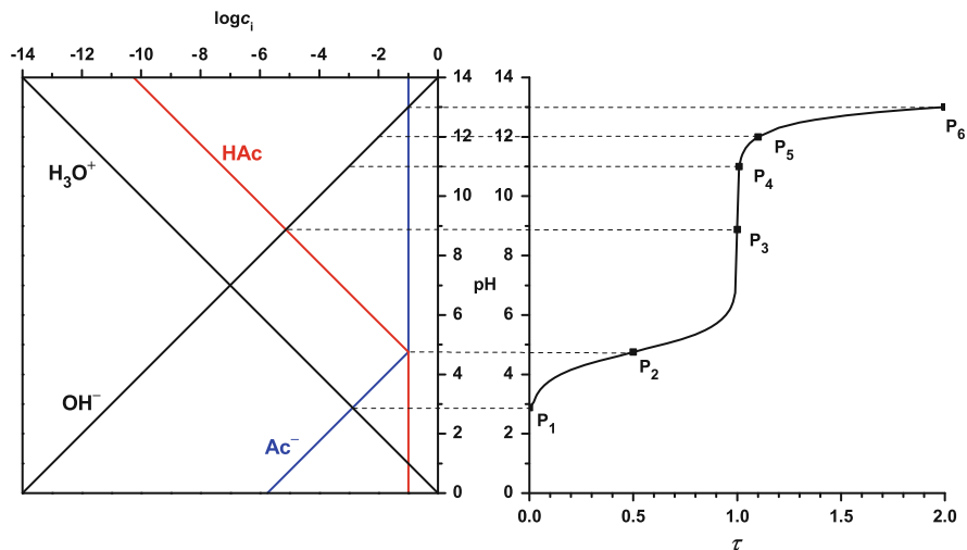
Fig. 76 Titration diagram of acetic acid ( \log C_{\text{acetic acid}}^{\circ} = -1 ; pK_a = 4.75 ) with sodium hydroxide
