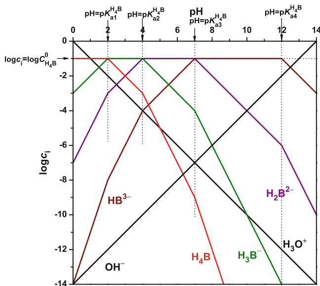
Fig. 30 Plotting the lines of \text{HB}^{3-} for \text{pH} < \text{p}K_{a1} , \text{p}K_{a1} < \text{pH} < \text{p}K_{a2} , \text{p}K_{a2} < \text{pH} < \text{p}K_{a3} , \text{p}K_{a3} < \text{pH} < \text{p}K_{a4} and \text{pH} > \text{p}K_{a4} . Example: acid with \log C_{\text{H}_4\text{B}}^0 = -1 , \text{p}K_{a1} = 2 , \text{p}K_{a2} = 4 , \text{p}K_{a3} = 7 and \text{p}K_{a4} = 12
