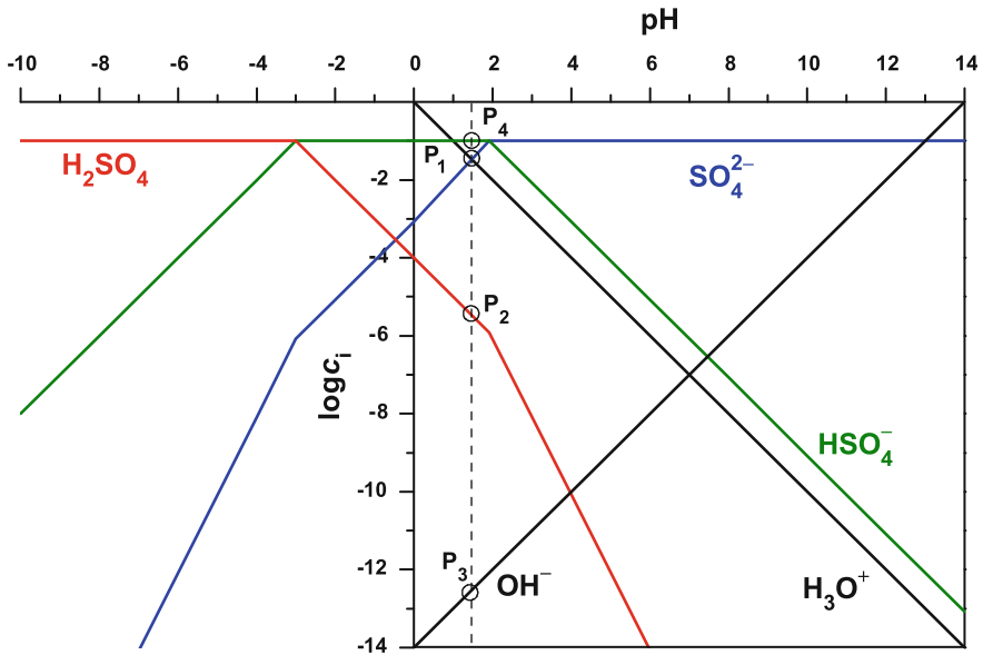
Fig. 52 pH-log i diagram of a NaHSO 4 solution at 10 -1 mol L -1 (pK a2 = 1.99 and pK b2 = 17). The range pH < 0 is shown for didactic reasons only. Normally it is not shown
