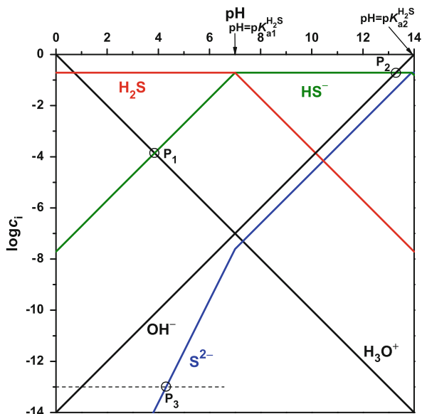
Fig. 62 pH- \log c_i diagram of hydrogen sulfide of hydrogen sulfide ( \log C_{\text{H}_2\text{S}}^\circ = -0.71 and pK_{a1} = 7.00 , pK_{a2} = 13.9 )
