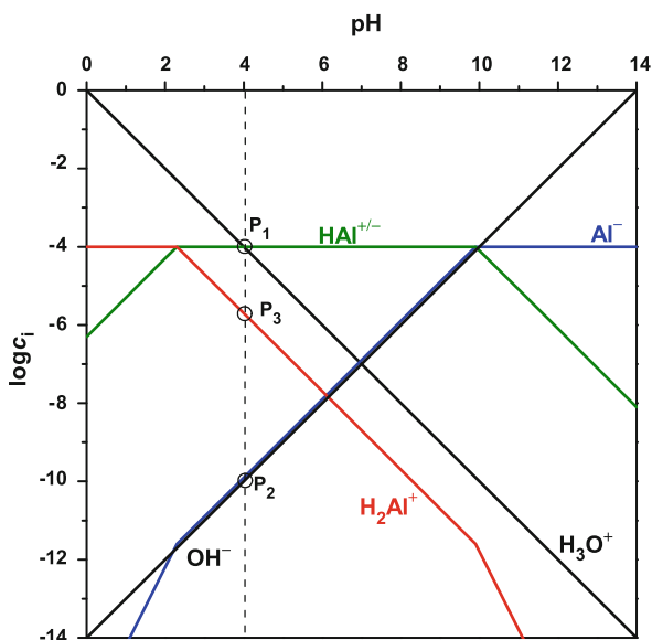
Fig. 51 pH-log i diagram of an alanine hydrochloride ( \text{H}_2\text{Al}^+\text{Cl}^- ) solution of 10^{-4} \text{ mol L}^{-1} ( \text{p}K_{\text{a}1} = 2.3 , \text{p}K_{\text{a}2} = 9.9 )
