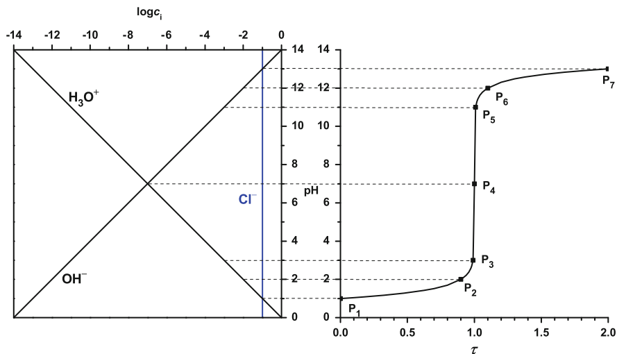
Fig. 73 Titration diagram of hydrochloric acid ( \log C_{\text{hydrochloric acid}}^{\circ} = -1 ) with sodium hydroxide solution
