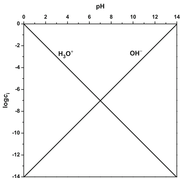
Fig. 20 Plotting the coordination system with the \text{H}_3\text{O}^+ and \text{OH}^- lines of water
