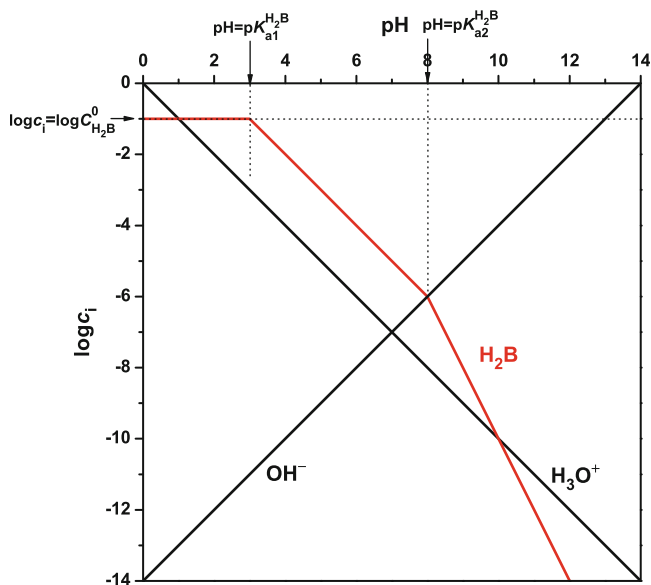
Fig. 17 Plotting the three lines of H_2B in the ranges pH < pK_{a1} , pK_{a1} < pH < pK_{a2} and pH > pK_{a2} . Example: acid with \log C_{H_2B}^0 = -1 , pK_{a1} = 3 and pK_{a2} = 8
