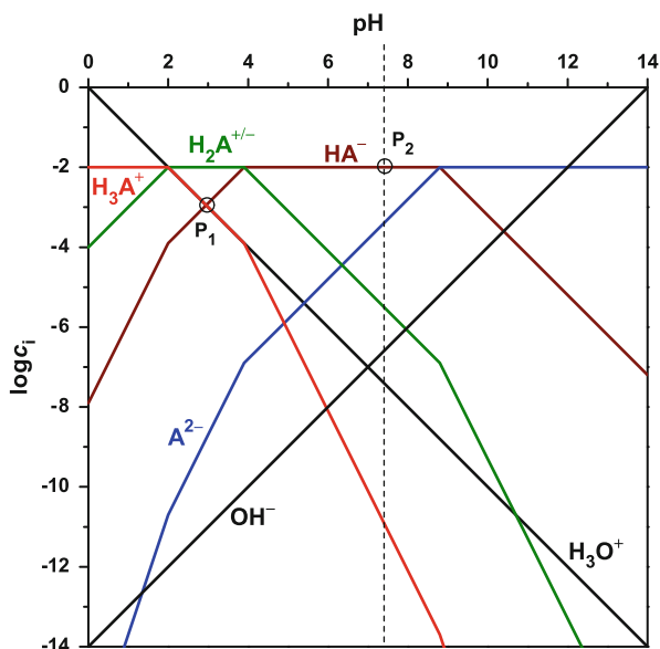
Fig. 69 pH- \log c_i diagram of aspartic acid at an overall concentration of 0.01 mol L -1
