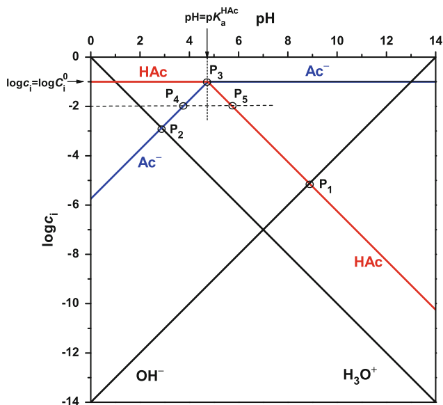
Fig. 61 pH-log i c i diagram of the corresponding acid–base pair acetic acid/acetate ions \log C_i^0 = -1.00 , pK_a = 4.75
