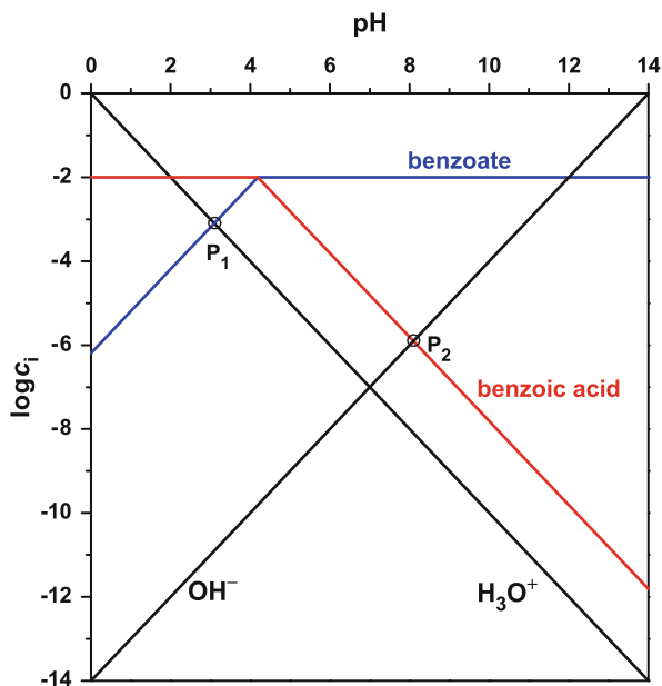
Fig. 67 pH- \log c_i diagram of benzoic acid at an overall concentration of 0.01 \text{ mol L}^{-1}
