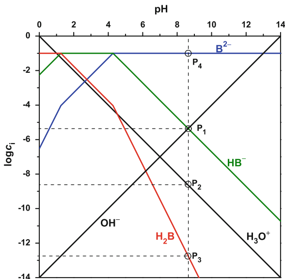
Fig. 55 pH-log c diagram of a solution containing 0.1 mol L -1 of sodium oxalate (oxalate: pK b1 = 9.73 and pK b2 = 12.73)
