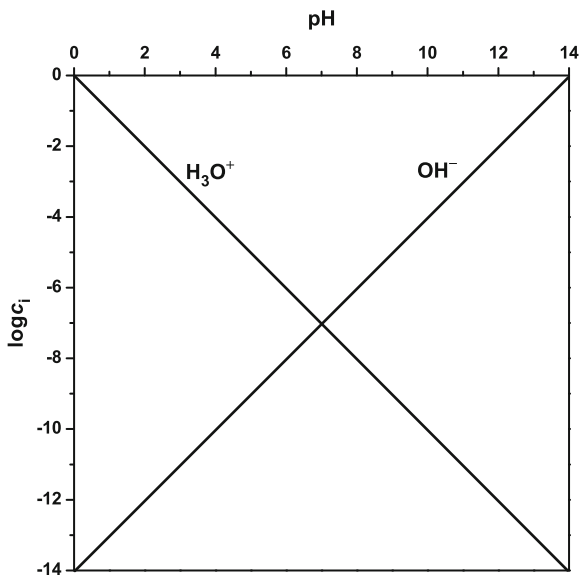
Fig. 15 Plotting the coordination system with the \text{H}_3\text{O}^+ and \text{OH}^- lines of water
