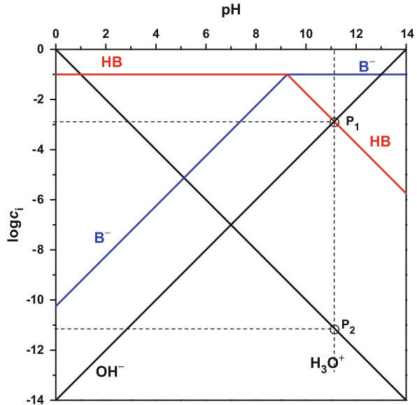
Fig. 43 pH-log i diagram of an ammonia solution, C_{\text{ammonia}}^{\circ} = 10^{-1} \text{ mol L}^{-1} (Ammonium: \text{p}K_a = 9.25 )
