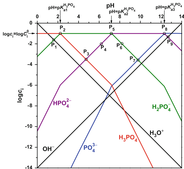
Fig. 63 pH-log c i diagram of phosphoric acid ( \log C_i^0 = -1.00 and pK_{a1} = 2.15 , pK_{a2} = 7.2 and pK_{a3} = 12.35 )
