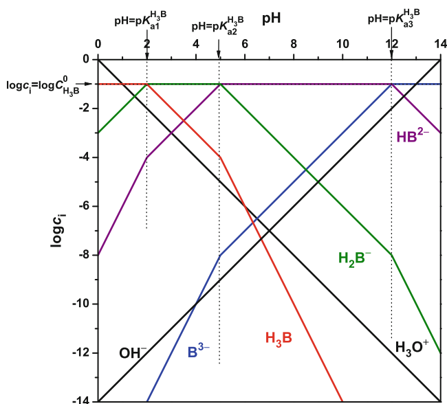
Fig. 25 Plotting the lines of \text{B}^{3-} in the ranges \text{p}K_{a1} < \text{pH} < \text{p}K_{a2} , \text{p}K_{a2} < \text{pH} < \text{p}K_{a3} and \text{pH} > \text{p}K_{a3} . The line for \text{pH} < \text{p}K_{a1} is situated outside the range of the coordination system. Example: \log C_{\text{H}_3\text{B}}^{\circ} = -1 , \text{p}K_{a1} = 2 , \text{p}K_{a2} = 5 and \text{p}K_{a3} = 12
