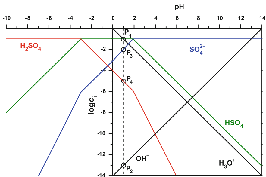
Fig. 48 pH- \log c_i diagram of a solution containing 0.1 \text{ mol L}^{-1} of sulfuric acid. The range \text{pH} < 0 is shown for didactic reasons only. Normally it is not shown
