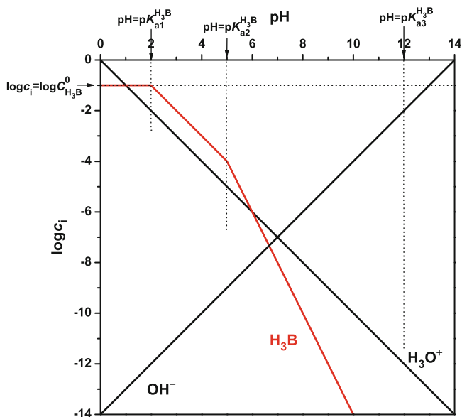
Fig. 22 Plotting the three lines of H_3B in the ranges pH < pK_{a1} , pK_{a1} < pH < pK_{a2} and pK_{a2} < pH < pK_{a3} . The line of H_3B for pH > pK_{a3} is situated outside the range of the diagram. Example: \log C_{H_3B}^{\circ} = -1 , pK_{a1} = 2 , pK_{a2} = 5 and pK_{a3} = 12
