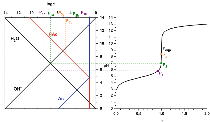
Fig. 84 Reading of the relevant concentration data from the \text{pH}-\log c_i diagram for estimation of the systematic titration errors in case of the titration of acetic acid ( C_{\text{acetic acid}}^{\circ} = 0.1 \text{ mol L}^{-1} ) with sodium hydroxide. P_{\text{eq}} : equivalence point, P_1 to P_3 are transition points of the indicators methyl red, neutral red, and phenolphthalein
