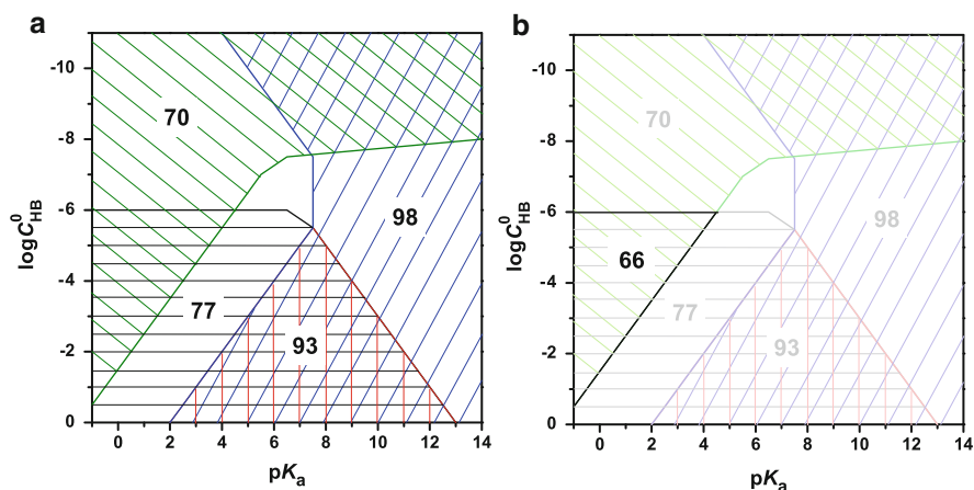
Fig. 47 (a) Validity ranges of the simplified equations (70), (77), (93), and (98). (b) Validity range of the simplified equation (66). For the calculation of the borderlines (validity ranges), a maximum allowable error of 0.02 pH units has been fixed
