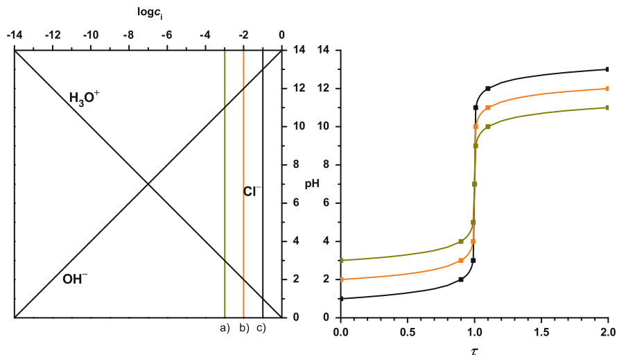
Fig. 74 Titration diagram of hydrochloric acid solutions of different concentrations with sodium hydroxide solution. (a) \log C_{\text{hydrochloric acid}}^{\circ} = -3 . (b) \log C_{\text{hydrochloric acid}}^{\circ} = -2 . (c) \log C_{\text{hydrochloric acid}}^{\circ} = -1
