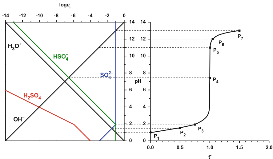
Fig. 81 Titration diagram of sulfuric acid ( \log C_{\text{sulfuric acid}}^{\circ} = -1 ), \text{p}K_{\text{a}1} = -3 , \text{p}K_{\text{a}2} = 1.99 with sodium hydroxide
