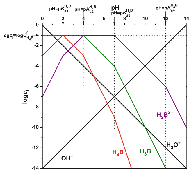
Fig. 29 Plotting the lines of \text{H}_2\text{B}^{2-} for \text{pH} < \text{p}K_{a1} , \text{p}K_{a1} < \text{pH} < \text{p}K_{a2} , \text{p}K_{a2} < \text{pH} < \text{p}K_{a3} , \text{p}K_{a3} < \text{pH} < \text{p}K_{a4} and \text{pH} > \text{p}K_{a4} . Example: acid with \log C_{\text{H}_4\text{B}}^0 = -1 , \text{p}K_{a1} = 2 , \text{p}K_{a2} = 4 , \text{p}K_{a3} = 7 and \text{p}K_{a4} = 12
