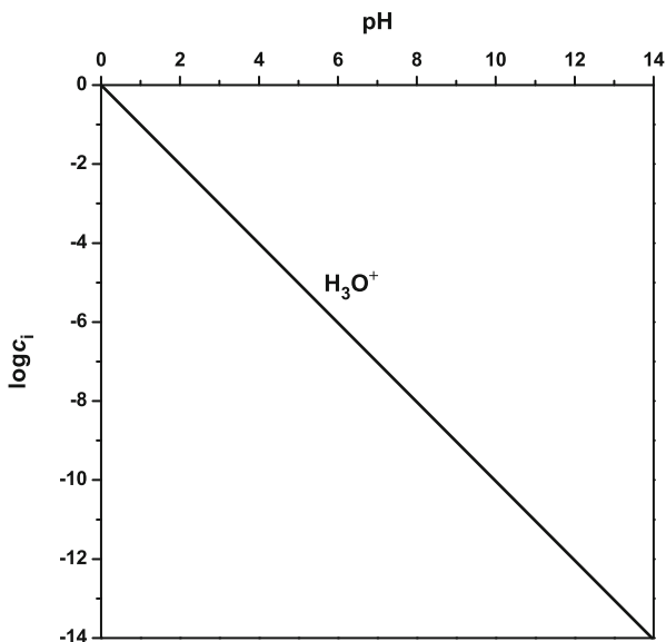
Fig. 5 The pH-log i diagram with the H 3 O + line of water
