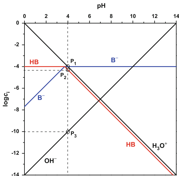
Fig. 36 pH-log i diagram of formic acid ( \text{p}K_a = 3.75 ) at C_{\text{HB}}^{\circ} = 10^{-4} \text{ mol L}^{-1}
