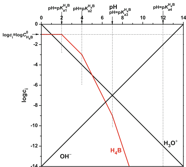
Fig. 27 Plotting the lines of \text{H}_4\text{B} for \text{pH} < \text{p}K_{\text{a}1} , \text{p}K_{\text{a}1} < \text{pH} < \text{p}K_{\text{a}2} , \text{p}K_{\text{a}2} < \text{pH} < \text{p}K_{\text{a}3} and \text{p}K_{\text{a}3} < \text{pH} < \text{p}K_{\text{a}4} . The line of \text{H}_4\text{B} for \text{pH} > \text{p}K_{\text{a}4} is situated outside the plotted range. Example: acid with \log C_{\text{H}_4\text{B}}^0 = -1 , \text{p}K_{\text{a}1} = 2 , \text{p}K_{\text{a}2} = 4 , \text{p}K_{\text{a}3} = 7 and \text{p}K_{\text{a}4} = 12
