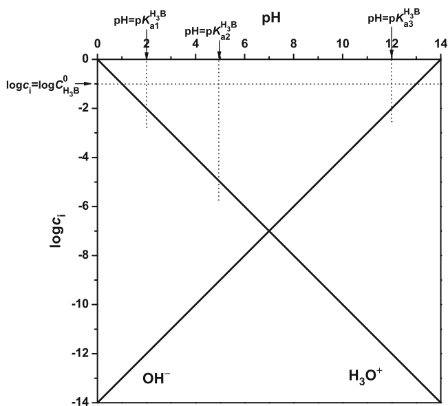
Fig. 21 Marking the coordinates, here for an acid with \log c_i = \log C_{\text{H}_3\text{B}}^0 = -1 , \text{pH} = \text{p}K_{\text{a}1} = 2 , \text{pH} = \text{p}K_{\text{a}2} = 5 and \text{pH} = \text{p}K_{\text{a}3} = 12
