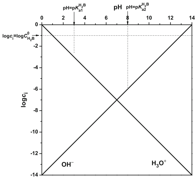
Fig. 16 Marking the coordinates, here for the example of an acid with \log c_i = \log C_{\text{H}_2\text{B}}^0 = -1 , \text{pH} = \text{p}K_{a1} = 3 and \text{pH} = \text{p}K_{a2} = 8
