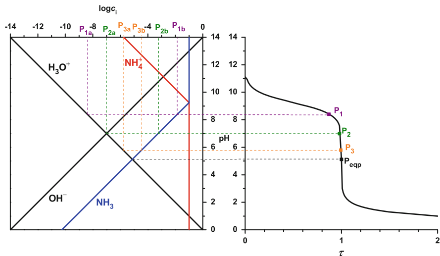
Fig. 85 Reading of the relevant concentration data from the pH- \log c_i diagram for estimation of the systematic titration errors in case of the titration of ammonia ( C_{\text{ammonia}}^{\circ} = 0.1 \text{ mol L}^{-1} ) with hydrochloric acid using different color indicators: P_{\text{eq}} : equivalence point, P_1 to P_3 are the transition points of the indicators phenolphthalein, neutral red, and methyl red
