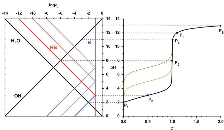
Fig. 78 Titration diagrams of three acids ( \log C_{\text{acid}}^{\circ} = -1 ) with \text{p}K_a = 3 (black line), \text{p}K_a = 5 (orange line), and \text{p}K_a = 7 (olive line) with sodium hydroxide solution. The distinctive points are given only for \text{p}K_a = 3
