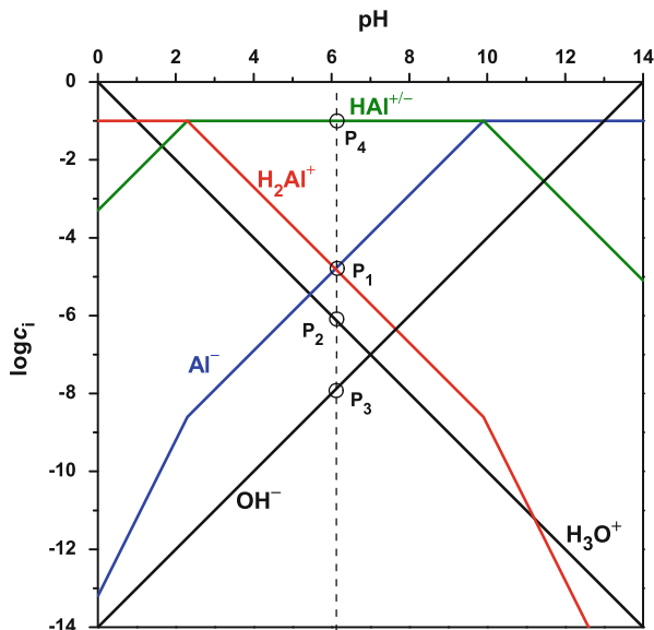
Fig. 53 pH- \log c_i diagram of a solution containing 10^{-1} \text{ mol L}^{-1} alanine ( \text{p}K_{a1} = 2.3 , \text{p}K_{a2} = 9.9 ) ( \text{H}_2\text{Al}^+ corresponds to \text{H}_2\text{B} , \text{HAl}^{+/-} corresponds to \text{HB}^- , and \text{Al}^- corresponds to \text{B}^{2-} of the dibasic acids \text{H}_2\text{B} )
