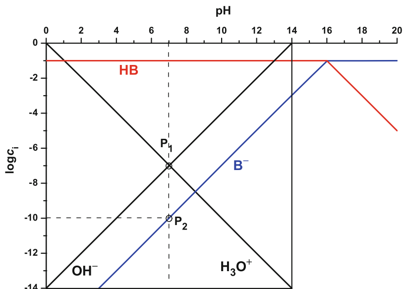
Fig. 44 \text{pH}-\log c_i diagram of an aqueous solution of 10^{-1} \text{ mol L}^{-1} ethanol ( \text{p}K_a = 16 ). The range of \text{pH} > 14 is shown for didactic reasons only. Normally it is not shown
