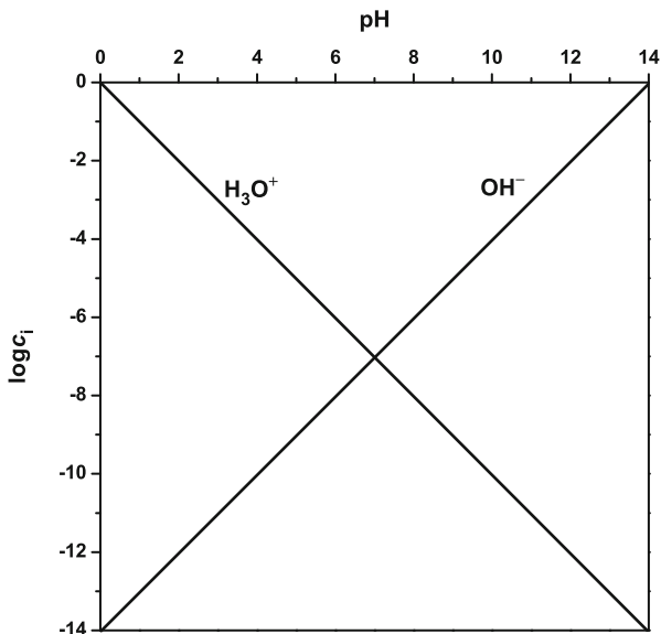
Fig. 6 The pH-log c diagram with the H 3 O + and OH - lines of water
