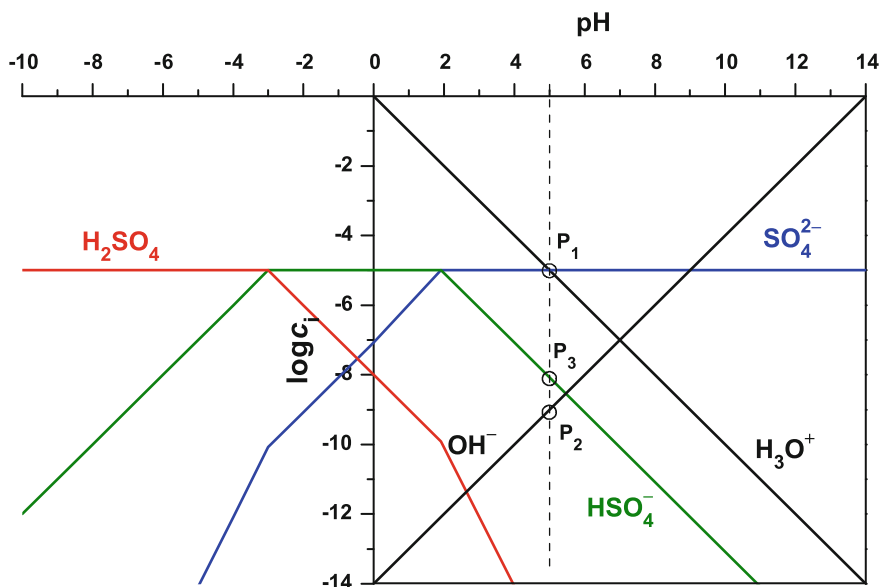
Fig. 49 pH- \log c_i diagram of sulfuric acid at 10^{-5} \text{ mol L}^{-1} . The range \text{pH} < 0 is shown for didactic reasons only. Normally it is not shown
