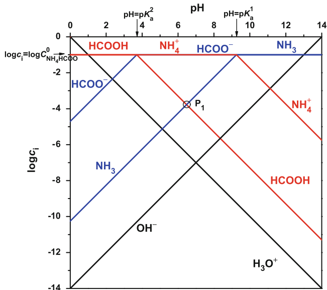
Fig. 56 pH-log i diagram of a solution containing 0.1 mol L -1 ammonium formate
