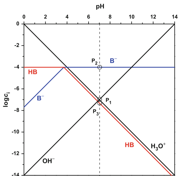
Fig. 40 pH- \log c_i diagram of sodium formate solution at C_{\text{HB}}^{\circ} = 10^{-4} \text{ mol L}^{-1} (Formic acid: \text{p}K_{\text{a}} = 3.75 )
