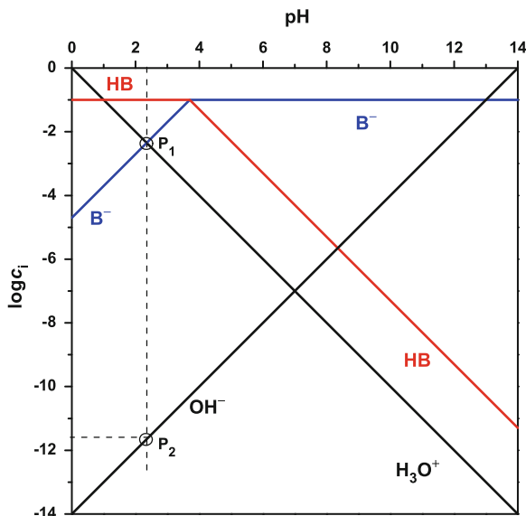
Fig. 35 pH- \log c_i diagram for formic acid ( \text{p}K_a = 3.75 ) at C_{\text{HB}}^{\circ} = 10^{-1} \text{ mol L}^{-1}
