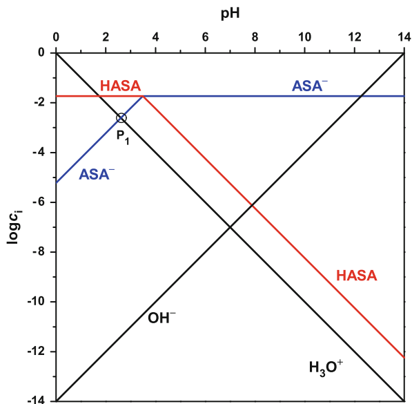
Fig. 65 pH-log i diagram of an ASA solution ( \log C_1^{\circ} = -1.73 , pK_a = 3.48 )
