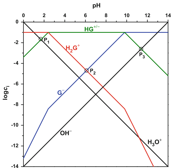
Fig. 68 pH-log c_i diagram of glycine at an overall concentration of 0.1 mol L -1
