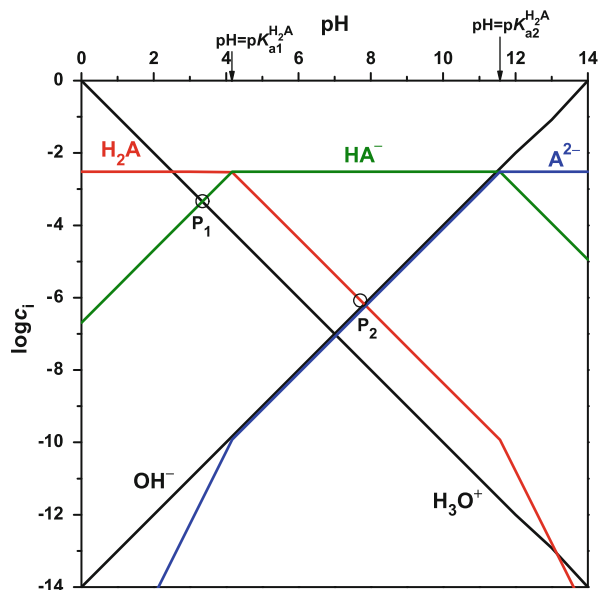
Fig. 64 pH- \log c_i diagram of ascorbic acid ( \log C_i^\circ = -2.52 , pK_{a1} = 4.17 , pK_{a2} = 11.57 )
