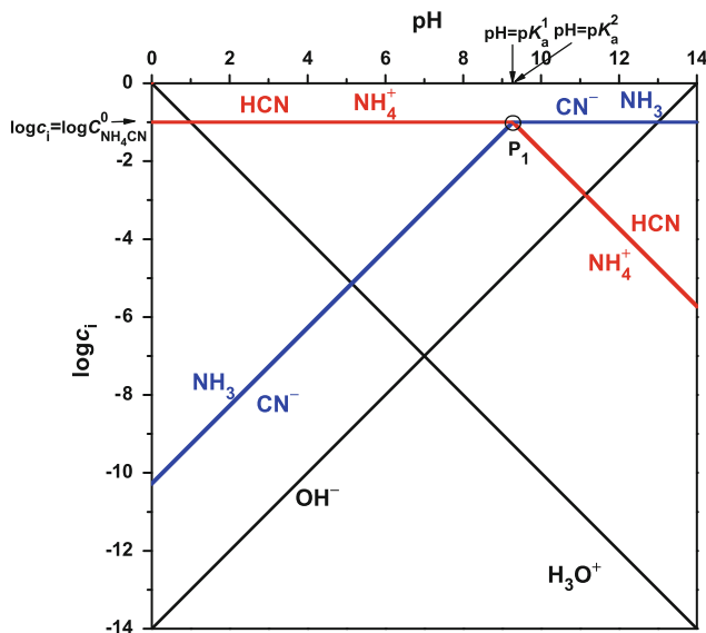
Fig. 58 pH- \log c_i diagram of a solution containing 0.1 \text{ mol L}^{-1} ammonium cyanide
