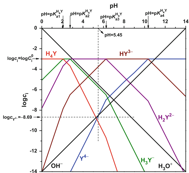
Fig. 71 pH- \log c_i diagram of EDTA ( \log C_i^0 = -3 , pK_{a1} = 2.07 , pK_{a2} = 2.75 , pK_{a3} = 6.24 , pK_{a4} = 10.34 )
