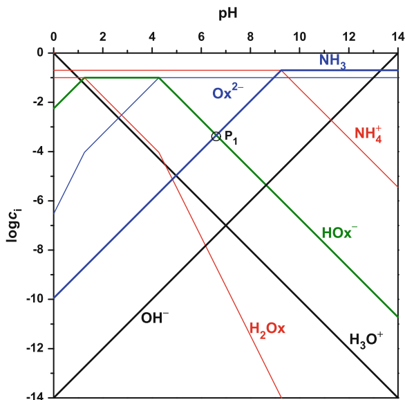
Fig. 59 pH-log i diagram of a solution containing 0.1 mol L -1 ammonium oxalate
