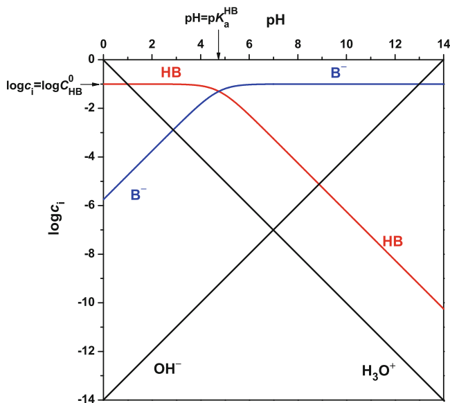
Fig. 8 The pH-log i diagram with the lines of H 3 O + , OH - , HB and B - for acetic acid with C HB 0 = 0.1 mol L -1 and pK a = 4.75
