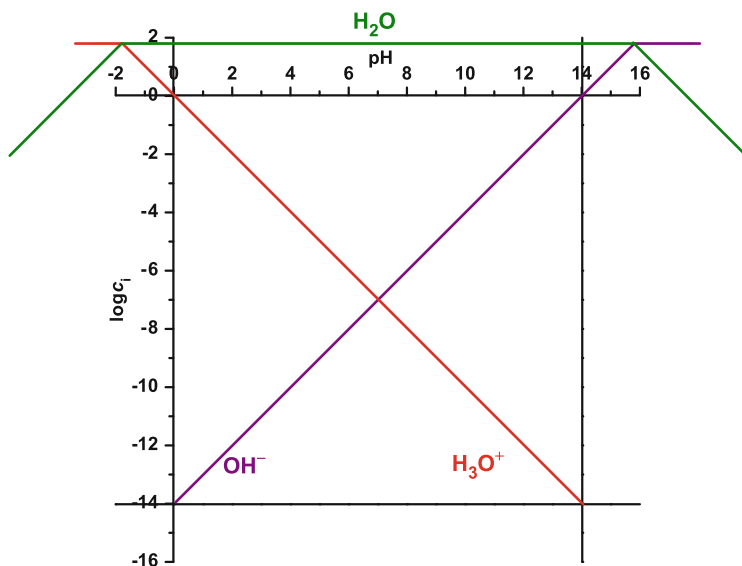
Fig. 60 pH- \log c_i diagram of water with \log C_{\text{H}_2\text{O}}^\circ = 1.74 and the two not entirely correct values \text{p}K_a(\text{H}_3\text{O}^+) = -1.74 and \text{p}K_a(\text{H}_2\text{O}) = 15.74
