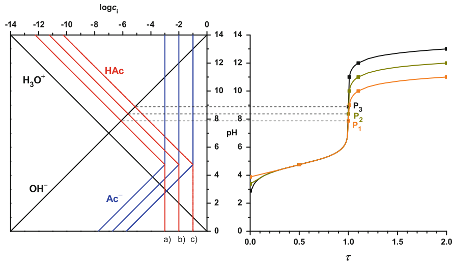
Fig. 77 Titration diagrams of acetic acid of different concentrations ( pK_a = 4.75 ) with sodium hydroxide. (a) \log C_{\text{acetic acid}}^{\circ} = -3 . (b) \log C_{\text{acetic acid}}^{\circ} = -2 . (c) \log C_{\text{acetic acid}}^{\circ} = -1
