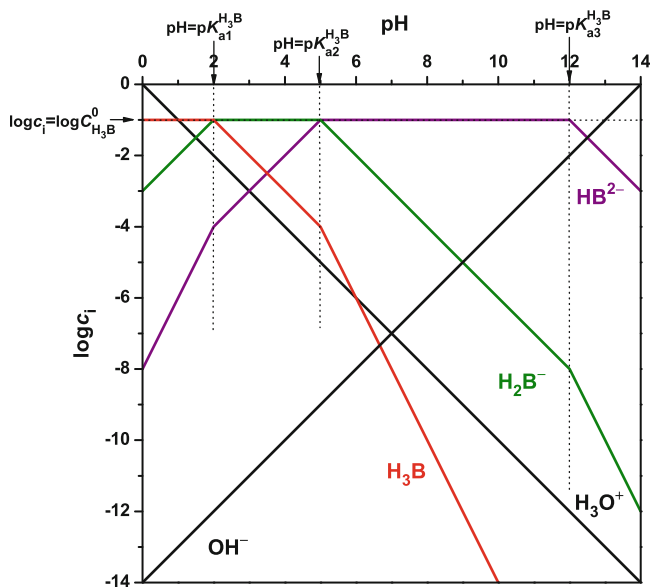
Fig. 24 Plotting the lines of \text{HB}^{2-} in the ranges \text{pH} < \text{p}K_{a1} , \text{p}K_{a1} < \text{pH} < \text{p}K_{a2} , \text{p}K_{a2} < \text{pH} < \text{p}K_{a3} and \text{pH} > \text{p}K_{a3} . Example: \log C_{\text{H}_3\text{B}}^{\circ} = -1 , \text{p}K_{a1} = 2 , \text{p}K_{a2} = 5 and \text{p}K_{a3} = 12
