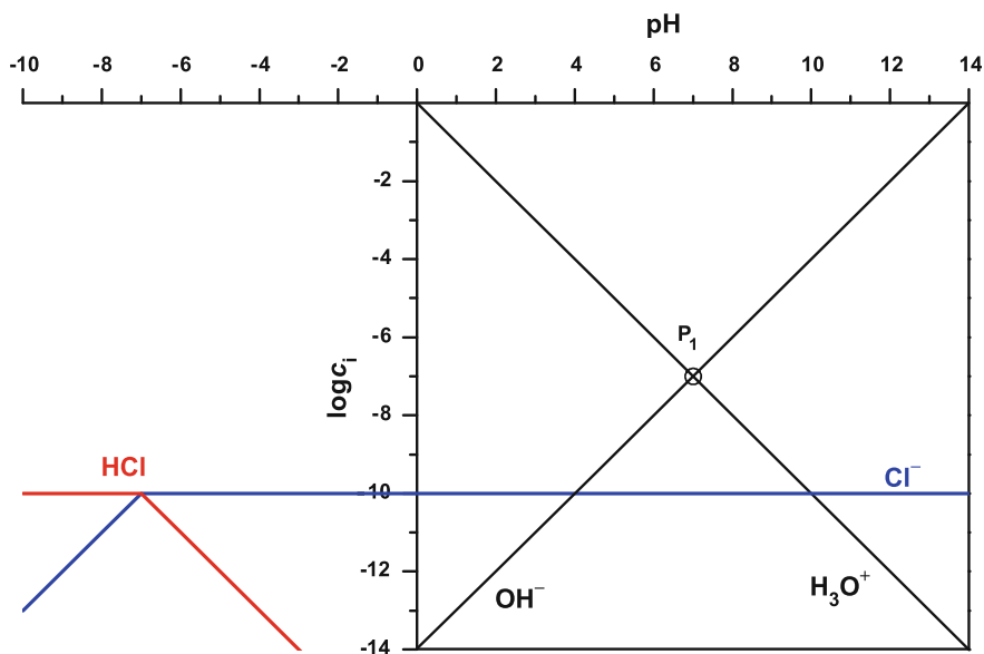
Fig. 34 pH- \log c_i diagram of a hydrochloric acid ( pK_a = -7 ) at 10^{-10} \text{ mol L}^{-1} concentration. The range for \text{pH} < 0 is only shown for didactic reasons. Normally this is not done
