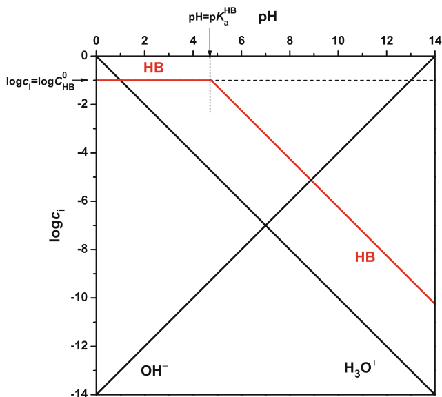
Fig. 13 Plotting the two asymptotes of HB with Eq. (33) for \text{pH} < \text{p}K_a and Eq. (34) for \text{pH} > \text{p}K_a . Example: acetic acid with C_{\text{HB}}^{\text{O}} = 0.1 \text{ mol L}^{-1} and \text{p}K_a = 4.75
