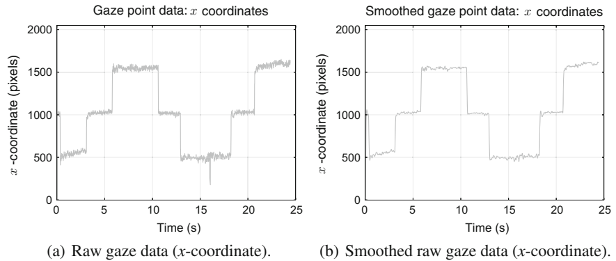
Fig. 14.1 Example 1D raw gaze x -coordinate data captured over a calibration validation grid: b Shows the effect of applying the Butterworth filter to the unfiltered data shown in (a) Notice in particular the removal of a downward spike at about the 16 s mark
