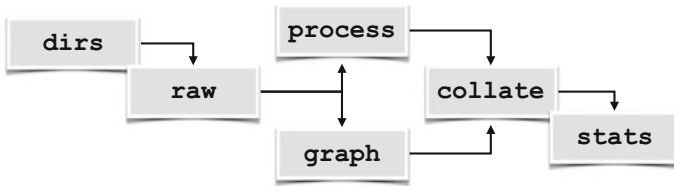
Fig. 15.1 The gaze analytics pipeline
