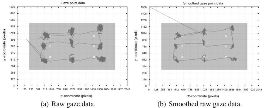
Fig. 14.2 Example 2D raw gaze data captured over a calibration validation grid: b Shows the effect of applying the Butterworth filter to the unfiltered data shown in (a) . Notice in particular the smoother path curves and reduced data. This effect is especially pleasing in real-time applications as the real-time gaze point appears to move more smoothly to the user without jitter that has been smoothed out by the filter. The long streak of points emanating from upper-left is the result of the Butterworth filter's initially empty history buffer, i.e., the filter needs to build up a history of data points to function properly
