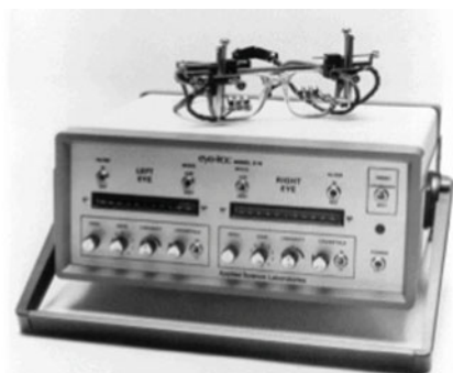
(b) Example of infra-red limbus tracker apparatus. Courtesy of Applied Science Laboratories (ASL), Bedford, MA < http://www.a-s-l.com >. Reproduced with permission.
