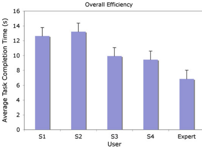
Fig. 19.7 Mean completion times of all users and expert (with SE whiskers)
