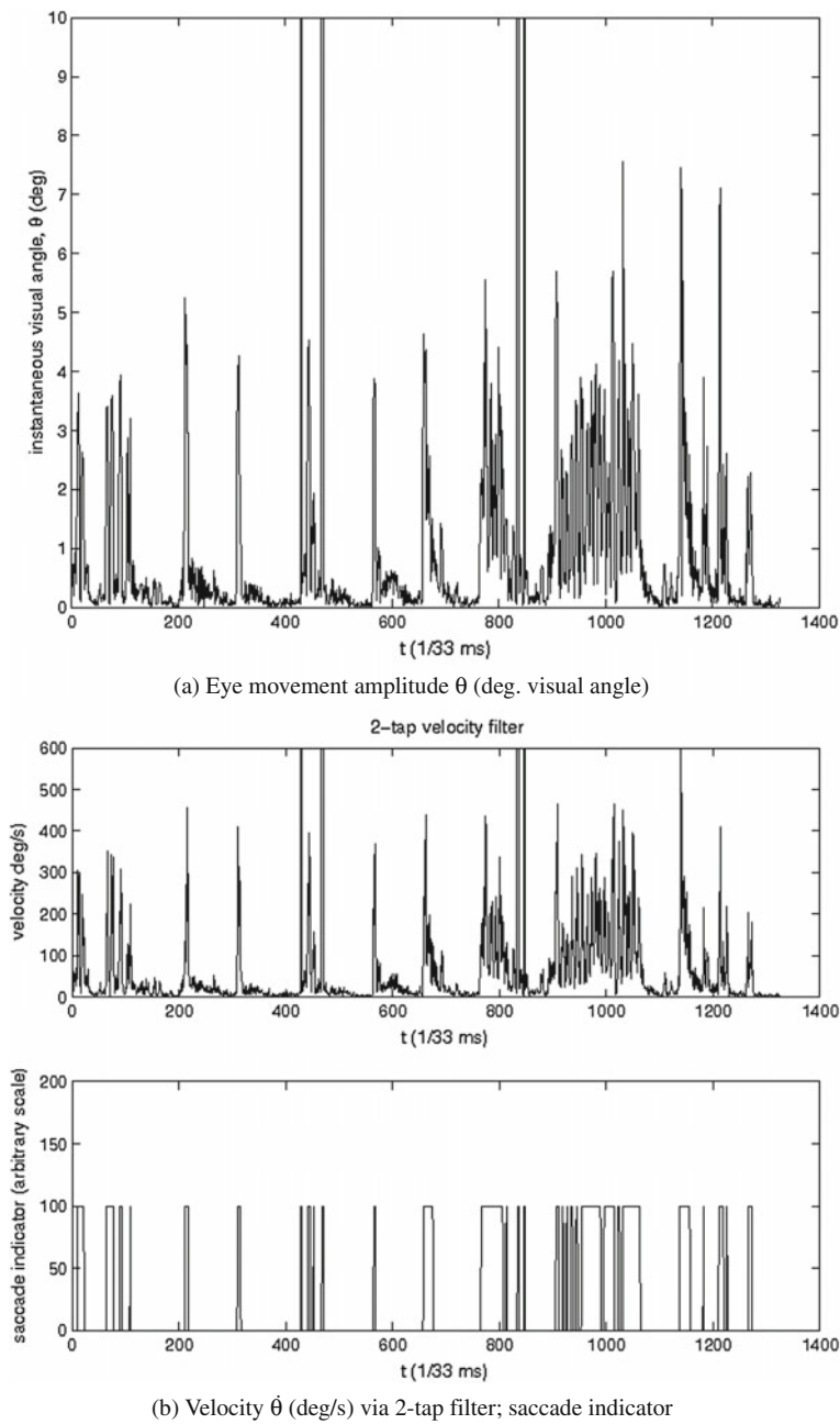
Fig. 13.9 Eye movement signal and filter responses
