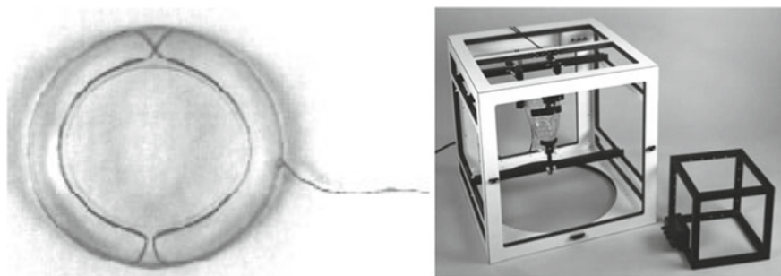
Fig. 5.2 Example of search coil embedded in contact lens and electromagnetic field frames for search coil eye movement measurement. Courtesy of Skalar Medical, Delft, The Netherlands ( http://www.skalar.nl ). Reproduced with permission
