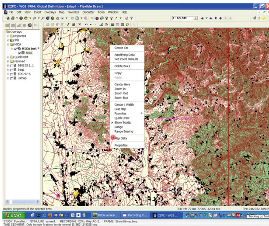
Fig. 19.8 Example of problematic Properties dialog selection. After two unsuccessful attempts, the user has finally right-clicked on the narrow box outline (at top left of the popup menu)
