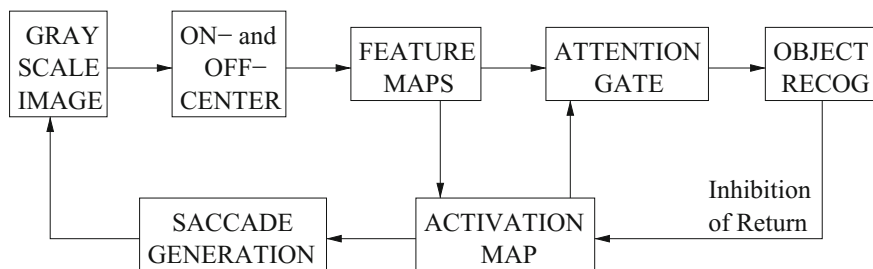
Fig. 21.5 Architecture of Guided Search 3.0. Adapted from Wolfe and Gancarz (1996) with permission © 1996 Kluwer Academic/Plenum Press
