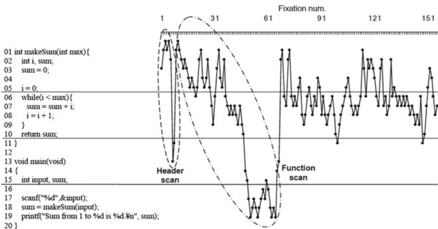
Fig. 24.1 Scanning behavior during program debugging. From Uwano et al. (2006)   2006 ACM, Inc. Reprinted by permission
