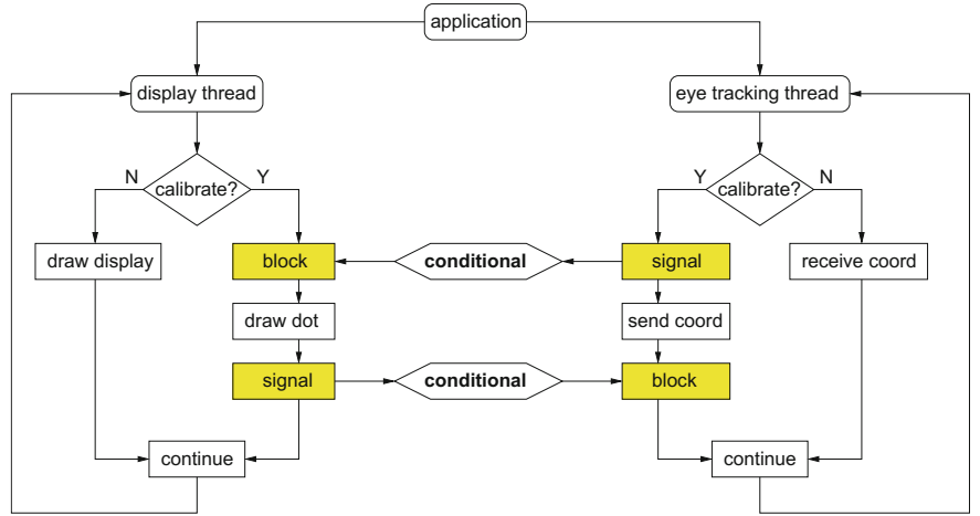
Fig. 11.2 Tobii concurrent process layout
