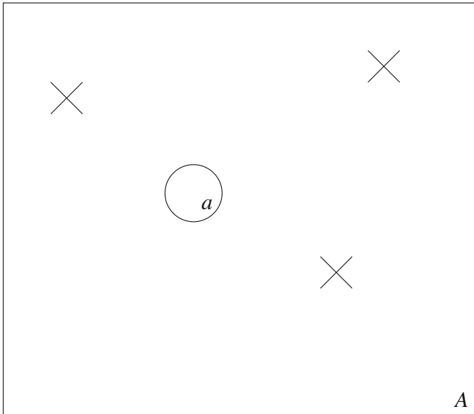
Fig. 22.3 Model of visual search area, visual lobe, and targets
