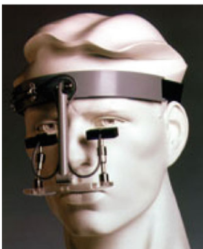
(c) Another example of infra-red limbus tracker apparatus, as worn by subject. Courtesy of Microguide, Downers Grove, IL < http://www.eyemove.com >. Reproduced with permission.
