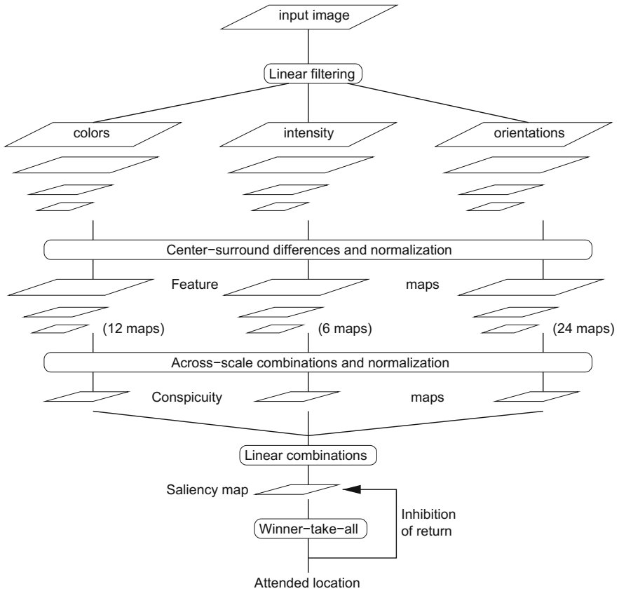
Fig. 21.6 Architecture of Itti et al.'s visual attention system. Adapted from Itti et al. with permission © 1998 IEEE
