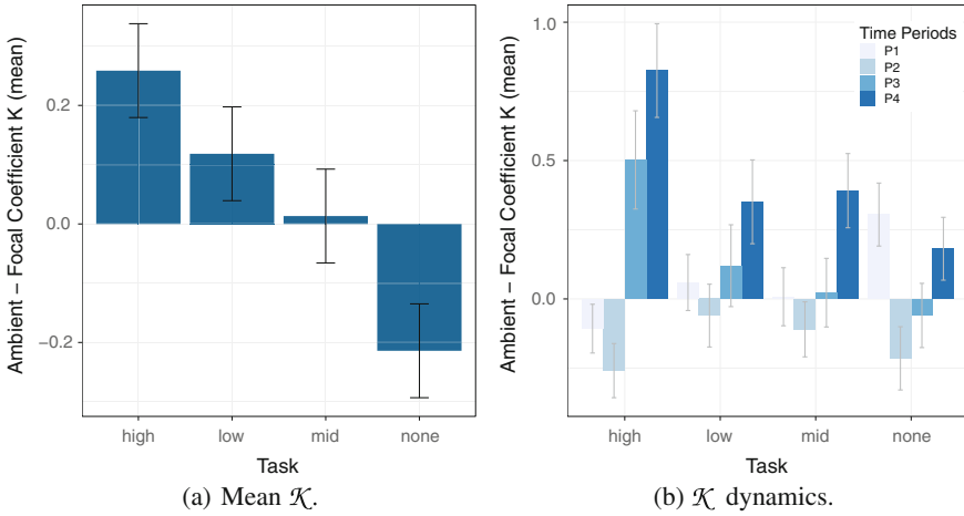
Fig. 15.6 Analysis of mean \mathcal{K} , \mathcal{K} dynamics, and transition entropy ( 2 \times 3 AOI grid)
