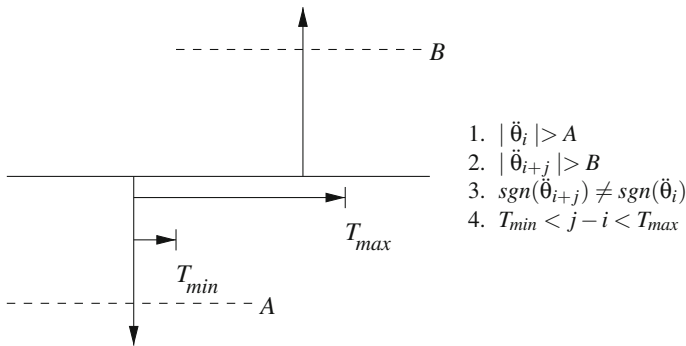
Fig. 13.8 Acceleration thresholding
