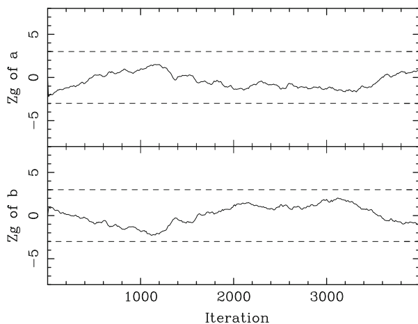
Fig. 16.6 Geweke Z scores with segment A and segment B, respectively, 20 and 40 % of the total chain length. The results correspond to the chain run with a proposal width of 10. The Z scores are calculated by using only every other 10-th iteration
