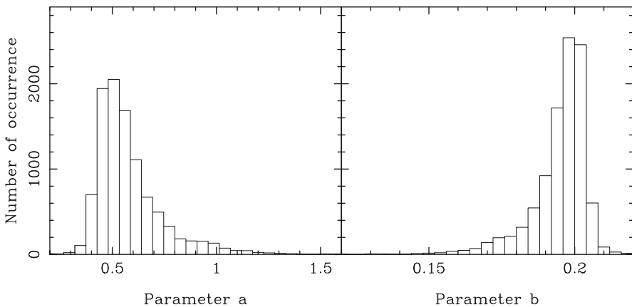
Fig. 14.3 Monte Carlo bootstrap method applied to the data from Hubble’s experiment. (Left) Sample distribution of parameter a , with a median of a = 0.54 and a 68 % central range of 0.45–0.70. (Right) Distribution of b , with median b = 0.197 and a central range of 0.188–0.202. The best-fit values of the original dataset Z were found to be a = 0.55 and b = 0.197 (see page 159)
