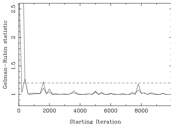
Fig. 16.7 Gelman–Rubin statistic \hat{R} calculated from m = 2 chains with the same distributions as in Fig. 16.3, one starting at a = 12 , b = 6 , and the other at a = 300 and b = 300 . The chain rapidly converges to its stationary distribution, and appears to forget about the starting point after approximately 500 iterations. The values of \hat{R} were calculated in segments of length b = 200 , starting at iteration i = 0
