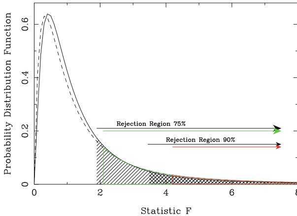
Fig. 7.3 Solid curve is the F distribution with \nu_1 = 5 , \nu_2 = 5 degrees of freedom; the hatched area is the 75% rejection region, and the cross-hatched area is the 90% rejection region. For comparison, the F distribution with \nu_1 = 4 , \nu_2 = 4 degrees of freedom is shown as the dashed line , and the two rejection regions are outlined in green and red , respectively. The rejection region for the F distribution with \nu_1 = 4 , \nu_2 = 4 degrees of freedom is shifted to higher values, relative to that with \nu_1 = 5 , \nu_2 = 5 degrees of freedom, because of its heavier tail
