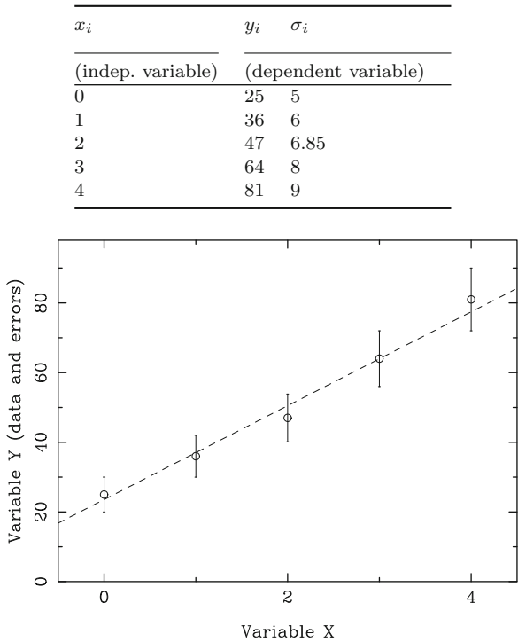
Fig. 10.2 Best-fit linear model ( dashed line ) to the data of Table 10.1. The \chi_{min} = 0.53 indicates a very good fit which cannot be rejected at any reasonable confidence level
