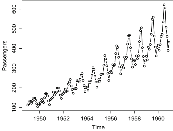
Fig. 12.2. Time series plot of monthly totals of air passengers (in thousands).
