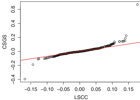
Fig. 6.2. QQ plot of returns on two stocks in the midcapD.ts data set. The reference line goes through the first and third quartiles.
