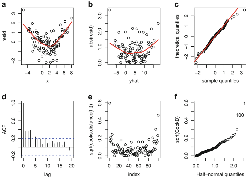
Fig. 10.10. Residual plots and diagnostics for regression of Y on X in Problem 1. The residuals are r student values. (a) Plot of residuals versus x . (b) Plot of absolute residuals versus fitted values. (c) Normal Q-Q plot of residuals. (d) ACF plot of residuals. (e) Plot of the square root of Cook's D versus index (= observation number). (f) Half-normal plot of square root of Cook's D .
