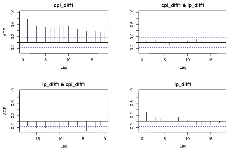
Fig. 13.13. Sample ACF for (\Delta cpi, \Delta ip)' . The marginal sample ACF for \Delta cpi and \Delta ip are shown in the first and second diagonal panels, respectively; the sample CCF for \Delta cpi and \Delta ip has been split between the top right and bottom left panels by positive and negative lags, respectively.
