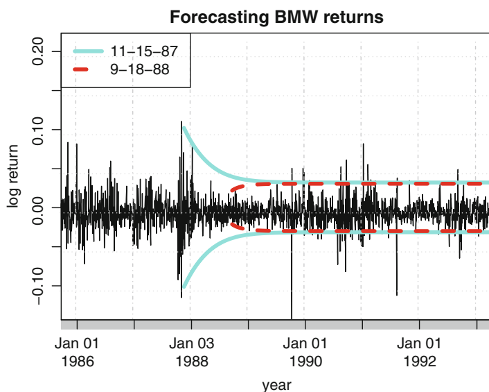
Fig. 14.10. Prediction limits for forecasting daily BMW stock log returns from two different time origins.
