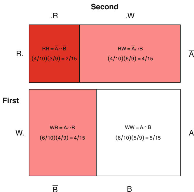
Fig. 3.1 Mosaic plot corresponding to Table 3.1. The area of each panel is equal to the probability of the event identified in that panel. The bottom row representing the event A = "W \text{ is selected first}" consists of the two panels WR and WW . The bottom row has height .6 = P(A) . The right-hand column represents the event B = "W \text{ is selected second}" consists of the two panels RW and WW . The event " B \cap A " is the white region WW in the lower right corner. The event WW has height .6 and width 5/9 , hence area .6 \times 5/9 = 1/3 . The event B | A is also the white area WW , but now thought of as the proportion of the A area that is also B . The probability of B | A is the ratio of the area of B | A to the A area (1/3)/.6 = 5/9 . The event B | \bar{A} is the pink region RW in the upper right corner. The probability of B | \bar{A} is the ratio of the pink area RW to the \bar{A} area (4/15)/.4 = 2/3 . The event \bar{B} \cap \bar{A} is the red region RR in the upper left corner. The event RR has height .4 and width 3/9 , hence area .4 \times 3/9 = 2/15 .
