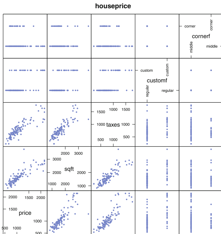
Fig. 9.3 House-price data. The discreteness of variables custom and corner decreases the informativeness of this splom, particularly the panel for this pair of variables. Figure 9.4 is a preferred splom presentation of these data.
