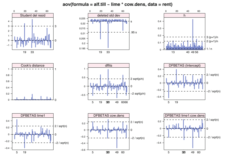
Fig. 11.6 Diagnostics from ANCOVA ( \text{rnt.alf/rnt.till} \sim \text{cow.dens} \mid \text{lime} ). The model is displayed in Table 11.4 and Figure 11.4. Each of the statistics in these panels is discussed in Section 11.3 and shown enlarged in Figures 11.12–11.17. To work around the problem that identification in the graph's x-axis of noteworthy cases often suffers from overprinting, the plot.case function returns and prints a list of noteworthy cases. We show the list in Table 11.5.
