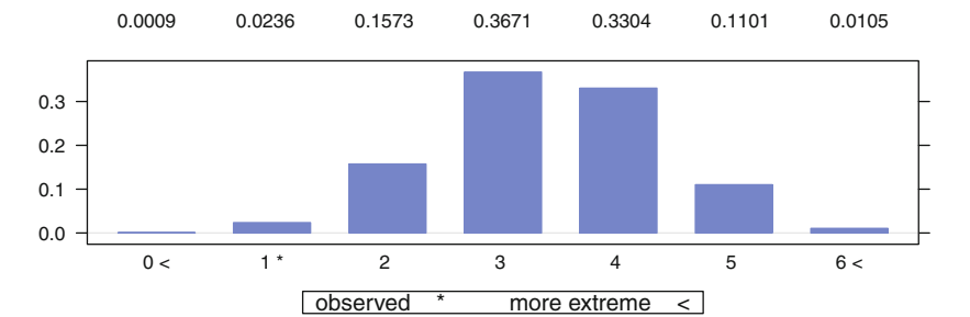
Fig. 15.6 Probabilities for all possible 2×2 tables with the same margins as the observed glasses table.
