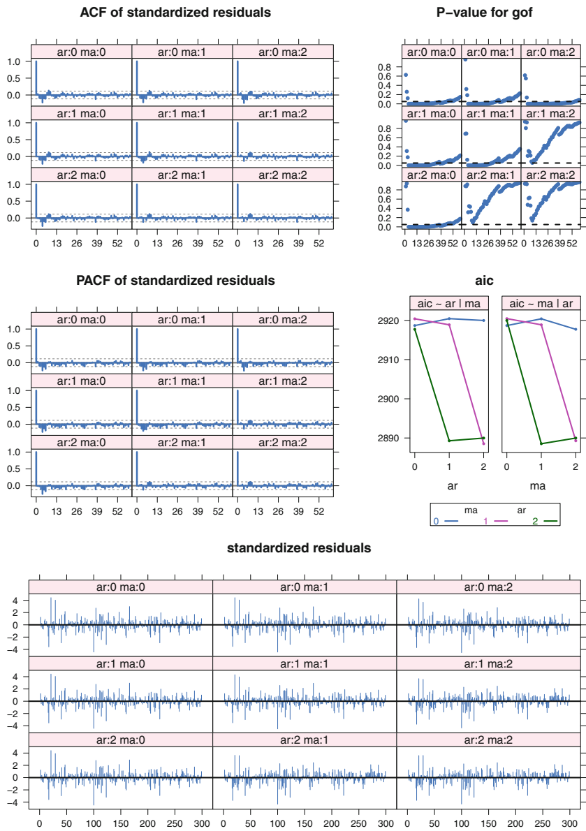
Fig. 18.19 Diagnostic plots for the set of models ARIMA(p,1,q) fit to the Product data by maximum likelihood. Each set of nine panels is systematically structured in a 3x3 array with rows indexed by the number of AR parameters p and columns by the number of MA parameters q . All nine panels in a set are scaled identically. The AIC has been plotted as a pair of interaction plots: AIC plotted against q using line types defined by p ; and AIC plotted against p , using line types defined by q .
