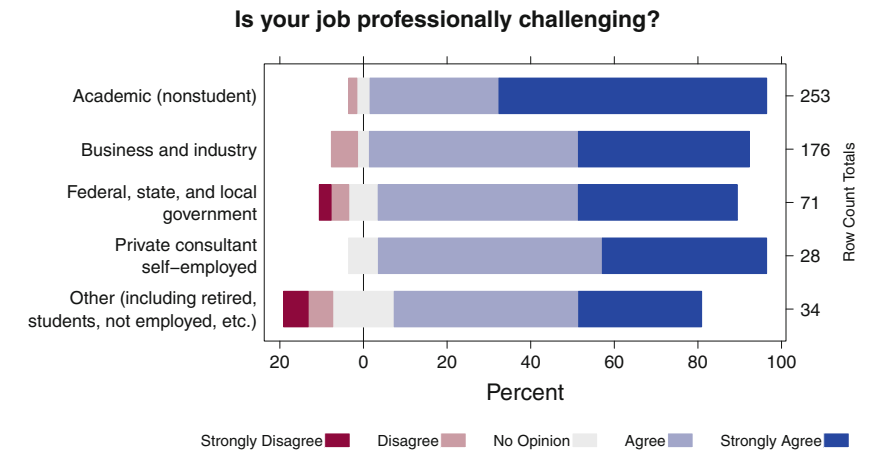
Fig. 15.16 In this variant of the plot, we display the row percents. We don't want to lose information about the uneven selection of respondents from the employment sectors so we display the counts as the right axis labels. Now we see that "Academic (nonstudent)" stands out as the largest percentage of dark blue on the graph.
