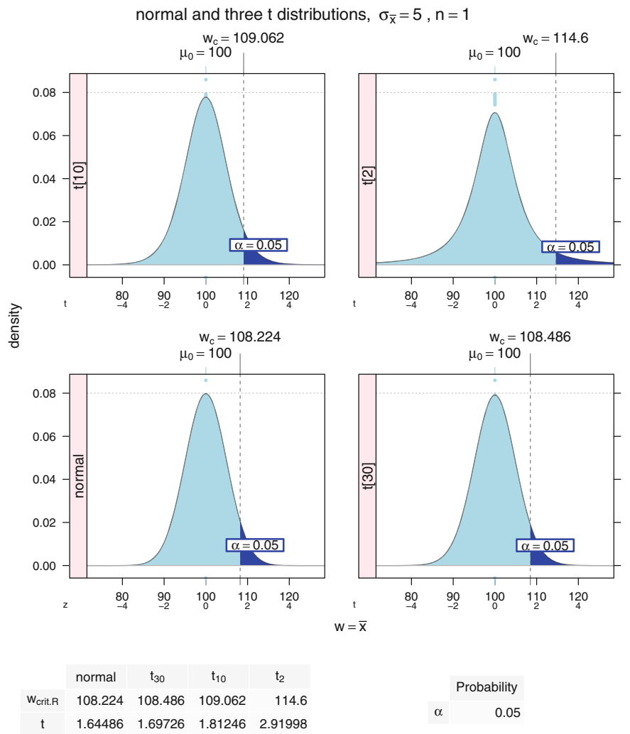
Fig. 3.14 These panels are similar to Figure 3.13, the first panel is identical to Figure 3.13. The remaining panels show t -distributions with 30 df, 10 df, and 2 df. Each panel has less area in the center and more area in the tails. Use the reference line at y = .08 to see the drop in central area, use the thickness of the tails at \bar{x} = 120 to see the increase in the probability in the tails. Use the location of the critical value w_c = \bar{x}_c on the graph and in the table below the graph to see that the critical value for the \alpha = .05 test is moving away from the null hypothesis value \mu_0 as the df gets larger.
