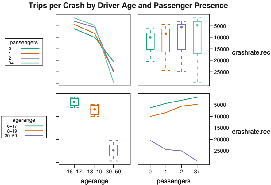
Fig. 14.18 Interaction plot of reciprocal crash data. The message is best seen in the bottom row. The boxplots in the lower-left panel show a difference in the small number of trips per crash for teens compared to the larger number of trips per crash for the adults. The lines in the lower-right panel show that adults increase the number of trips per crash with more passengers, meaning that they drive more safely with more passengers. But teens decrease the number of trips per crash with more passengers, meaning that they drive less safely with more passengers. This figure is identical to panel d in Figure 14.17.
