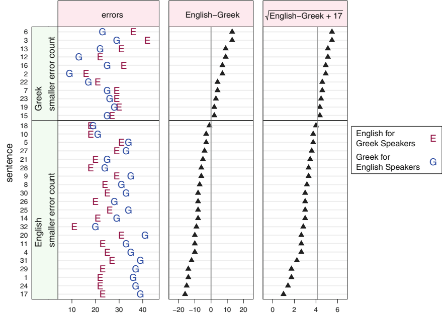
Fig. 5.7 Dotplot of language difficulty scores. The difficulty in learning each of 32 sentences written in English for Greek speakers (marked English) and written in Greek for English speakers (marked Greek) is noted. The panels are defined by placing the sentences in which the English version showed fewer errors on the bottom and the sentences in which the Greek version showed fewer errors on the top. The sentences have been ordered by the difference in the English and Greek error scores. The left panels show the observed error scores. The center panels show the differences, English–Greek, of the error scores. The right panels show the square root transformed differences, \sqrt{\text{English} - \text{Greek} + 17} . The t -tests in Table 5.8 will be based on the differences and the transformed differences.
