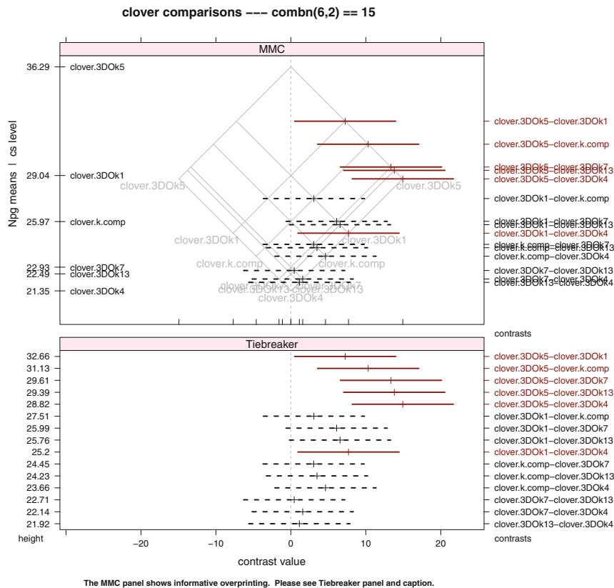
Fig. 12.14 MMC plot and Tiebreaker plot of Tukey simple effect contrasts for comb="clover" data. It is visually quite clear that the strain 3D0k5 differs from the rest (very strongly for the bottom three strains and less so for the middle two strains.) There is also one marginally significant contrast between the second largest mean and the smallest mean. We illustrate this observation in Figure 12.15 with an appropriately chosen set of orthogonal contrasts. The Tiebreaker plot in the bottom panel is imperative for this example. The means at many of the levels of cs are very close and therefore their labels are overprinted. The Tiebreaker plot shows the contrasts equally spaced along the y -axis and in the same sequence as the top panel.
