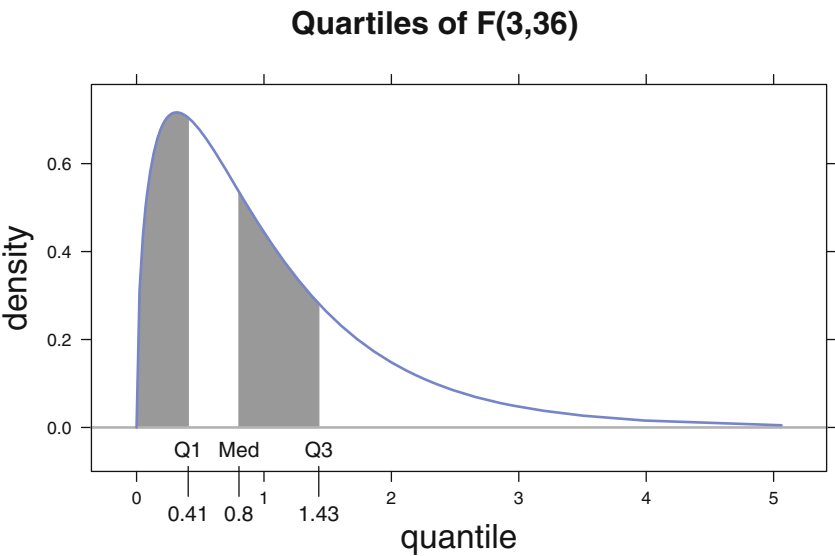
Fig. 3.6 Illustration of median and quartiles for a continuous distribution.
