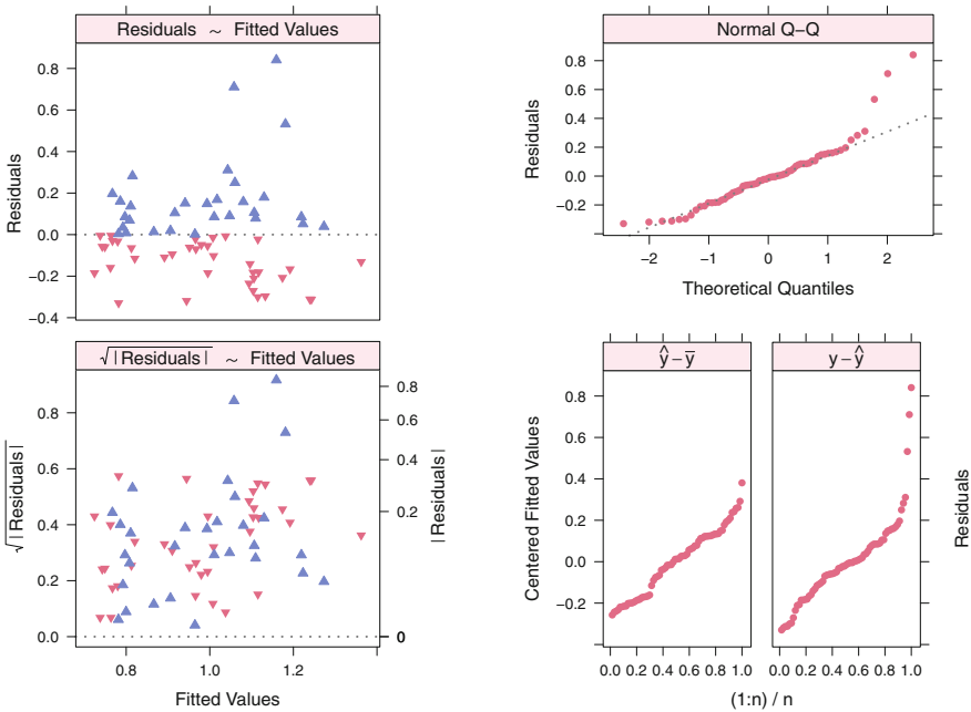
Fig. 11.5 Residuals from ANCOVA (\text{rnt.alf/rnt.till}) \sim \text{cow.dens} \mid \text{lime} . See Table 11.4 and Figure 11.4. The structure of the panels in this figure is discussed in Section 8.4. The figure itself is similar to Figure 8.6.
