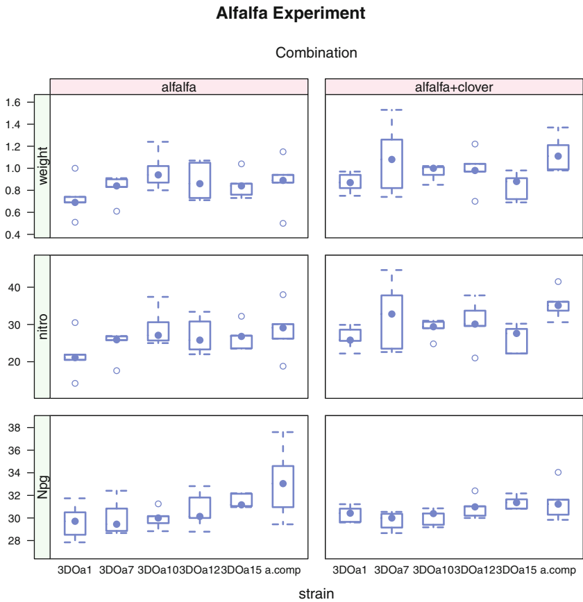
Fig. 12.7 Boxplot of alfalfa data. The Npg response variable has the least variability. We shall continue our analysis with Npg.
