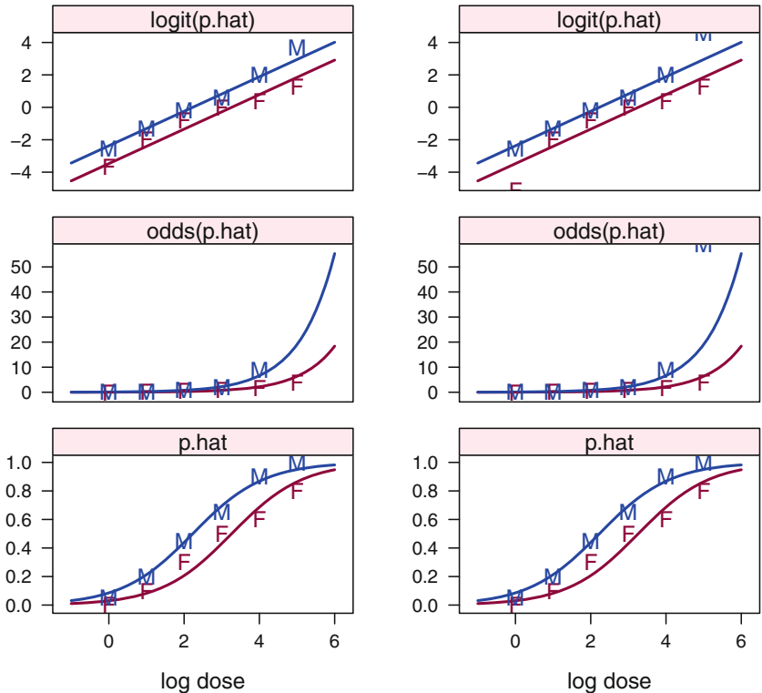
Fig. 17.9 Predicted probabilities of kill, and the odds and logit=log(odds), as a function of log(dose). A constant difference in the logit scale, seen as parallel lines in the logit ~ log.dose panel, corresponds to a constant ratio in the odds. The logit scale plot of this example, with one continuous covariate and one factor, is analogous to the analysis of covariance for continuous response and normally distributed error term as seen in Figure 10.8. The panels on the left for odds and logit have missing symbols where the transformation created infinite values ( \text{odds}(1) = \infty , \text{logit}(0) = -\infty , \text{logit}(1) = \infty ). In the panels on the right we placed partial symbols on the edge of the panel to indicate that there is an observation and that it is off the scale. The p.hat ~ log.dose is the same on both sides and is the same as Figure 17.8.
