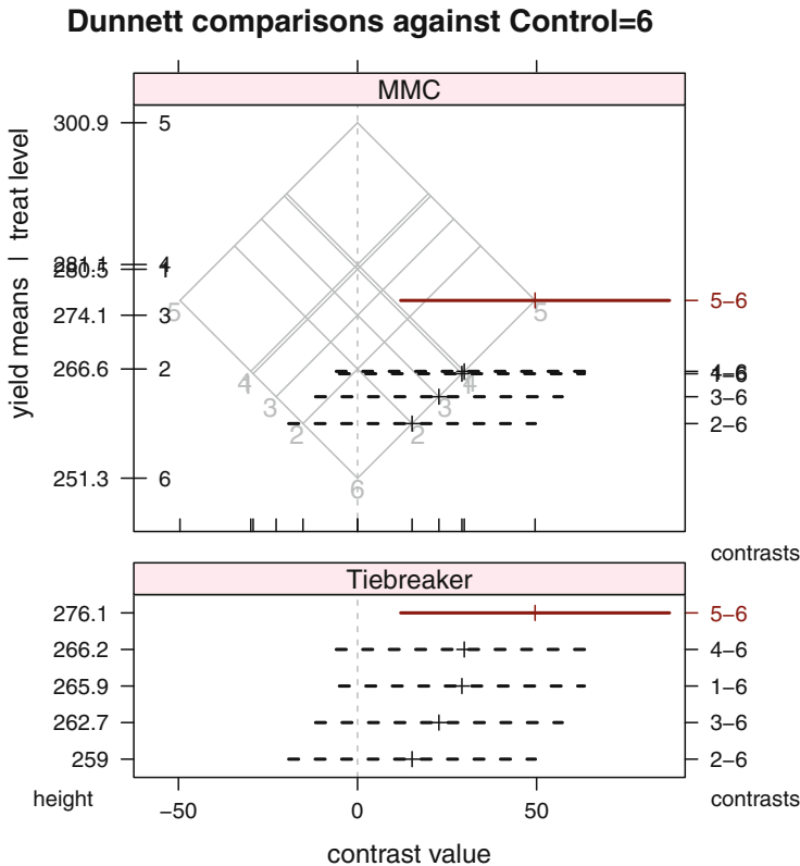
Fig. 14.9 Multiple comparisons of Treatments for Model 5 (yield ~ block + pre + treat) by Dunnett’s method. The comparison of treatment 5 with the control treatment 6 is the only significant comparison. The means for treatments 1 and 4 are very close; therefore the contrasts 4–6 and 1–6 are almost collinear in the MMC panel. We need the Tiebreaker panel to distinguish them.
