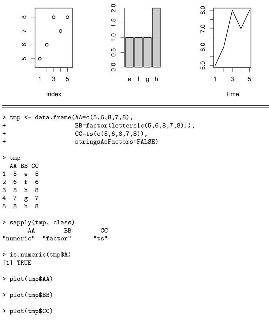
Fig. 6.7 The three columns of the data.frame tmp have three different classes. The plot function is sensitive to the class of its argument and draws a different style plot for each of these classes. The integer object (more generally numeric object) is plotted as a scatterplot with an index on the horizontal axis. The factor object is plotted as a bar chart with the level names on the horizontal axis. The time series object is plotted as a line graph with the time value on the horizontal axis.
