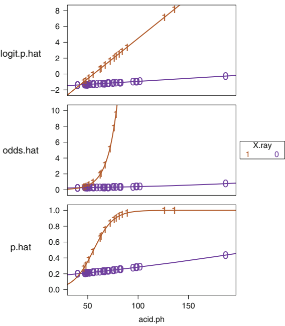
Fig. 17.18 Three scalings of fit to nodes ~ X.ray * acid.ph with the responses at both values of X.ray superposed on the same plot. The non-parallel lines in the logit.p.hat panel show the analogy with interaction in the ANCOVA setting. Two of the points in the odds.hat panel are beyond the limits we chose for the display. Their values in the odds.hat scale are 1256 and 3472.
