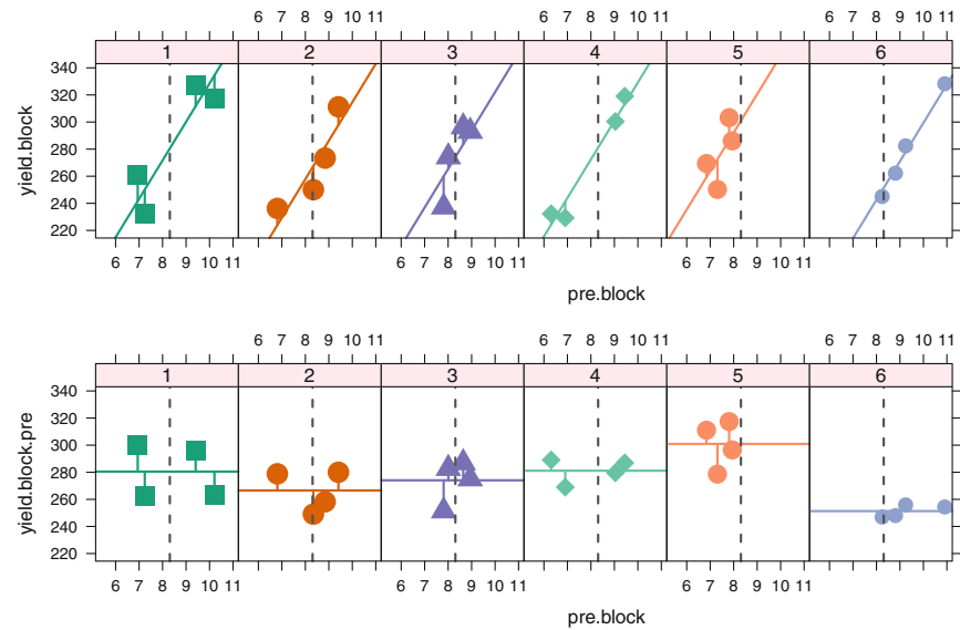
Fig. 14.8 Vertical difference between points and the parallel lines from rows 5 and 6 of Figure 14.6. It is easily seen in the bottom row that the control treatment 6 has a lower adjusted mean than the others. The light gray vertical reference line is at the mean of the adjusted pre values. The vertical reference line indicates the fulcrum of the vertical shifting of the points and parallel regression lines. The lengths of the residual lines from the points to the fitted line are identical in rows 5 and 6.
