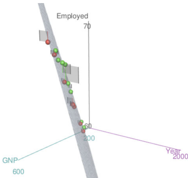
Fig. 9.8 The two X -variables, Year and GNP , are highly collinear. See model longley2.lm <- lm(Employed ~ Year + GNP, data=longley) in file HHscriptnames(9) . The response variable Employed is essentially on a straight line in the three-dimensional space of the figure. The specific plane displayed is almost arbitrary. Any plane that goes through the straight line of the observed points on the plane we see would work just as well.
