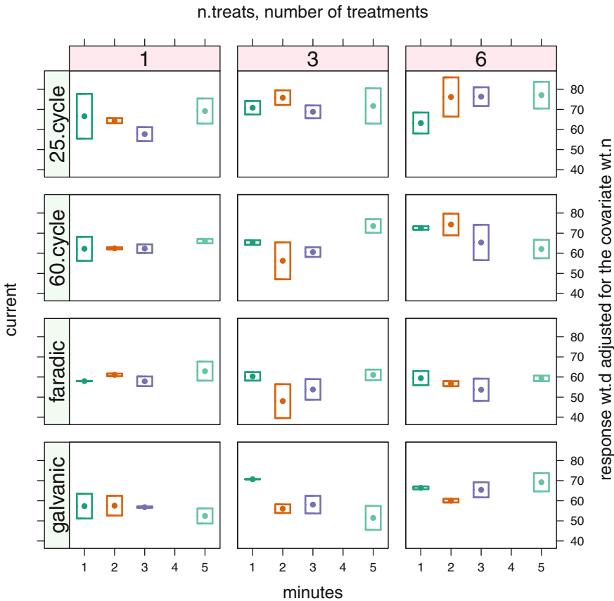
Fig. 13.3 Muscle data. Three-way interactions of all effects. One of the ( 3! = 6 ) possible orderings. The three-way interaction is not significant in this example. If there were a significant three-way interaction, the patterns in boxplots in adjacent rows and columns would not be the same. For example, we note a hint of a difference in the y.adj \sim minutes behavior across panels. It has a negative slope in the galvanic \sim 3 panel and a positive slope in the faradic \sim 3 panel, but a positive slope in the galvanic \sim 6 panel and a negative slope in the faradic \sim 6 panel. The ANOVA table tells us these differences in slope are not significant. These boxplots are all based on samples of size 2. Such boxplots are a well-defined but unc customary way to display such a sample.
