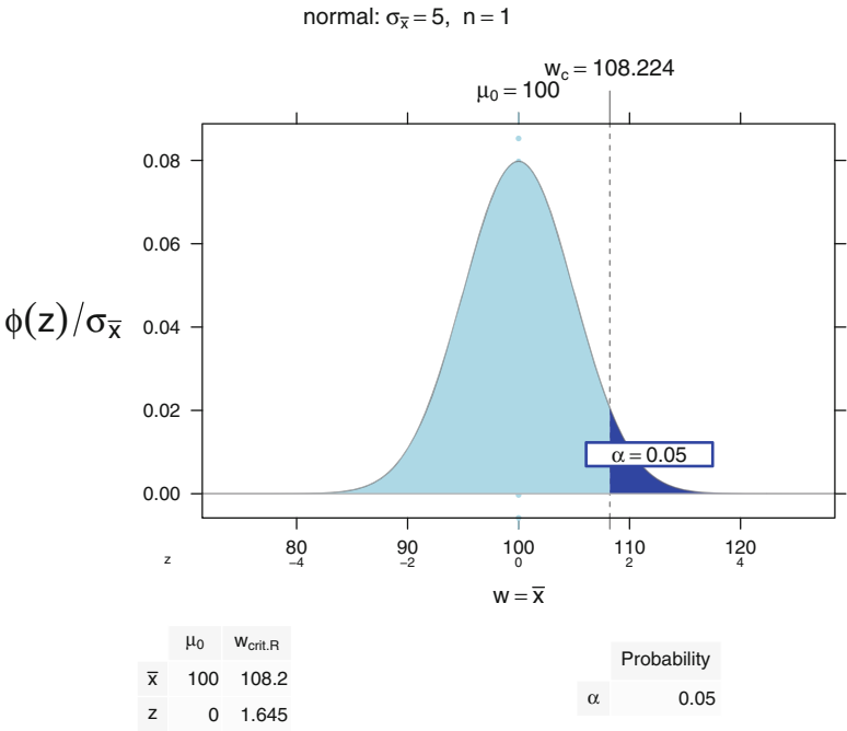
Fig. 3.13 A normal curve centered on the assumed true mean \mu = 100 . We assume \sigma = 5 and \alpha = .05 . The left lightly shaded area is .95 = P\left(z = (X - \mu)/\sigma \leq \Phi^{-1}(1 - \alpha) = 1.645\right) . The right darkly shaded area is \alpha = .05 = P\left(z = (X - \mu)/\sigma \geq \Phi^{-1}(1 - \alpha) = 1.645\right) . The plot shows both the \bar{x} scale and (in smaller font) the z scale. The table below the plot shows \mu_0 and the right critical value \bar{x}_{\text{crit.R}} in both scales. The critical value in the z scale is directly from the normal table.
