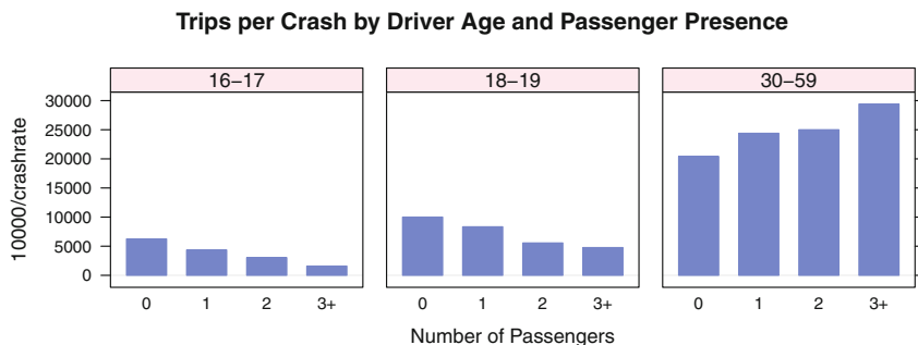
Fig. 14.19 Barplot of reciprocal crash data. The values displayed here are identical to the traces in the lower-right panel of Figure 14.18. Again we see that adults increase the number of trips per crash with more passengers, meaning that they drive more safely with more passengers. But teens decrease the number of trips per crash with more passengers, meaning that they drive less safely with more passengers.
