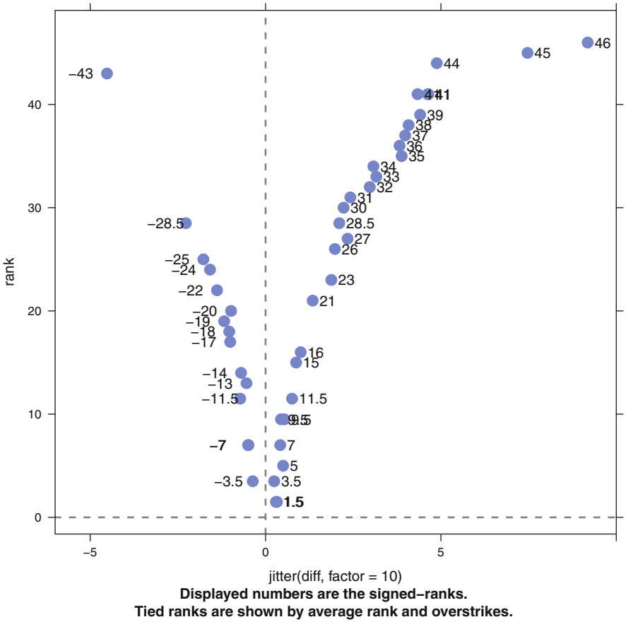
Fig. 16.3 The differences and ranks from Table 16.3 used in the Wilcoxon test of data(har1) . Observe that the positive differences between pre- and post-treatment angles tend to have larger magnitudes than the negative differences. The Wilcoxon test, which takes account of these magnitudes, has more power than the sign test, which ignores the magnitudes. The test statistic is the sum of the ranks for positive differences (the sum of the displayed numbers in the upper-right quadrant).
