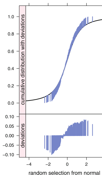
Fig. 5.17 Kolmogorov–Smirnov plots. Kolmogorov–Smirnov One-Sample Test. On the left we compare a random selection from the t distribution with 5 df to a null hypothesis distribution of t with 2 df. The ks.test in Table 5.12 shows a p -value of 0.2982 and does not reject the null. On the right we compare a random selection from the standard normal distribution to a null hypothesis distribution of t with 2 df. The ks.test in Table 5.12 shows a p -value of 0.003808 and rejects the null. The solid line in the top panels is the CDF for null distribution, in this example the t with 2 df. The deviation lines connect the observed y -values from the dataset under test to the hypothesized y -values from the null distribution. The deviation lines are magnified and centered in the bottom panels. The largest |vertical deviation| is the value of the K–S statistic in Table 5.12.
