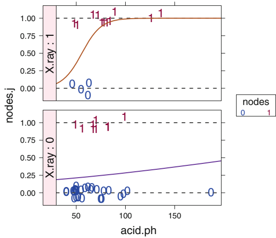
Fig. 17.17 Figure 17.13 plus fitted logistic curves for the interaction model glm(nodes ~ X.ray * acid.ph, data=lymph, family=binomial) .
