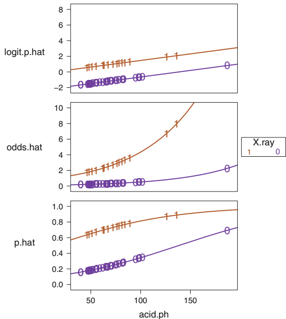
Fig. 17.16 Three scalings of fit to \text{nodes} \sim \text{acid.ph} \mid \text{X.ray} with the responses at both values of \text{X.ray} superposed on the same plot. The parallel lines in the \text{logit.p.hat} panel show the analogy with ANCOVA.
