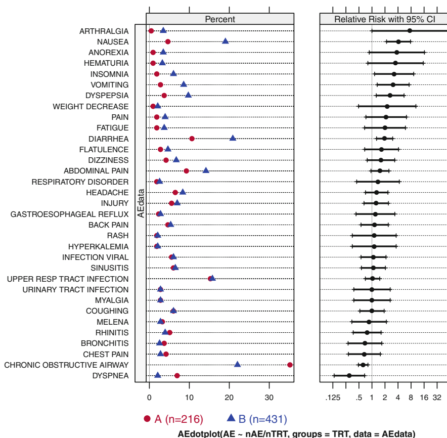
Fig. 15.13 Adverse Events dotplot for the clinical trial discussed in Amit et al. (2008). The left panel shows the observed percents of patients who reported each adverse event. The center panel shows the relative risk of Drug B relative to Drug A with 95% confidence intervals for a 2×2 table. By default, the AEs are ordered by relative risk so that events with the largest increases in risk for the active treatment are prominent at the top of the display.
