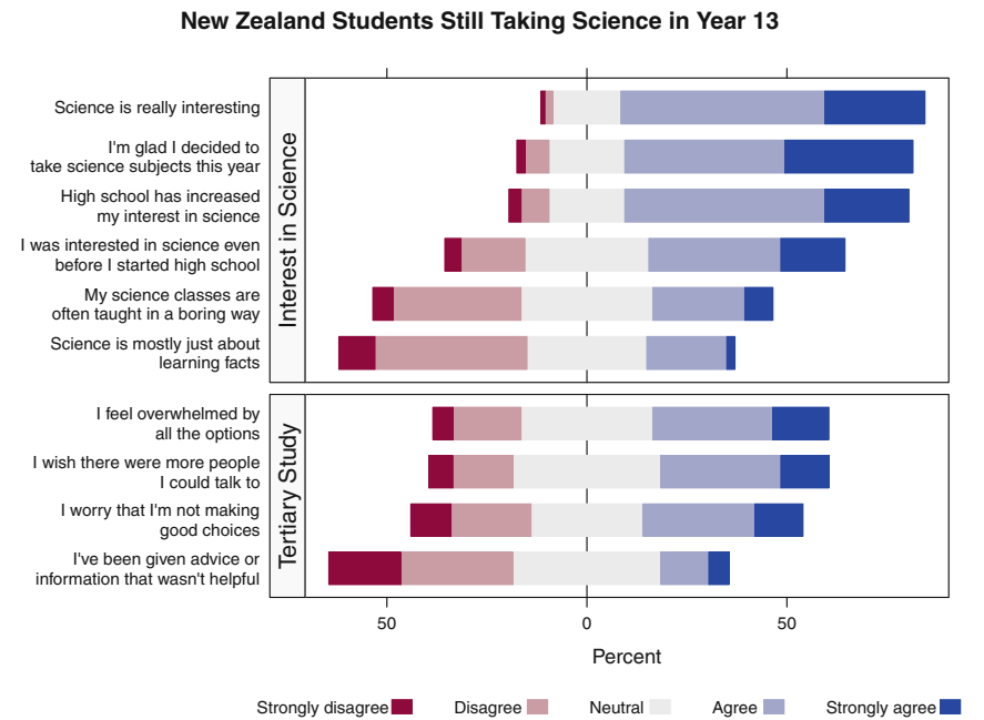
Fig. 15.18 Two sets of questions have been asked of all respondents. Each set is presented in its own panel.
