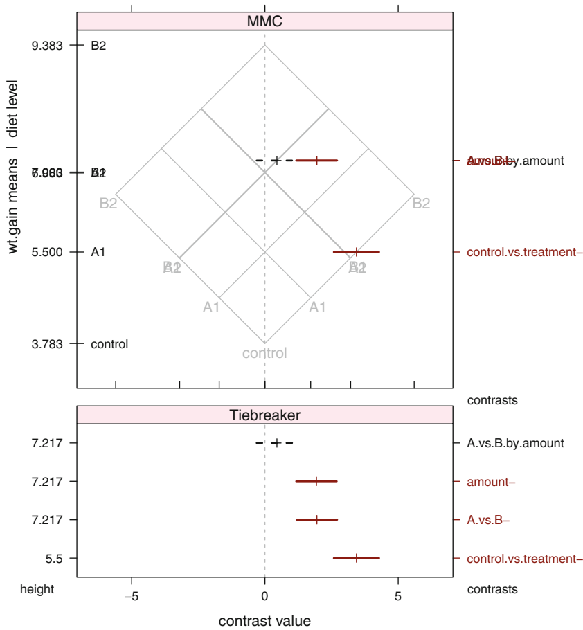
Fig. 7.6 MMC: Orthogonal basis set of contrasts for Turkey data. Overprinting of the confidence lines (for contrasts A . vs . B -, amount -, and A . vs . B . by . amount, in this example) and their labels in the right-axis labels of the MMC panel is a consequence of almost identical values for the group means in the left-axis labels (A2 and B1). The overprinting is resolved in the Tiebreaker panel, a standard multiple comparisons plot (without information on the group means) ordered to match the order of the MMC plot. The contrasts in these panels are the same contrasts that appear in Figure 7.4, but negative estimates there have been reversed here. During the reversal a “-” was appended to contrast names for which it was not possible to figure out how to reverse the contrast name.
