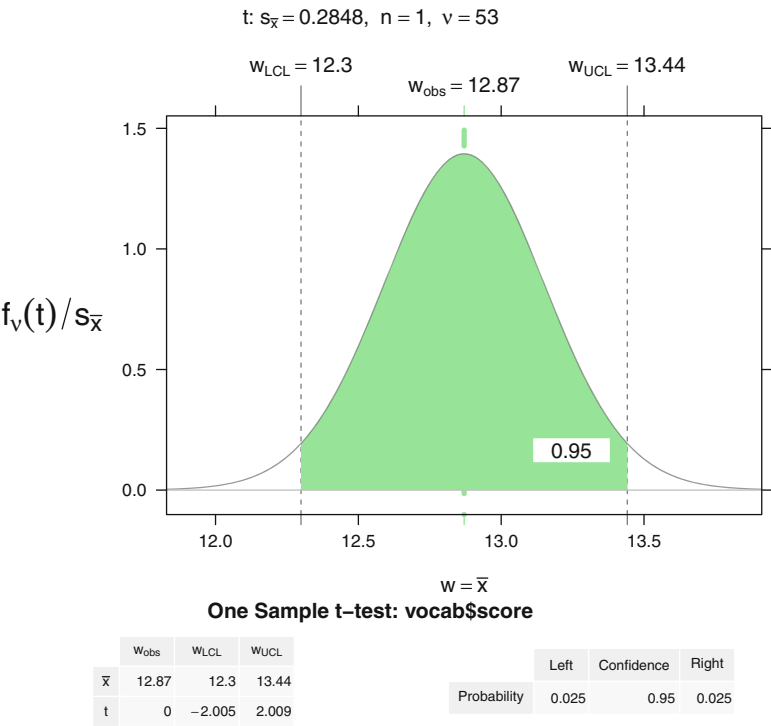
Fig. 5.4 t -test and t -based confidence interval of vocabulary scores.
