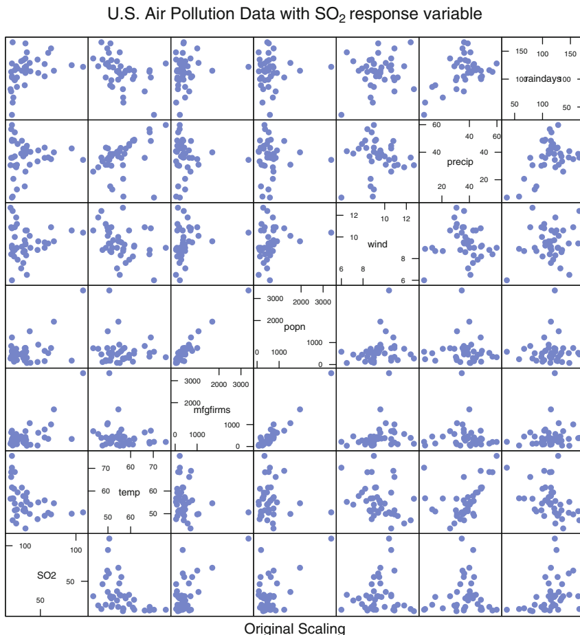
Fig. 9.11 Scatterplot matrices for air pollution data with the original scaling.
