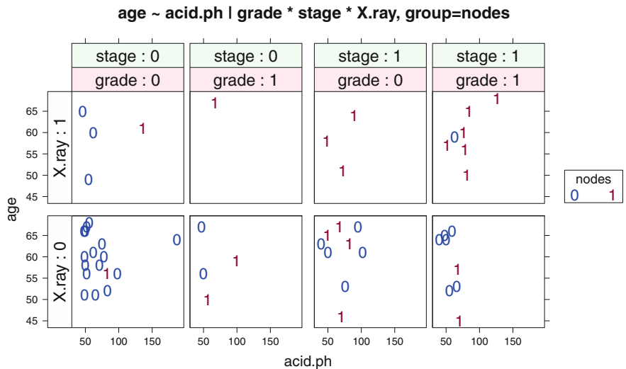
Fig. 17.10 Much of the relation between variables is visible in this set of panels conditioned on three factors, with the plotting symbol representing a fourth factor. The top row with X.ray=1 has a higher proportion of nodes=1 . The right two columns with stage=1 have a higher proportion of nodes=1 .
