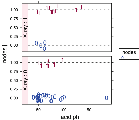
Fig. 17.13 xyplot(nodes.j ~ acid.ph | X.ray) . The observed nodes are jittered to break the ties. The dashed lines indicate the location of the actual 0 and 1 values.
