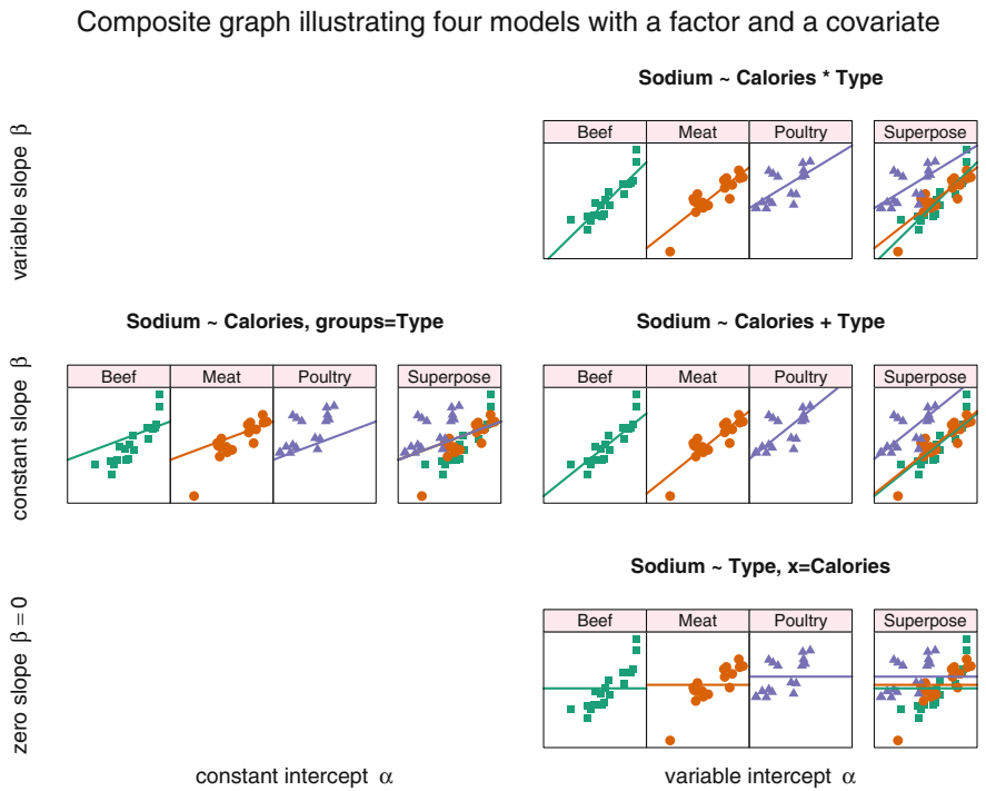
Fig. 10.12 Four models for the hot dog data, arranged in two columns corresponding to the two possibilities for the intercept in the model and three rows corresponding to the three possibilities for the slope in the model. The models are often described as
