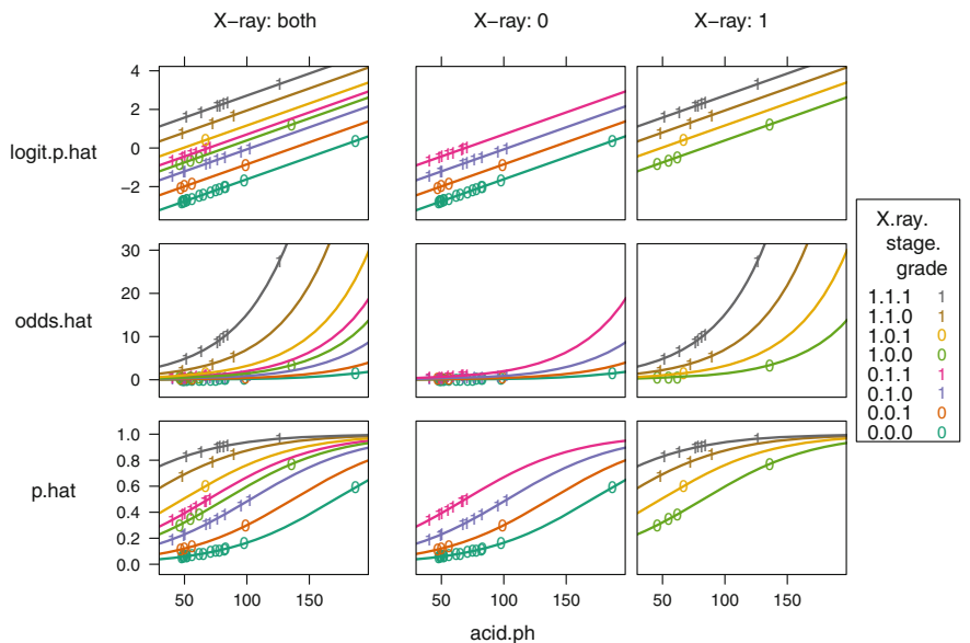
Fig. 17.12 Plot of \hat{p} , \text{odds}(\hat{p}) , \text{logit}(\hat{p}) for the model nodes \sim \text{acid.ph} \mid \text{X.ray} + \text{stage} + \text{grade} , with plotting symbol indicating stage and placed at the predicted values for the observed acid.ph. The left column shows the fit for both values of X.ray. The right columns are the same fitted values with the illustration conditioned on the value of X.ray. The panel in the p.hat row and the X-ray: both column shows the eight fitted lines from Figure 17.11.
