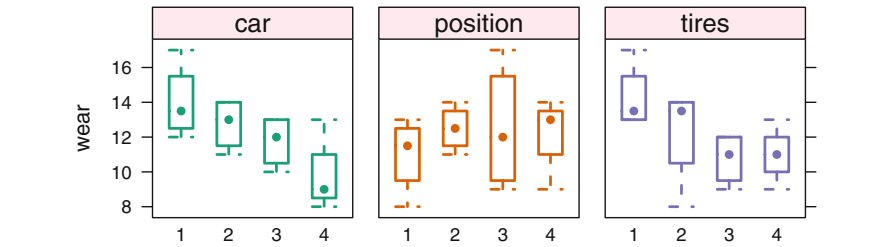
Fig. 13.6 Tires data. Boxplots of the response variables wear against the three factors.
