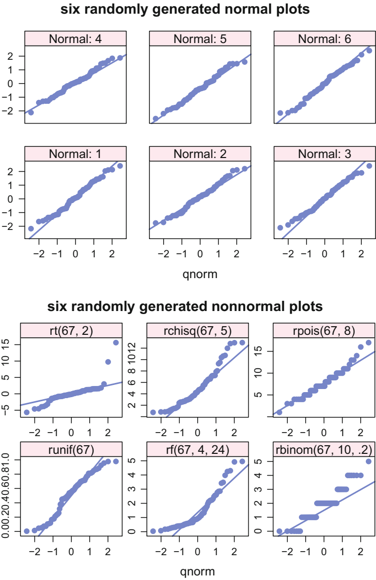
Fig. 11.10 Normal plot of six randomly generated normal variables and six randomly generated nonnormal variables. These plots are placed here to help you calibrate your eye to what normal and nonnormal distributions look like when plotted against the normal quantiles. t : long left and right tails as indicated by points below the diagonal on the left and above the diagonal on the right. Chi-square: short left and long right tails. Poisson: discrete appearance and long tail on the right. Uniform: short tails on left and right as indicated by points above the diagonal line on the left and below the diagonal line on the right. F : short tail on the left and long tail on the right. Binomial: discrete positions on the y-axis, with short tail on the left; this example with p = .2 is not symmetric and we see more points on the left.
