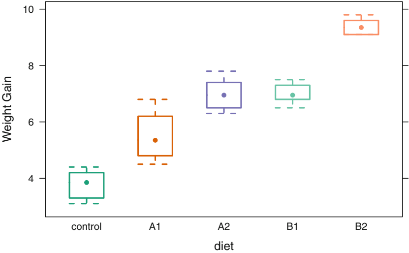
Fig. 6.5 Turkey Data: Boxplots of Weight Gain for each Diet
