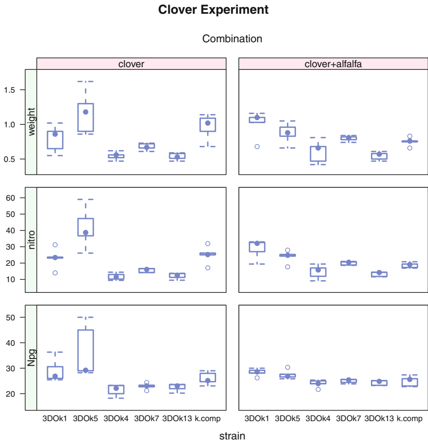
Fig. 12.8 Boxplot of clover data. The Npg response variable has the least variability. We shall continue our analysis with Npg . The large variability in the 3D0k5 strain is visible in all three response variables.
