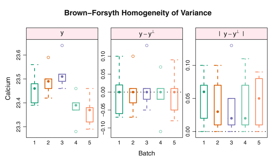
Fig. 6.3 Homogeneity of Variance plot for Batch. The left panel shows the data within each group. The center panel shows the same variabilities centered on the group medians ( y_{ij} - \bar{y}_j ). The right panel shows the boxplot of the absolute deviations from the median ( |y_{ij} - \bar{y}_j| ). The Brown–Forsyth test is an ordinary analysis of variance of these absolute deviations from the median. If the means of each group of the absolute deviations differ, then the test says the variances of the groups of original data differ.
