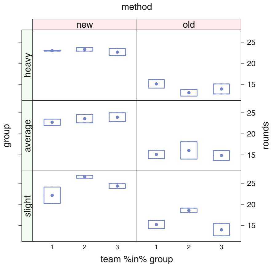
Fig. 13.12 Boxplot of gunload data. The response rounds is higher for the new method than the old method and does not appear to differ across the three physique groups. These findings are consistent with the small p -value for method and the large p -value for group in Table 13.13.
