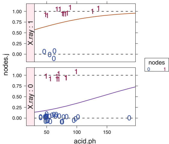
Fig. 17.15 Figure 17.13 plus fitted logistic curve for the simple model glm(nodes ~ X.ray + acid.ph, data=lymph, family=binomial) .
