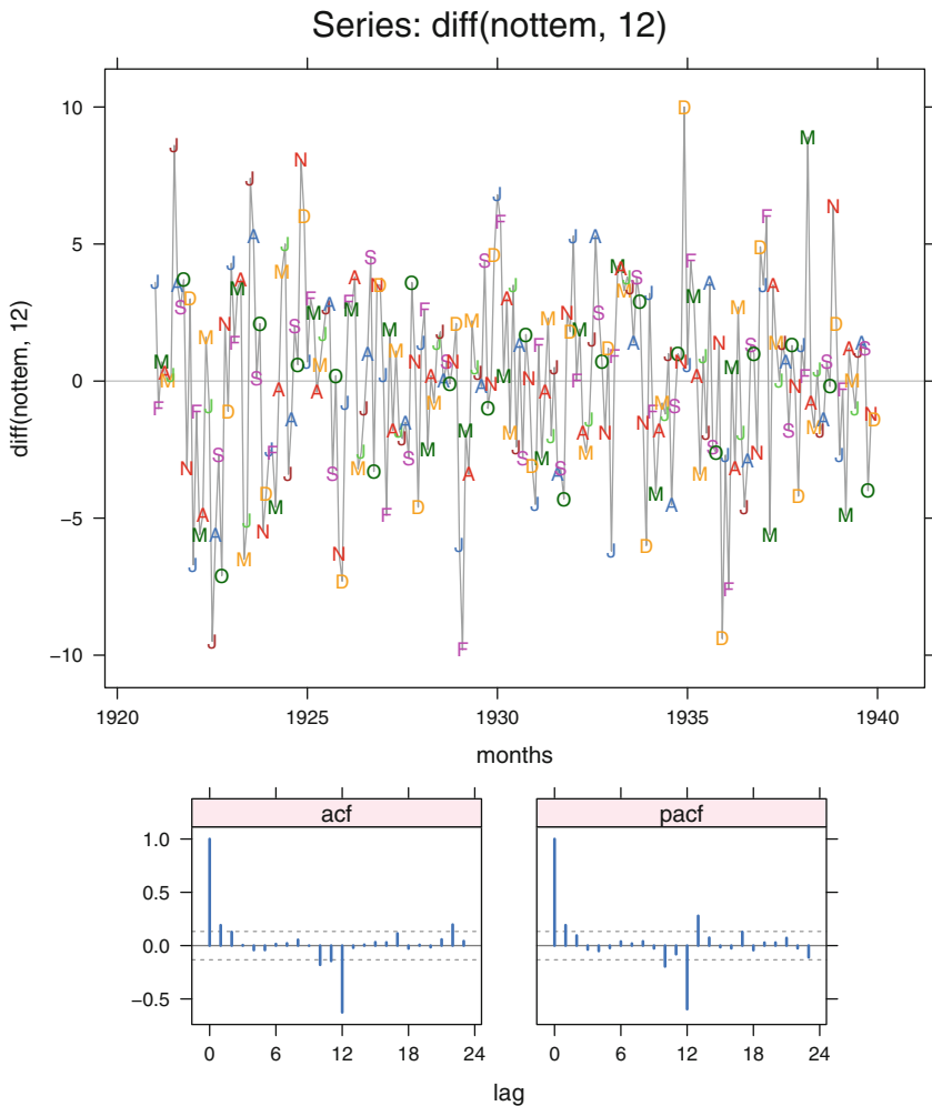
Fig. 18.21 Seasonal differences of mean monthly air temperature in degrees Fahrenheit from January 1920 to December 1939 at Nottingham.
