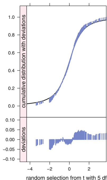
Fig. 5.17 Kolmogorov–Smirnov plots. Kolmogorov–Smirnov One-Sample Test. On the left we compare a random selection from the t distribution with 5 df to a null hypothesis distribution of t with 2 df. The ks.test in Table 5.12 shows a p -value of 0.2982 and does not reject the null. On the right we compare a random selection from the standard normal distribution to a null hypothesis distribution of t with 2 df. The ks.test in Table 5.12 shows a p -value of 0.003808 and rejects the null. The solid line in the top panels is the CDF for null distribution, in this example the t with 2 df. The deviation lines connect the observed y -values from the dataset under test to the hypothesized y -values from the null distribution. The deviation lines are magnified and centered in the bottom panels. The largest |vertical deviation| is the value of the K–S statistic in Table 5.12.
