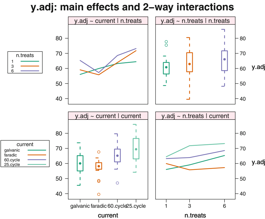
Fig. 13.2 Muscle data. Two-way interactions of significant main effects from the ANCOVA in Table 13.1. The adjusted response y.adj increases linearly with n.treats and differs according to the type of current used.
