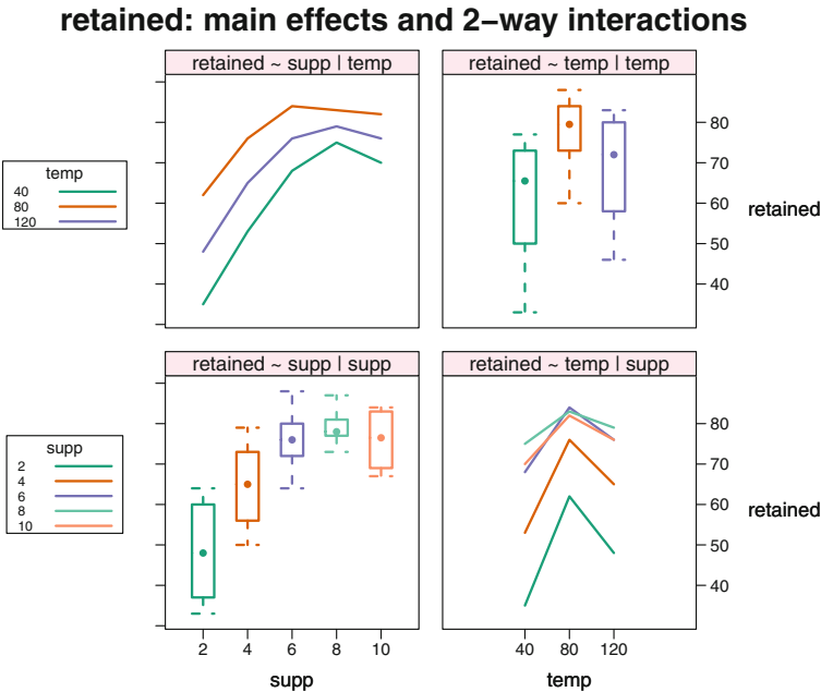
Fig. 12.17 Feed data interaction plots.
