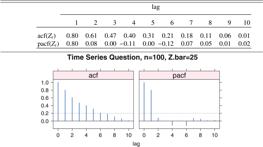
Fig. 18.26 ACF and PACF for Exercise 18.9, n = 100 and \bar{Z} = 25 . The same information is presented in both tabular and graphical form.
