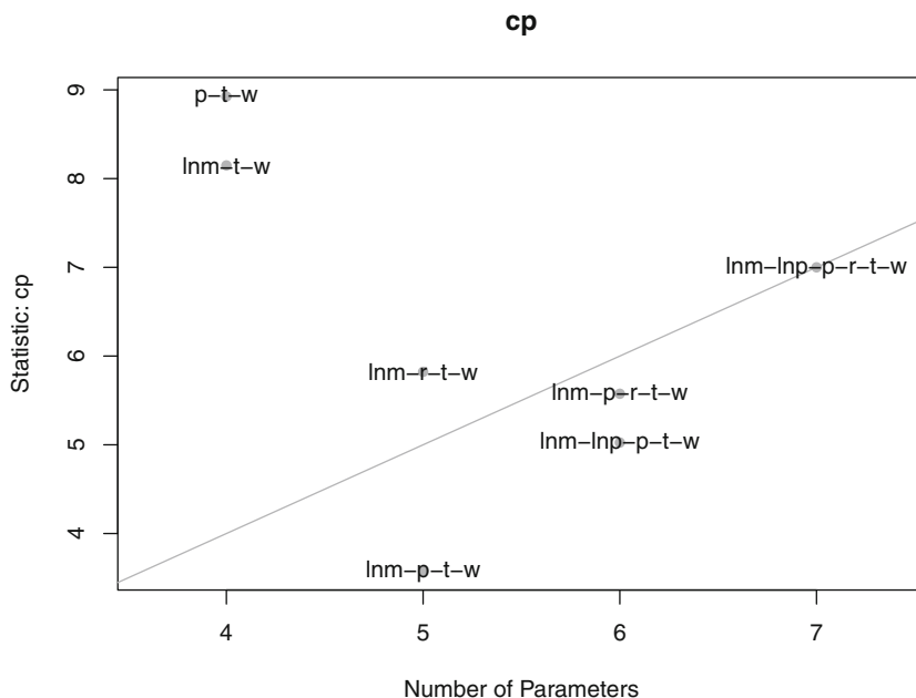
Fig. 9.13 C_p plot. Model “lnm-p-t-w” (lnmfg, precip, temp, wind) has the smallest C_p value and the largest R^2_{\text{adj}} . See also Table 9.14.
