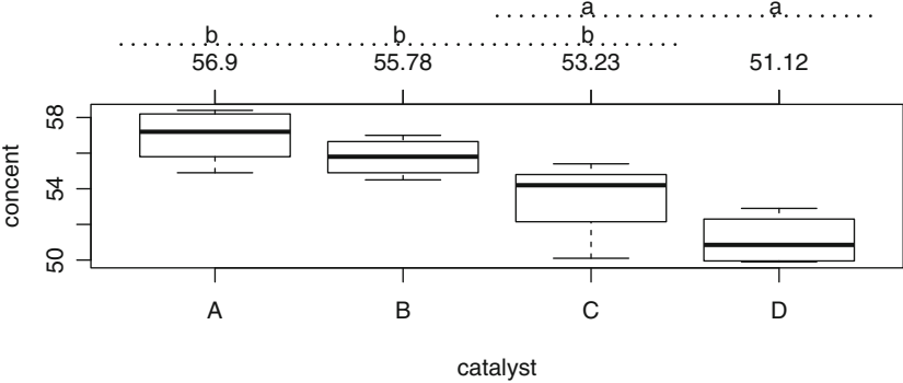
Fig. 7.8 This example is constructed from the cld function in the multcomp package. The function call plot(cld(catalystm.glm)) draws the boxplots and the letter values. We manually (by supplementary code) placed the numerical values of the means and the underlines connecting the letters.
