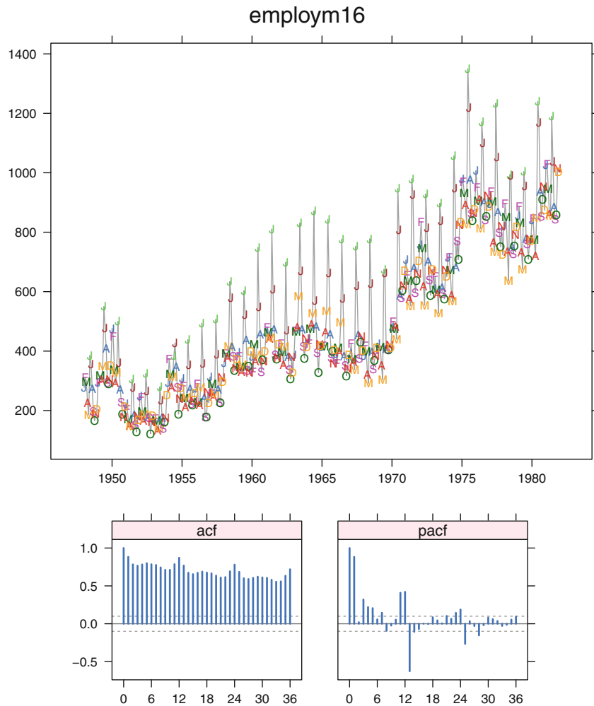
Fig. 18.29 United States of America Monthly Employment Figures for Males Aged 16–19 Years from 1948 to 1981, for use with Exercise 18.13.
