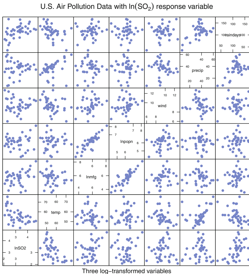
Fig. 9.12 Scatterplot matrices for air pollution data with improved symmetry after a log transformation of the three variables: \text{SO}_2 , \text{mfg} firms, \text{popn} .
