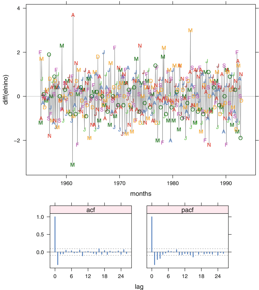
Fig. 18.2 Coordinated time series and ACF/PACF plots for the differenced elnino time series: \nabla y_t .
