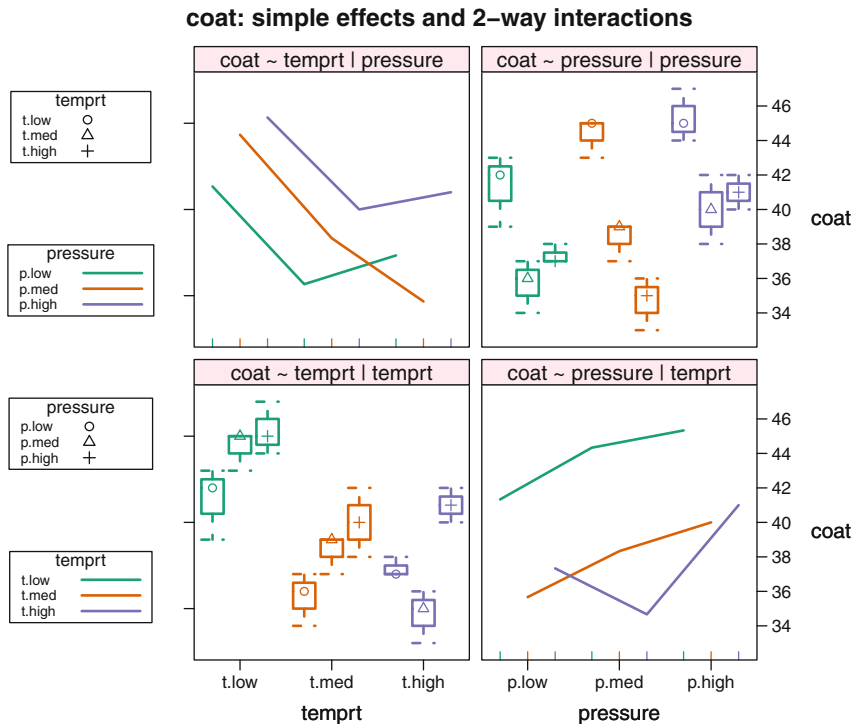
Fig. 13.9 Simple effects plot for filmcoat data. At medium pressure, mean coat is minimized at high temprt. No other firm conclusions can be drawn because many of the simultaneous confidence intervals in Figures 13.10 and 13.11 overlap zero. We saw in Section 13.3 that main effects are not defined in the presence of interaction. The simple effects plot here shows individual boxplots for each level of pressure conditioned on the level of temperature in the lower left panel. The plot shows individual boxplots for each level of temperature conditioned on the level of pressure in the upper right panel.
