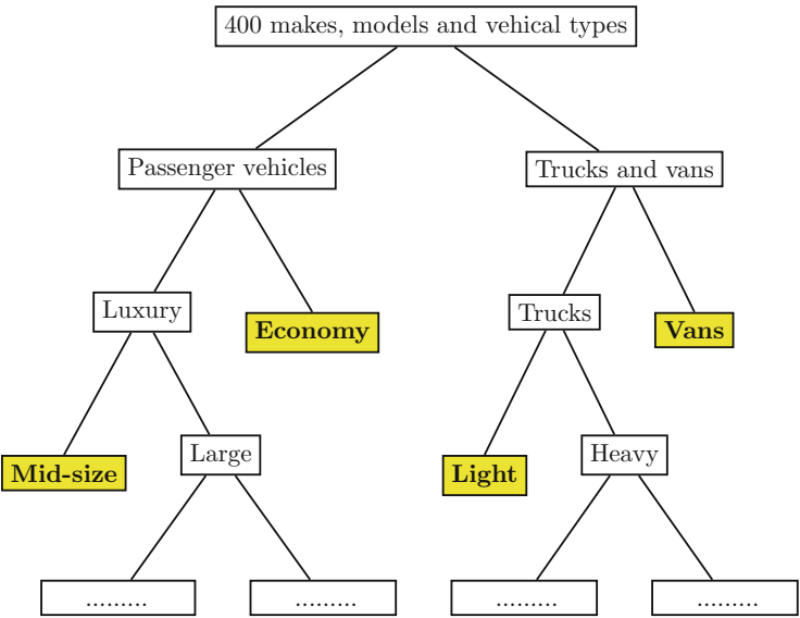
Fig. 20.25 Classification tree constructed by twoing index
