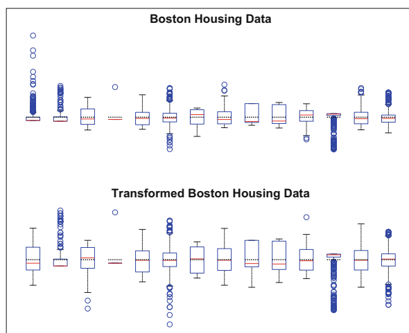
Fig. 1.37 Boxplots for all of the variables from the Boston housing data before and after the proposed transformations
