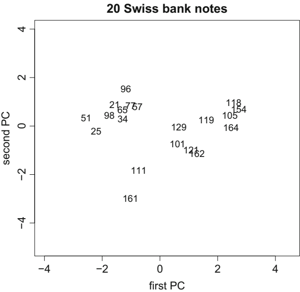
Fig. 13.4 PCA for 20 randomly chosen bank notes MVAcclusbank
