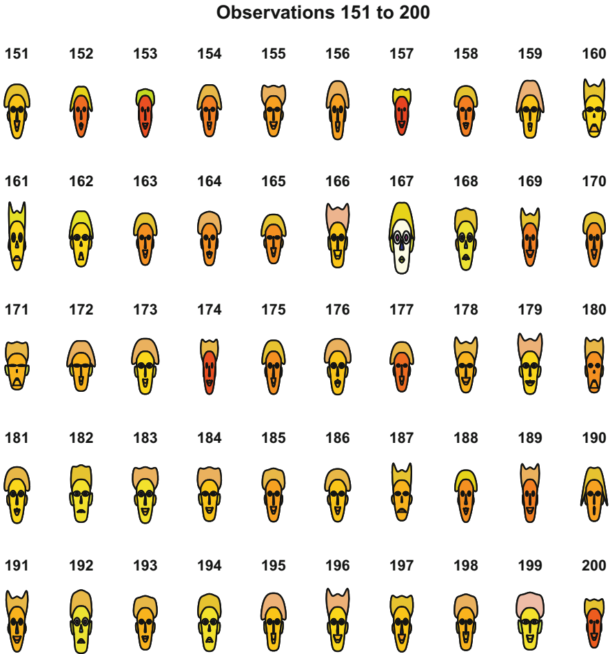
Fig. 1.19 Chernoff-Flury faces for observations 151–200 of the bank notes MVAfacebank50
