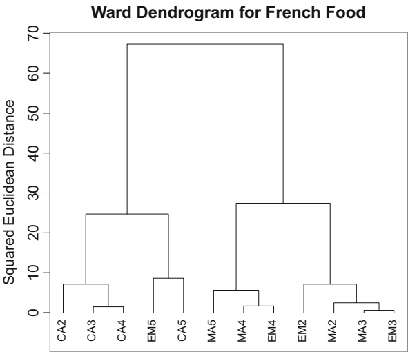
Fig. 13.6 The dendrogram for the French food expenditures, Ward algorithm MVAclusfood
