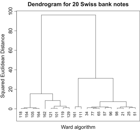
Fig. 13.5 The dendrogram for the 20 bank notes, Ward algorithm MVAcclusbank
