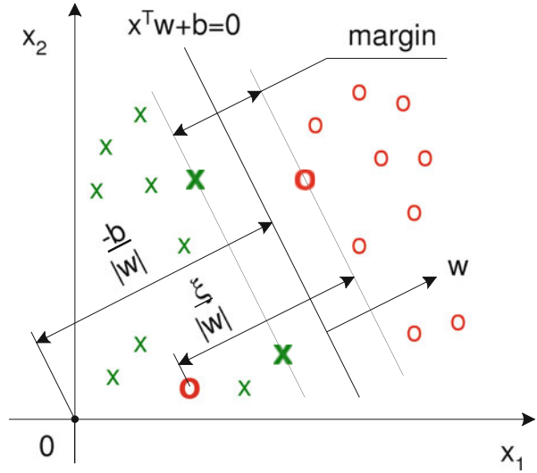
Fig. 20.13 The separating hyperplane x^\top w + b = 0 and the margin in the linearly non-separable case
