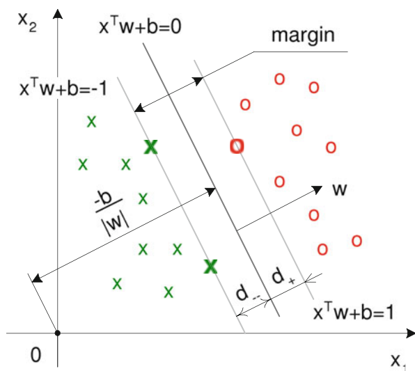
Fig. 20.12 The separating hyperplane x^\top w + b = 0 and the margin in the linearly separable case
