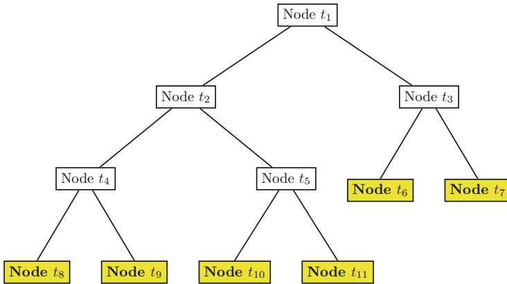
Fig. 20.26 Decision tree hierarchy
