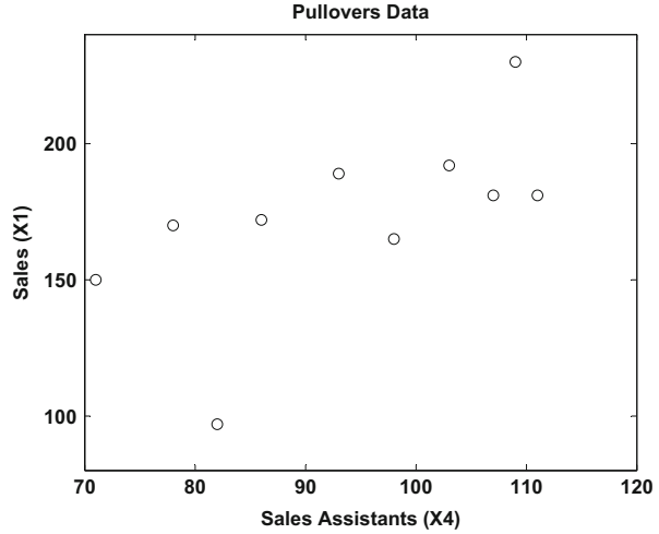
Fig. 3.4 Hours of sales assistants ( X_4 ) vs. sales ( X_1 ) of pullovers MVAscapull12
