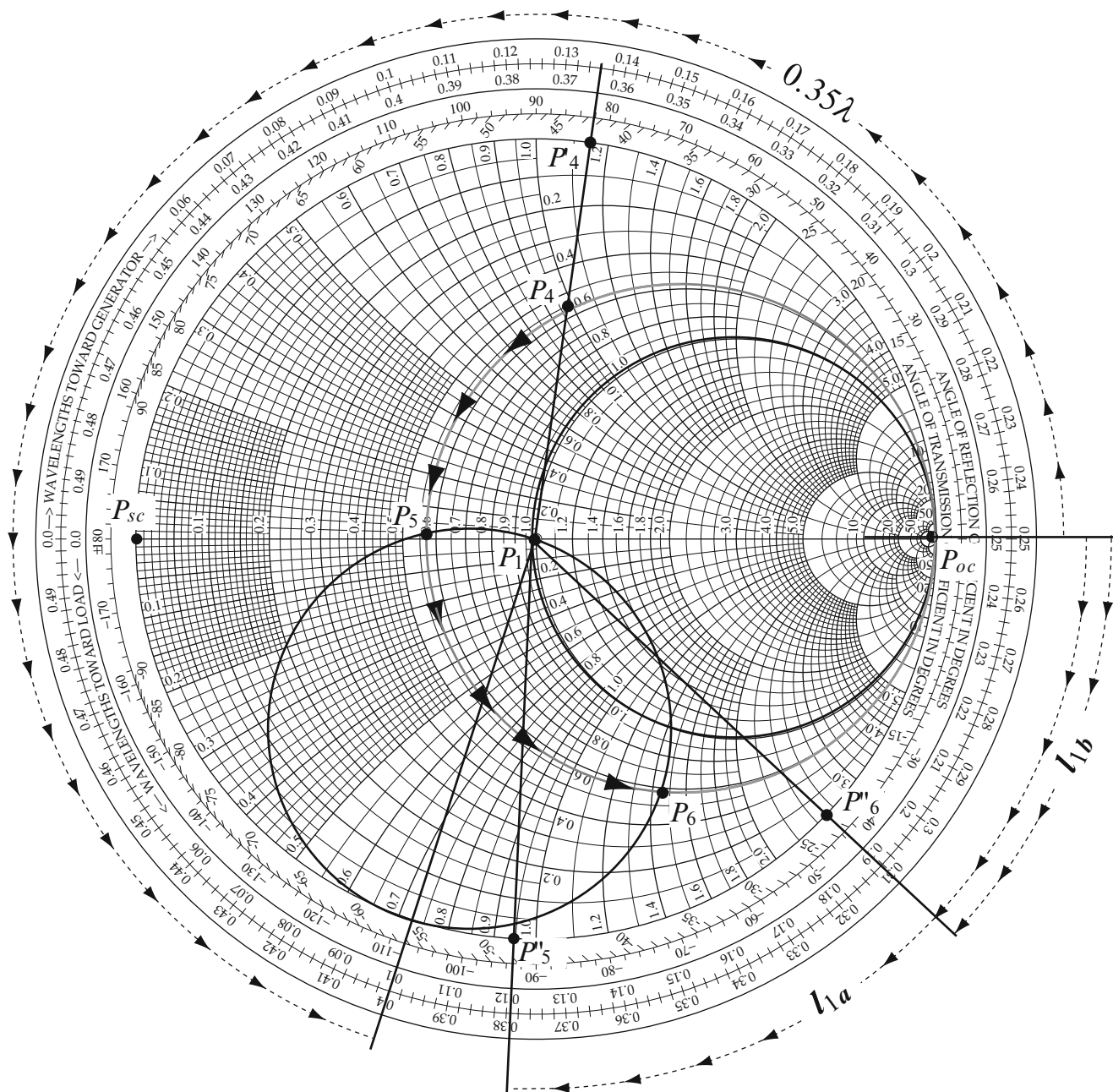
Figure 15.24 Smith chart for Example 15.6 (continuation)
