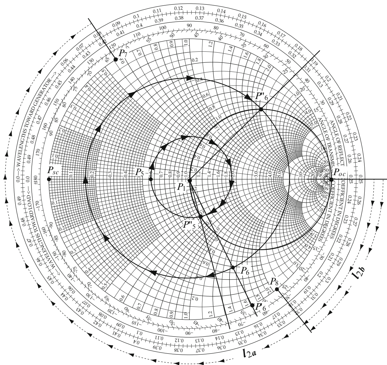
Figure 15.25 Smith chart for Example 15.6 (continuation)
