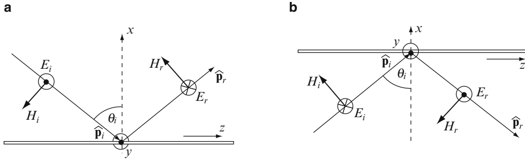
Figure 17.4 (a) Reflection of the incident wave off the lower plate in a parallel plate waveguide. (b) Reflection off the upper plate
