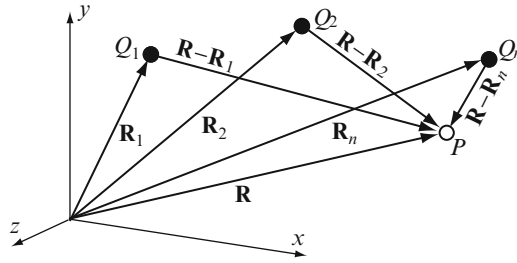
Figure 4.11 Calculation of potential at point P due to n point charges
