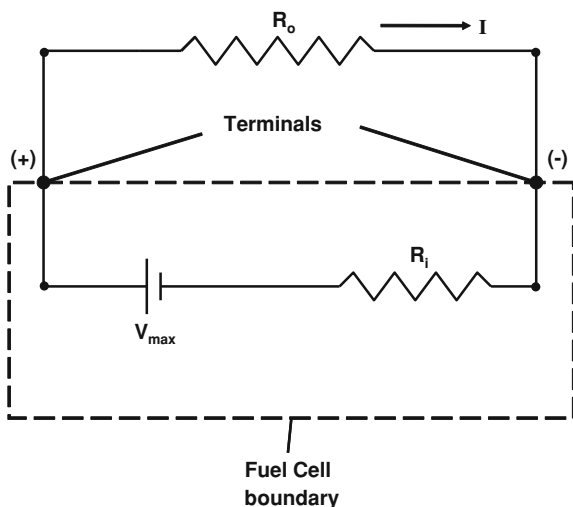
Fig. 12.11 The electric circuit diagram of a fuel cell
