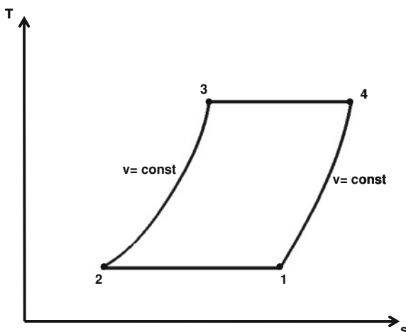
Fig. 7.6 The T-s diagram of the Stirling cycle
