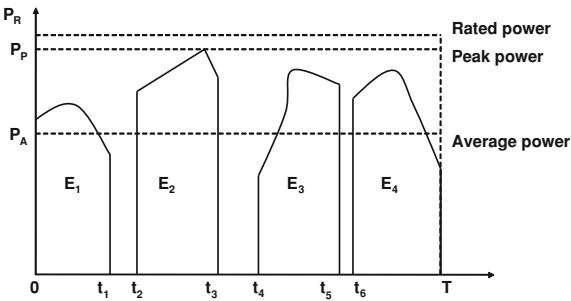
Fig. 12.3 Variable power parameters of a power plant
