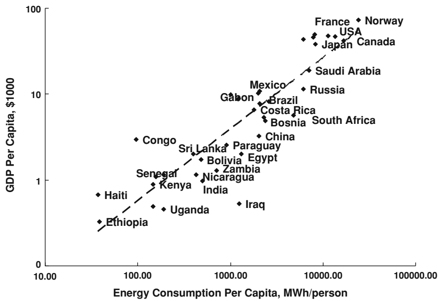
Fig. 1.1 Relationship between electric energy demand and GDP adjusted according to purchasing power. (Data from Key World Energy Statistics , IEA, 2009)
