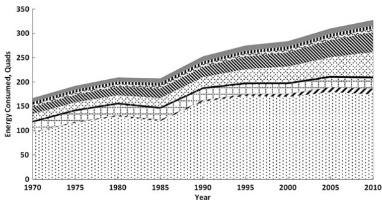
Fig. 1.5 The evolution of the global energy demand by region and groups of countries (data from Key World Energy Statistics , IEA, 2009). The areas (from bottom to top) represent OECD, Middle East, Former Soviet Union, non-OECD Europe, China, Rest of Asia, Latin America and Bunker fuel (the latter is used in transportation internationally)
