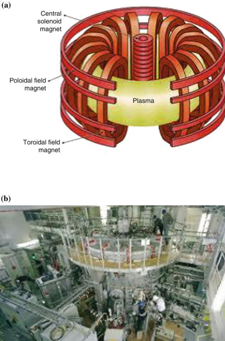
Fig. 6.6 a A schematic diagram of the Tokamak fusion reactor (courtesy of LLLNL) b A photograph of the MAST Tokamak reactor at Oxford, UK (courtesy of UKAEA)
