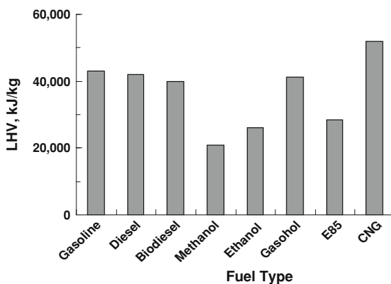
Fig. 10.3 LHV, in kJ/kg, of common fuels and biofuels
