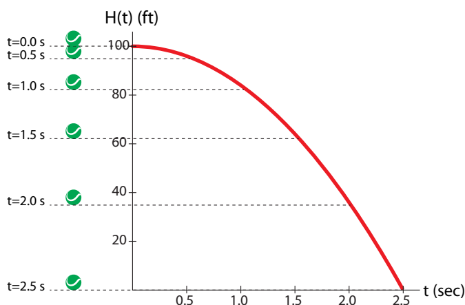
Figure 2.3: Graph of H(t) = 100 - 16t^2 , representing the height H of the ball, t seconds after being dropped from an initial height of 100 feet.
