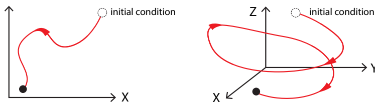
Figure 1.40: Trajectories in two- and three-dimensional state space.
