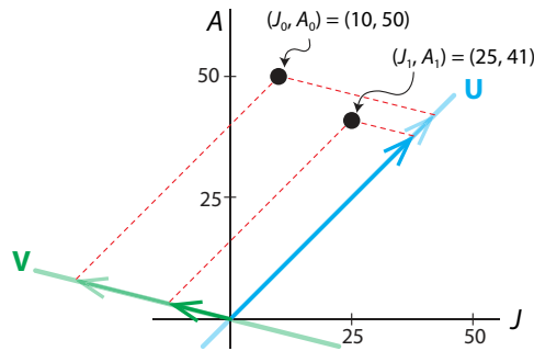
Figure 6.26: One application of the matrix \mathbf{M}_{bad} to the point (J_0, A_0) takes it to (J_1, A_1) which is closer to both the \mathbf{U} and \mathbf{V} axes.
