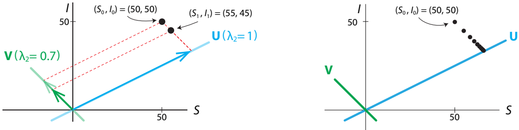
Figure 6.32: Left: Application of the S - I matrix M_{SI} to the initial condition (S_0, I_0) results in the state point (S_1, I_1) , closer to the U axis but at a constant distance from the V axis. Right: Repeated applications of M_{SI} approach the U axis while remaining a constant distance from V .
