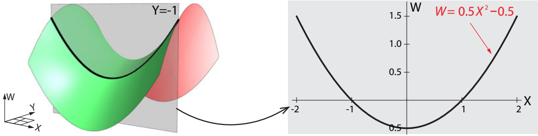
Figure 7.20: The XW cutting plane Y = -1 intersects the original surface, yielding the black curve.
