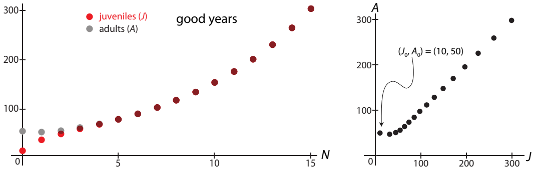
Figure 6.4: Time series (left) and corresponding trajectory (right) produced by iterating the matrix \mathbf{M} , modeling the black bear population in a good year. Notice that both consist of discrete points.
