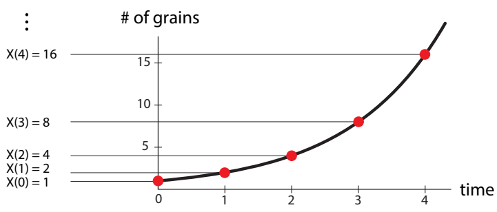
Figure 2.27: The red dots are calculations of X(t) = 2^t for t = 0, 1, 2, 3 and 4. The black curve is the continuous function X(t) = 2^t , which exhibits exponential growth.
