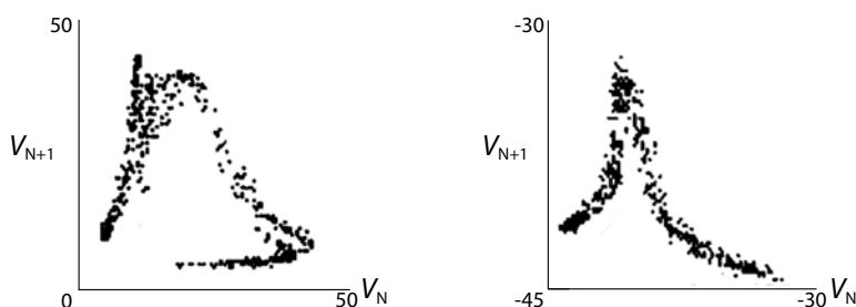
Figure 5.48: Poincaré plots of stroboscopic data from a neuron experiment. Here V is in millivolts. Reprinted from Physics Letters A 88(8), Hatsuo Hayashi, Satoru Ishizuka, Masahiro Ohta, and Kazuyoshi Hirakawa, “Chaotic behavior in the Onchidium giant neuron under sinusoidal stimulation,” pp. 435–438, Copyright 1982, with permission from Elsevier.
