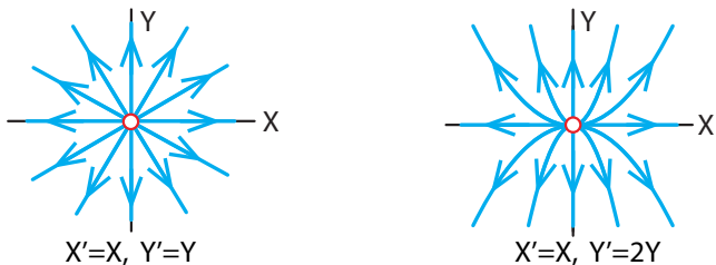
Figure 3.16: Unstable nodes.
