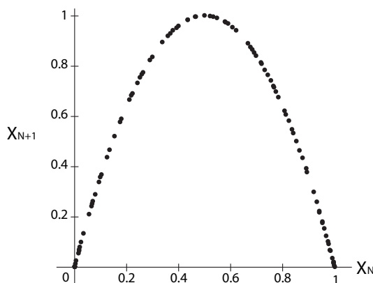
Figure 5.34: Poincaré plot of data from the previous figure.
