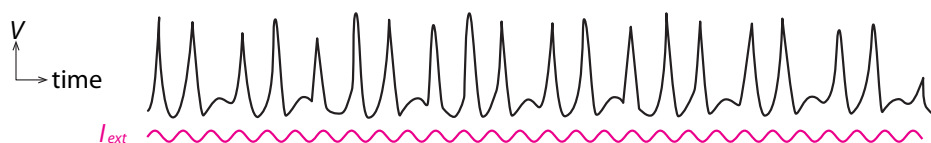
Figure 5.47: Chaotic response of a neuron to sinusoidal stimulation. Redrawn from Physics Letters A 111(5), K. Aihara, G. Matsumoto, and M. Ichikawa, 1985, “An alternating periodic-chaotic sequence observed in neural oscillators,” pp. 251–255, Copyright 1985, with permission from Elsevier.
