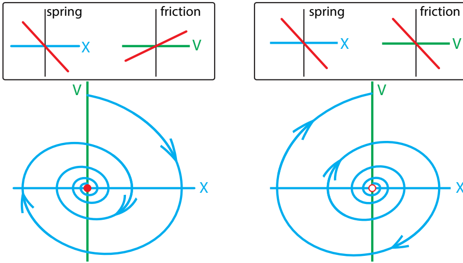
Figure 4.6: Left: When the friction force is positive, the system has a point attractor of spiral type at (0, 0) . Right: When the friction is negative, the origin becomes a spiral type unstable equilibrium.
