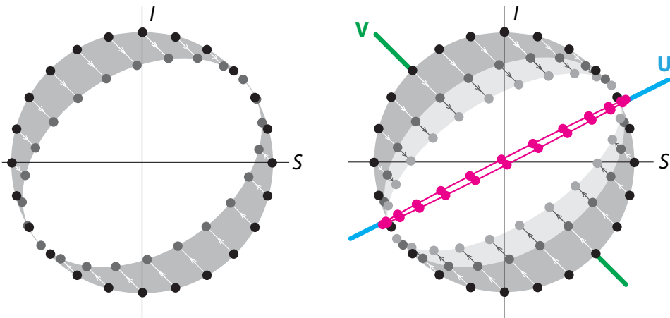
Figure 6.35: Left: one application of the S - I matrix to a circle of initial conditions (dark gray) transforms them into a oval. Right: repeated applications flatten and rotate the oval. By the tenth iteration (red dots), the initial circle has been transformed into a line lying along the principal eigenvector.
