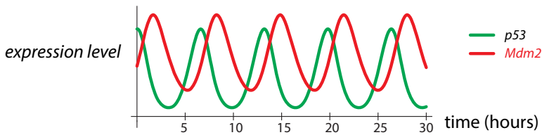
Figure 4.26: Simulation of Model VI of (Lahav et al. 2004). Green (lower) tracing is p53, red (upper) is Mdm2. Parameter values are \beta_X = 0.9 , \alpha_{XY} = 1.4 , \beta_Y = 1.2 , \alpha_Y = 0.8 , \beta_S = 0.9 , \alpha_S = 2.7 , \tau = 0.9 , X_0 = 0 , Y_0 = 0.9 , S_0 = 0 .
