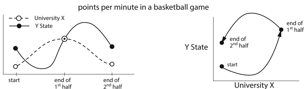
Figure 1.46: Time series and state space of a hypothetical basketball game.
