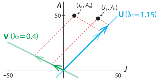
Figure 6.23: One application of the matrix \mathbf{M} to the point (J_0, A_0) takes it to (J_1, A_1) which is closer to the dominant eigenvector \mathbf{U} axis and further from the \mathbf{V} axis.
