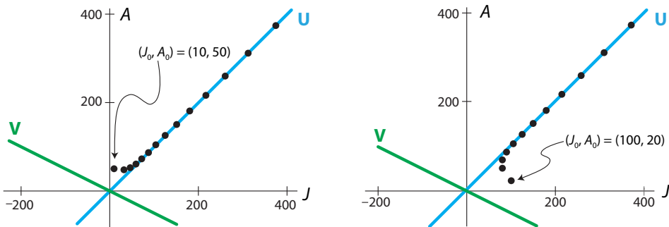
Figure 6.24: After repeated iterations of the matrix \mathbf{M} , the long-term trajectory lies along the direction of the dominant eigenvector \mathbf{U} axis, regardless of the initial conditions. Eventually, the ratio of adults to juveniles approaches a constant value.
