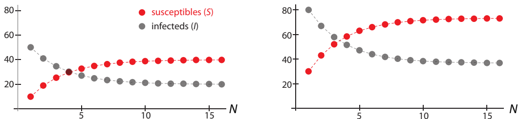
Figure 6.7: Time series from two simulations of the susceptible-infected model. Starting from different initial conditions, the system converges to different equilibrium points.
