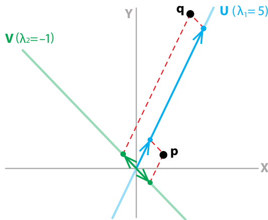
Figure 6.13: Using eigenvalues and corresponding eigenvectors to find the action of \mathbf{M} on the point \mathbf{p} in the \{\mathbf{U}, \mathbf{V}\} coordinate system.
