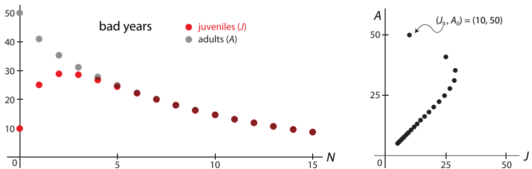
Figure 6.5: Time series (left) and corresponding trajectory (right) produced by iterating the matrix \mathbf{M}_{bad} , modeling the black bear population in a bad year.
