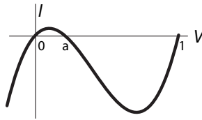
Figure 4.40: Shifted “N”-shaped resistor characteristic function f(V) . Here a = 0.1 .
