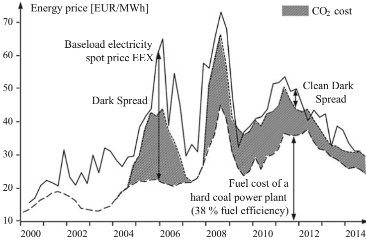
Fig. 10.7 German (clean) dark spread between 2001 and 2014
