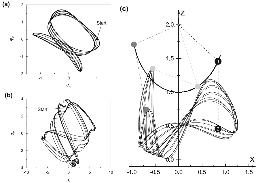
Fig. 6.3 Numerical solution of the double pendulum with initial conditions \varphi_1(0) = 1.0 , \varphi_2(0) = 0.0 , p_1(0) = 0.0 and p_2(0) = 3.0 . (a) Trajectory in \varphi -space, (b) trajectory in p -space, and (c) trajectory in local (x, z) -space. The solid circles numbered 1 and 2 represent the two masses in their initial configuration
