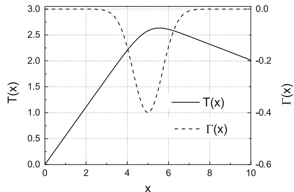
Fig. 9.4 Temperature profile T(x) (solid line, left hand scale) and the source function \Gamma(x) (dashed line, right hand scale) for N = 100
