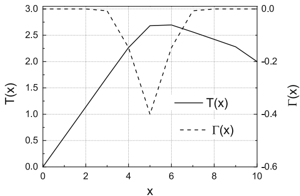
Fig. 9.3 Temperature profile T(x) (solid line, left hand scale) and the source function \Gamma(x) (dashed line, right hand scale) for N = 10
