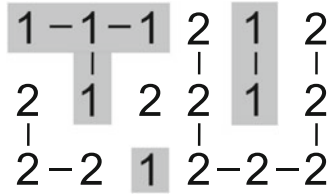
Fig. 18.8 Schematic illustration of the identification of clusters according to the SWENDSEN-WANG algorithm. 1 and 2 denote two different spin orientations, bonds are denoted by solid lines and all bonded spins form clusters
