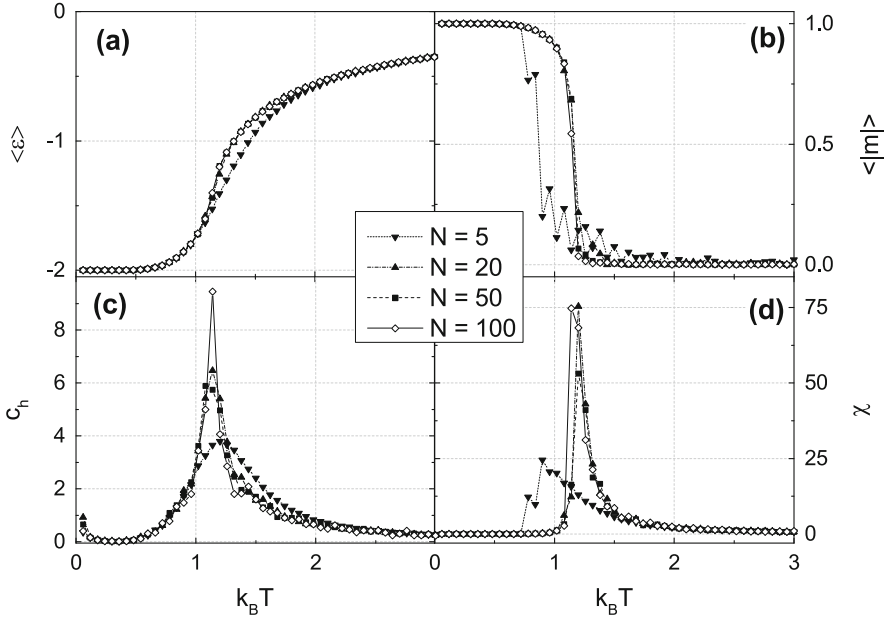
Fig. 15.5 (a) The expectation value of the energy per particle ( \varepsilon ), (b) the absolute value of the expectation value of the magnetization per particle |\langle m \rangle| , (c) the heat capacity c_h , and (d) the magnetic susceptibility \chi vs temperature k_B T for the two-dimensional ISING model. The system sizes are N = 5, 20, 50, 100
