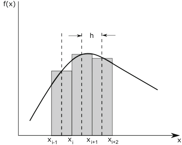
Fig. 3.2 Scheme of the rectangular integration rule according to Eq. (3.14). Note that boundary points do not enter the evaluation of the elemental areas
