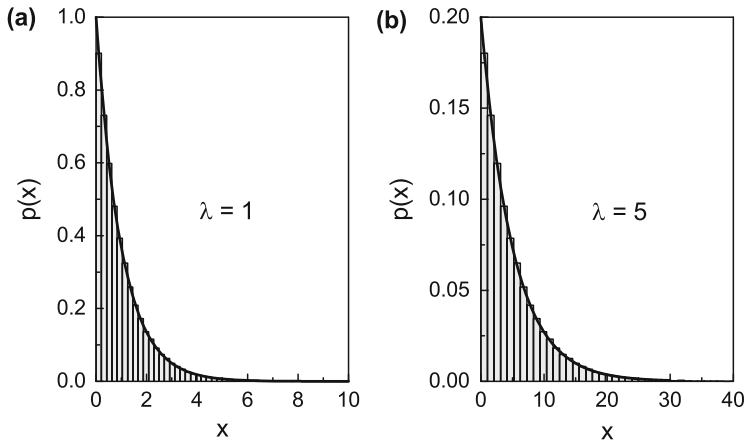
Fig. 13.1 The histogram representation of the pdf p(x) vs x generated by random numbers drawn from an exponential distribution Eq. (13.22) with the help of the inverse transformation sampling method. Two different values for \lambda have been considered, namely (a) \lambda = 1 and (b) \lambda = 5 . N = 10^5 random numbers have been sampled. The solid line corresponds to the pdf p(x) according to Eq. (13.22)
