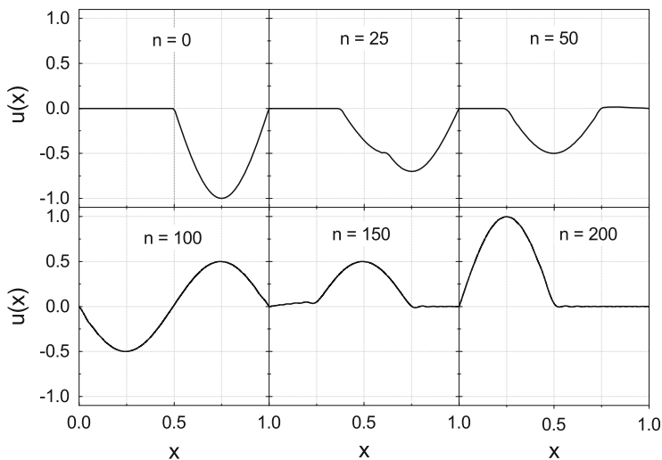
Fig. 11.6 Solutions of the wave equation u(x) vs x generated by the explicit EULER method with \lambda = 0.5 . Results after n = 25, 50, 100, 150, and 200 time steps are presented. n = 0 represents the initial conditions
