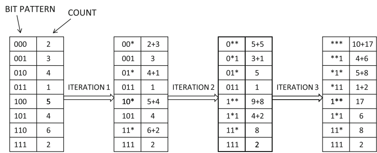
Figure 4.6: Performing the second phase of bucketing
