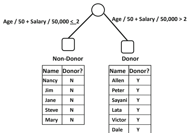
(b) Multivariate split
