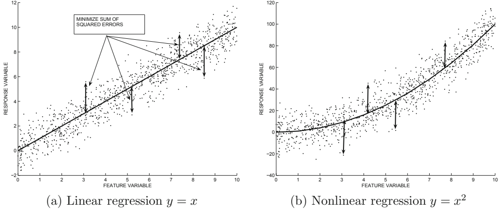
Figure 11.1: Examples of linear and nonlinear regression
