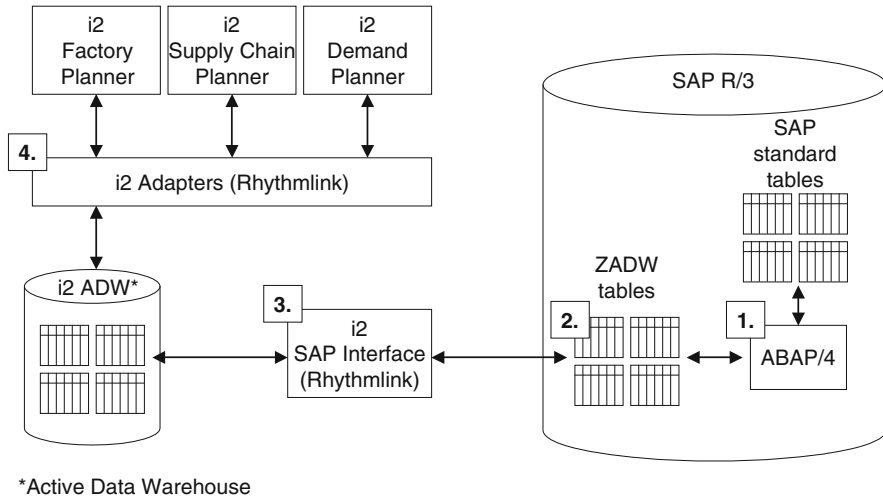
Fig. 23.7 Integration of the i2 planning modules with SAP R/3
