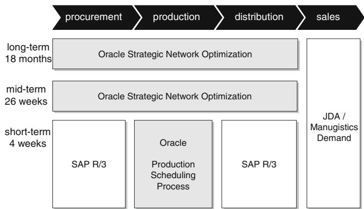
Fig. 21.3 The architecture of the planning system
