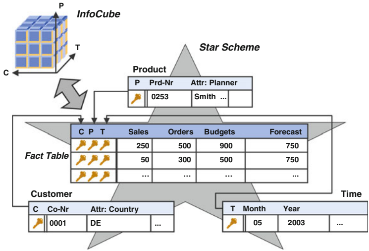
Fig. 20.4 InfoCube and star scheme
